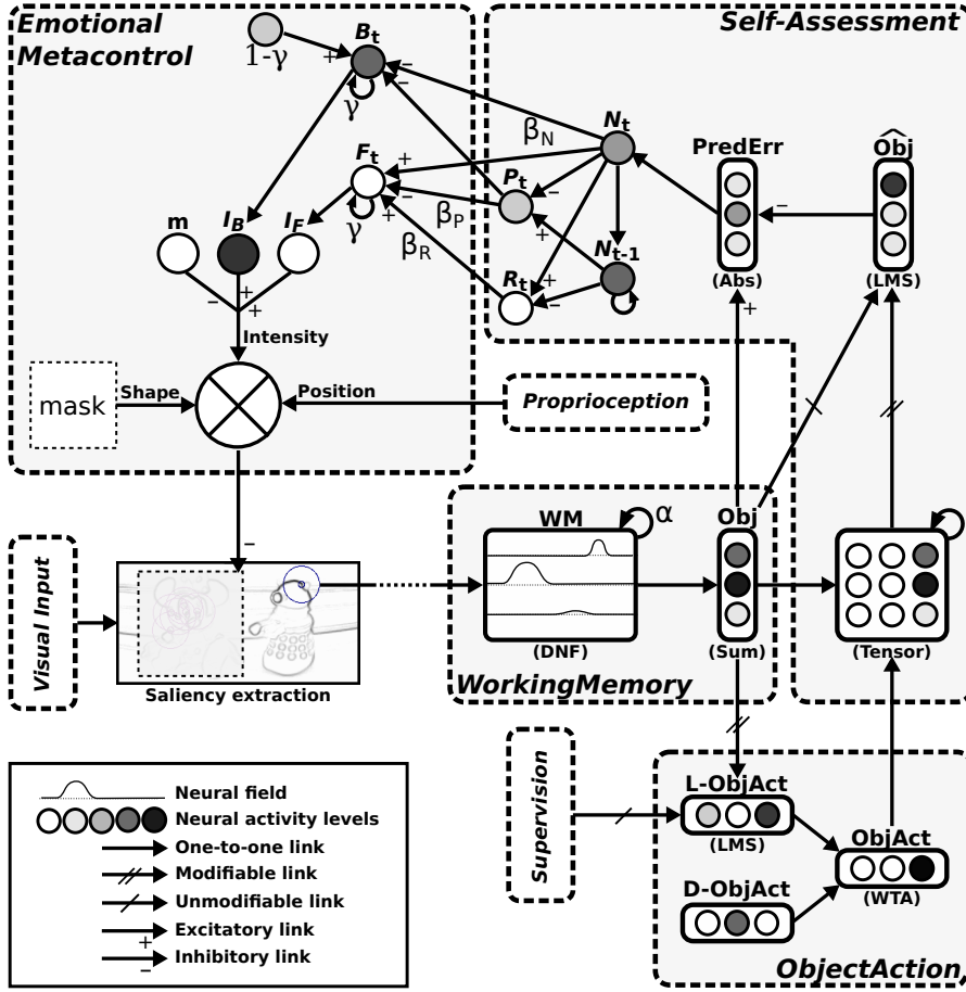
Figure 7.7: Self-Assessment and Emotional Metacontrol modules. LMS: Least Mean Square; DNF: Dynamic Neural Field; WTA: Winner-Takes-All; Abs: Absolute Value. WM: Working Memory. D-ObjAct: Default ObjectAction. L-ObjAct: Learned ObjectAction. N_t , P_t , R_t , F_t and B_t correspond to the novelty \mathcal{N} , progress \mathcal{P} , regress \mathcal{R} , frustration \mathcal{F} and boredom \mathcal{B} at time t in the equations. Some of the parameters of those equations like \alpha and \gamma are also shown on this figure.
