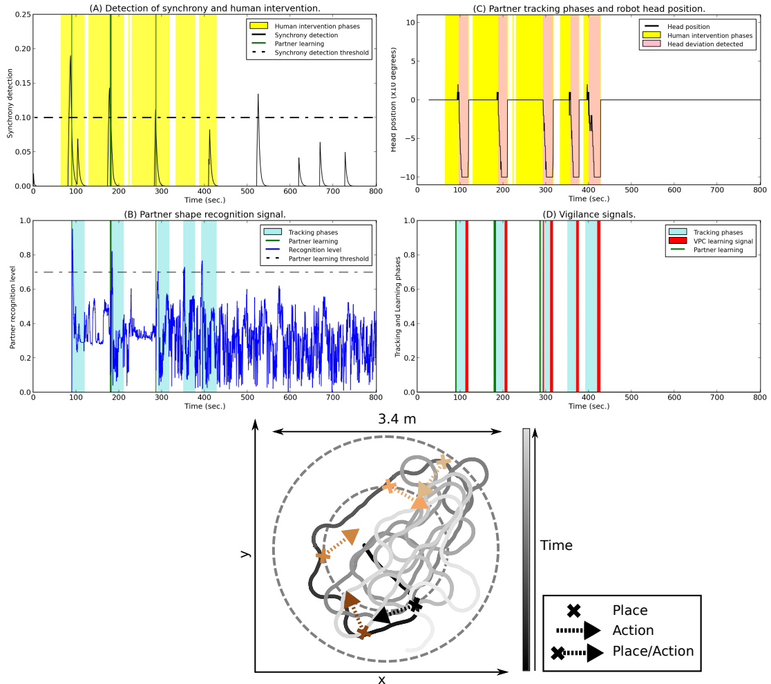
Figure 3.5: Results of the experiment on interactive learning of place-action navigation. TOP: Neural activities. The same signals have the same color in (A), (B), (C), and (D). (A) During human intervention, synchrony detection activities higher than threshold phases trigger partner learning. (B) When the partner is recognized the tracking phase is launched. (C) When the robot head orientation changes a deviation is detected. (D) Tracking phase induces a change of orientation which triggers place/action learning. BOTTOM: Robot trajectory and spots where place/action learning occurred. The gray gradient illustrates the time course. The robot learned to stay inside the 170 cm radius tolerated zone.
