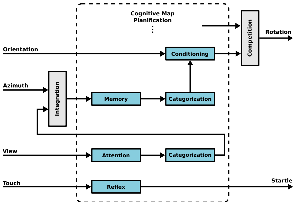
Figure 5.7: Instantiation of the abstract model of sensorimotor architectures. Two behaviors are represented: raw stimulus-driven startle reflex and place/action navigation strategy. The parallel computational processes included in this example are reflex, attention, memory, categorization and place–action learning (conditioning). Integration here refers to the combination of what–where information: visual landmarks and their azimuths.
