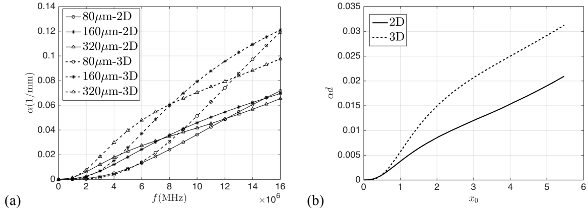
Fig. 2.5. Analytical results of the longitudinal wave attenuation coefficient for a polycrystalline titanium with different grain sizes in the 3D and 2D cases (a) \alpha vs. f ; (b) master curves \alpha d vs. x_0 .
