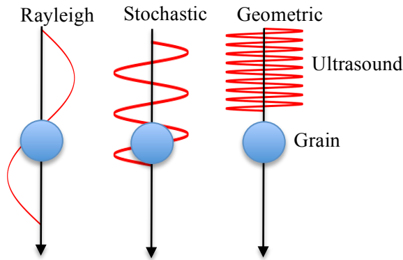
Fig. 1.3. Schematic of three scattering frequency regions
