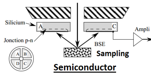
Figure 4.3: Backscattered electrons sensors [1].
