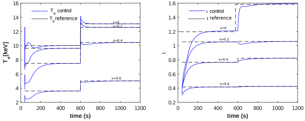
Figure 3.11: Evolution of T_e and l in the ITER simulation (control case 2).
