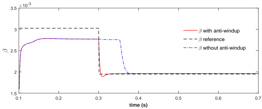
Figure 4.3: Comparison of the performance of the control of \beta without (blue dash line) and with (red line) the application of an anti-windup scheme.
