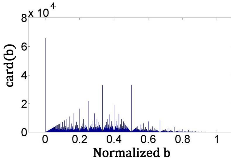
Figure 20: Non-uniform occurrence frequency of unique b values, calculated for all possible b values of the RGB space.
