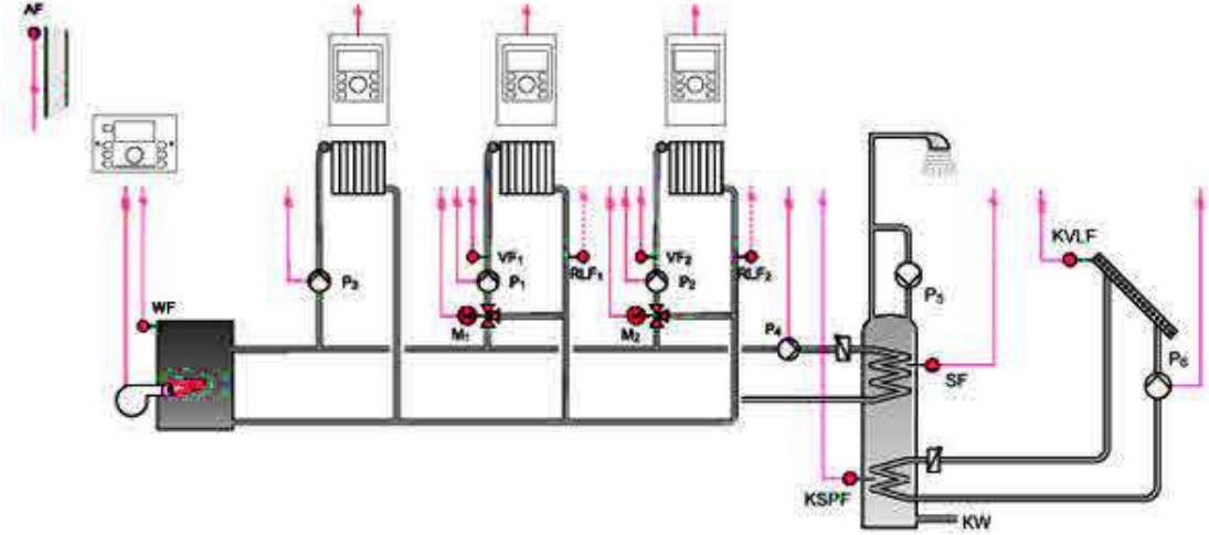
Figure 5.5: Separated heating and domestic hot water system
