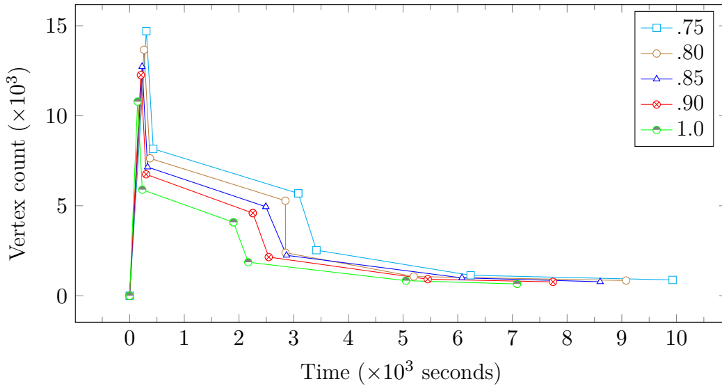
Figure 3.5: Evolution of mesh complexity over time for different \delta(\%) . Each mark depicts the completion of: refinement; simplification via halfedge collapses of \partial\Gamma ; edge collapses of \partial\Gamma ; mutual tessellation and halfedge collapses of \mathcal{Z} ; edge collapses of \mathcal{Z} ; and simplification of all edges. The input is a raw surface mesh of the fertility model (14kv).
