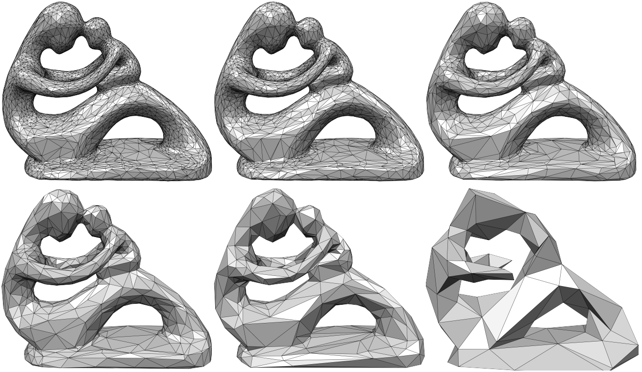
Figure 3.2: Fertility. From top left to bottom right: \delta is set to 0.15, 0.25, 0.4, 0.8, 2.0 and 8.0. The final vertex count is 4,642, 2,768, 1,484, 767, 417 and 120, respectively. The input model is a surface triangle mesh of the fertility model with 14k vertices.
