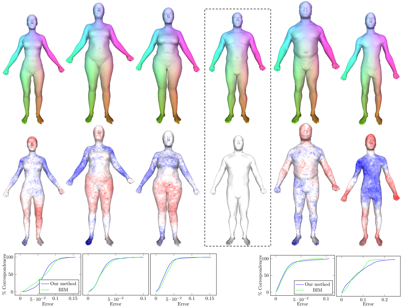
Figure 7.11: Mapping between human bodies. The reference model is outlined. We depict the mappings (xyz coloring) and the relaxed area. The curves depict the quality of the correspondences and offer a comparison to BIM.
