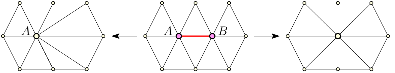
Figure 1.5: Edge collapse. Given an edge AB (middle), a half-edge collapse (left) locates the target vertex at one of the vertices of the edge. A general edge collapse (right), relocates the target vertex based on the user defined criteria. Note that an edge collapse always has a unique triangulation (combinatorially, depending on its one-ring neighbours), although the final vertex location may change.
