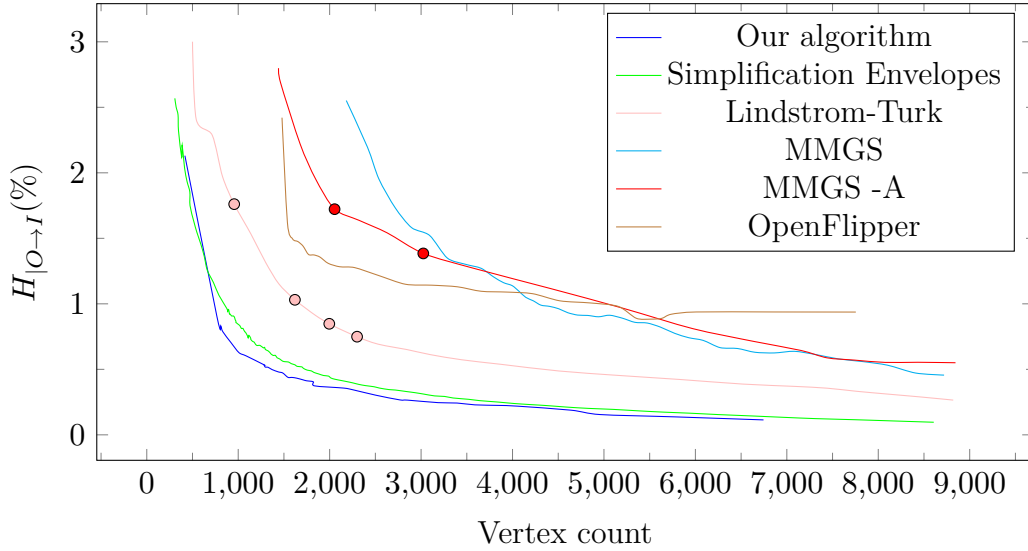
Figure 3.6: Comparisons. We plot the one-sided Hausdorff distance (output to input) ( H_{|O \rightarrow I} ) against the final number of vertices. A dot indicates a self-intersection of the output mesh. The input mesh is a clean surface triangle mesh of the fertility model (14kv).
