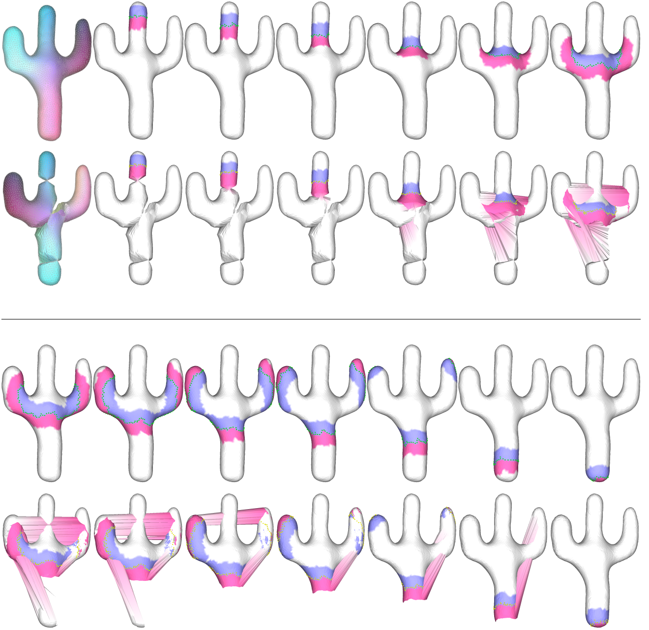
Figure 6.8: Fixing flips and twists. Starting from a suboptimal map having discontinuity (left, cactus (top) to itself (bottom) built by intentionally placing bad constraints), ironing proceeds through front propagation to remove all artifacts. For each strip, blue indicates the visited parts while the non visited parts are in pink. In case of multiple fronts, each front is considered independently. Note that the main idea behind whole approach is to slightly distort the neighborhood and favor already visited parts. Using high value for \omega (close to 1) cannot unfold the mapping, while low values (close to 0) seriously pull \eta 's towards already-visited parts.
