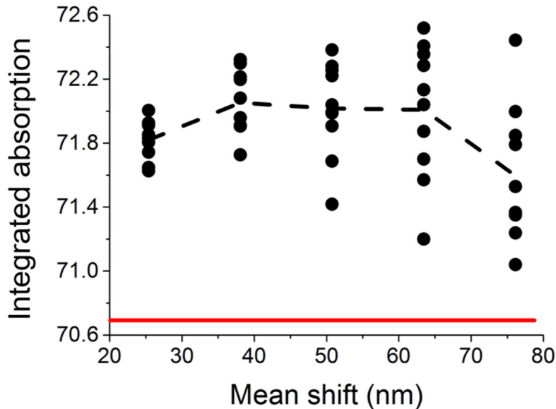
Figure 5-4. Evolution of the theoretical integrated absorption for 10*5 pseudo-disordered structures (dark dot). The mean value of integrated absorption (black dashed line) remains higher than the optimized square lattice of holes structure as the reference value (red horizontal line).
