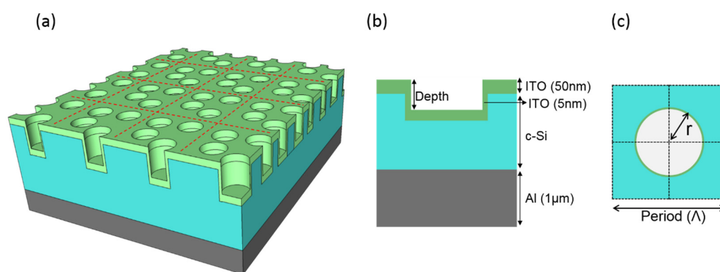
Figure 6-1. (a) Schematic view of the thin film solar cells stack with pseudo-disordered structure. (b) side-view and (c) top view of the thin film solar cell.
