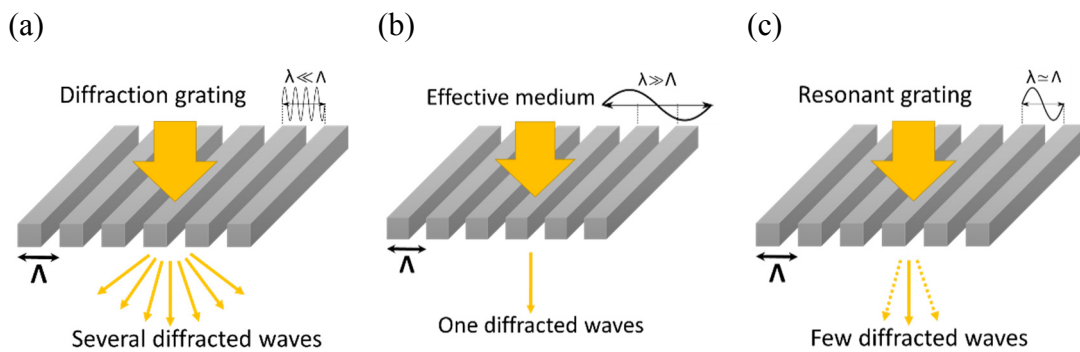
Figure 2-8. 1D grating structures designed for trapping of light. The different period of the grating ( \Lambda ) function with a normal incidence: diffraction grating (a), effective medium slab (b), and resonant (sub-wavelength) grating (c).
