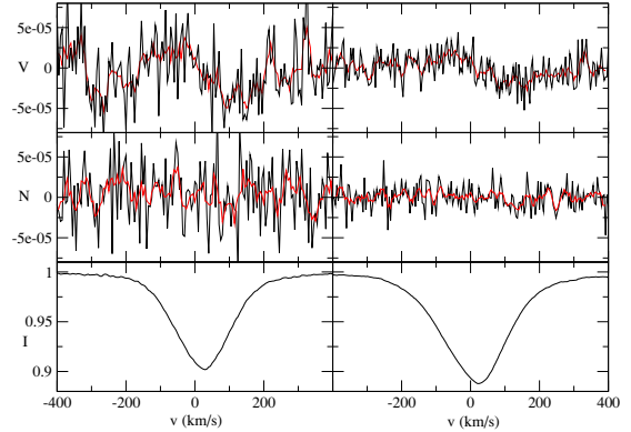
Fig. 2. LSD Stokes I (bottom), Stokes V (top), and null N (middle) profiles, normalized to I_c , for the night of 25 October 2008 for the mask of Bouret et al. (2008) (left) and for our own mask (right). The red line is a smoothed profile.
