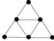
Figure 1: A self-centered graph G with diam(G) = rad(G) = 2 , while \delta(G) = 1/2 = diam(G)/4 .
