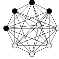
(b) \delta(BK(G_{3,3})) = 0
