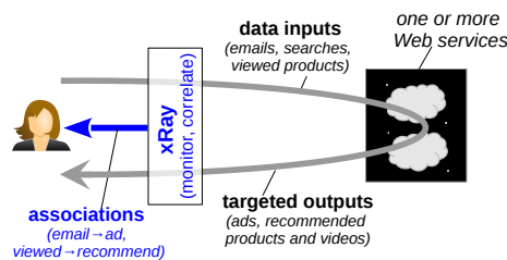
Figure 1: XRay Conceptual View. XRay views Web services as black boxes, monitors user inputs and outputs to/from them, and detects data use through correlation. It returns to the user or auditor associations of specific inputs and outputs.
