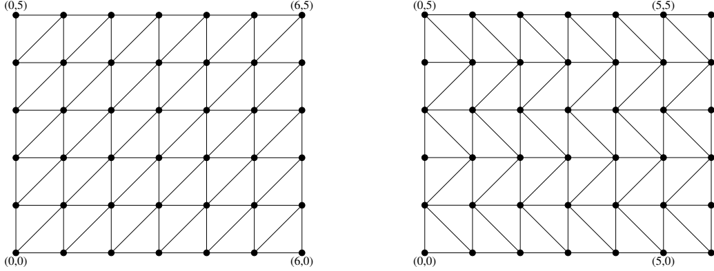
(a) The triangular (7,6) -grid has hyperbolicity \delta = \frac{5}{2} = \delta(u, v, x, y) with u = (6, 0) , v = (0, 5) , x = (0, 0) , y = (6, 5) . (b) The hexagonal (7,6) -grid has hyperbolicity \delta = \frac{5}{2} = \delta(u, v, x, y) with u = (0, 5) , v = (5, 0) , x = (0, 0) , y = (5, 5) .
