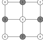
Figure 2: The bipartite graph G_{3,3} with each side of the bipartition colored differently.
