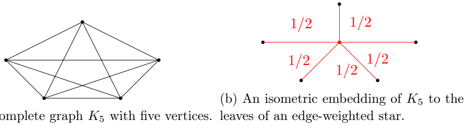
Figure 2.7: Complete graphs are 0-hyperbolic.
