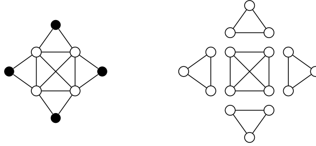
Figure 2.22: Clique-decomposition of a graph in five atoms. A 4-tuple with hyperbolicity 1 is drawn in bold.
