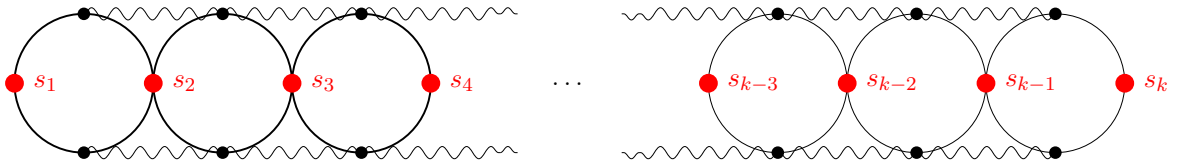
Figure 3.13: A minimal k -separator S for G \in \mathcal{G}_\ell with diameter \lfloor \ell/2 \rfloor \cdot (k - 1) . Vertices in S are ordered so that any two consecutive vertices s_i and s_{i+1} are diametrically opposed in an isometric cycle of length \ell . Furthermore, the removal of S disconnects G in two parts, respectively containing the upper and lower sections of these cycles.
