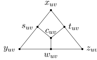
Figure 3.7: Gadget graph F_{uv} . The two vertices x_{uv}, w_{uv} are on disjoint s_{uv}t_{uv} -paths. Since they have no common neighbour, it ensures that s_{uv}, t_{uv} must be contained in a same bag in any star-decomposition of F_{uv} .
