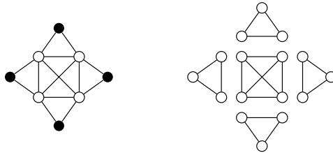
Figure 1: Clique-decomposition of a graph in five atoms. A 4-tuple with hyperbolicity 1 is drawn in bold.
