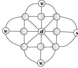
Figure 25: A planar graph G with tb(G) = 1 and all of its four leaf-vertices v_1, v_2, v_3, v_4 of Type 2.
