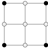
(a) \delta(G_{3,3}) = 2
