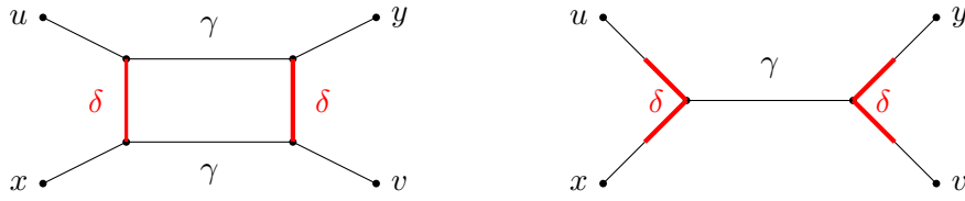
(a) Canonical realization of the 4-tuple. Distances in the realization are exactly the distances in the graph. (b) Non contractive tree embedding with distortion \delta that is obtained from the realization.
