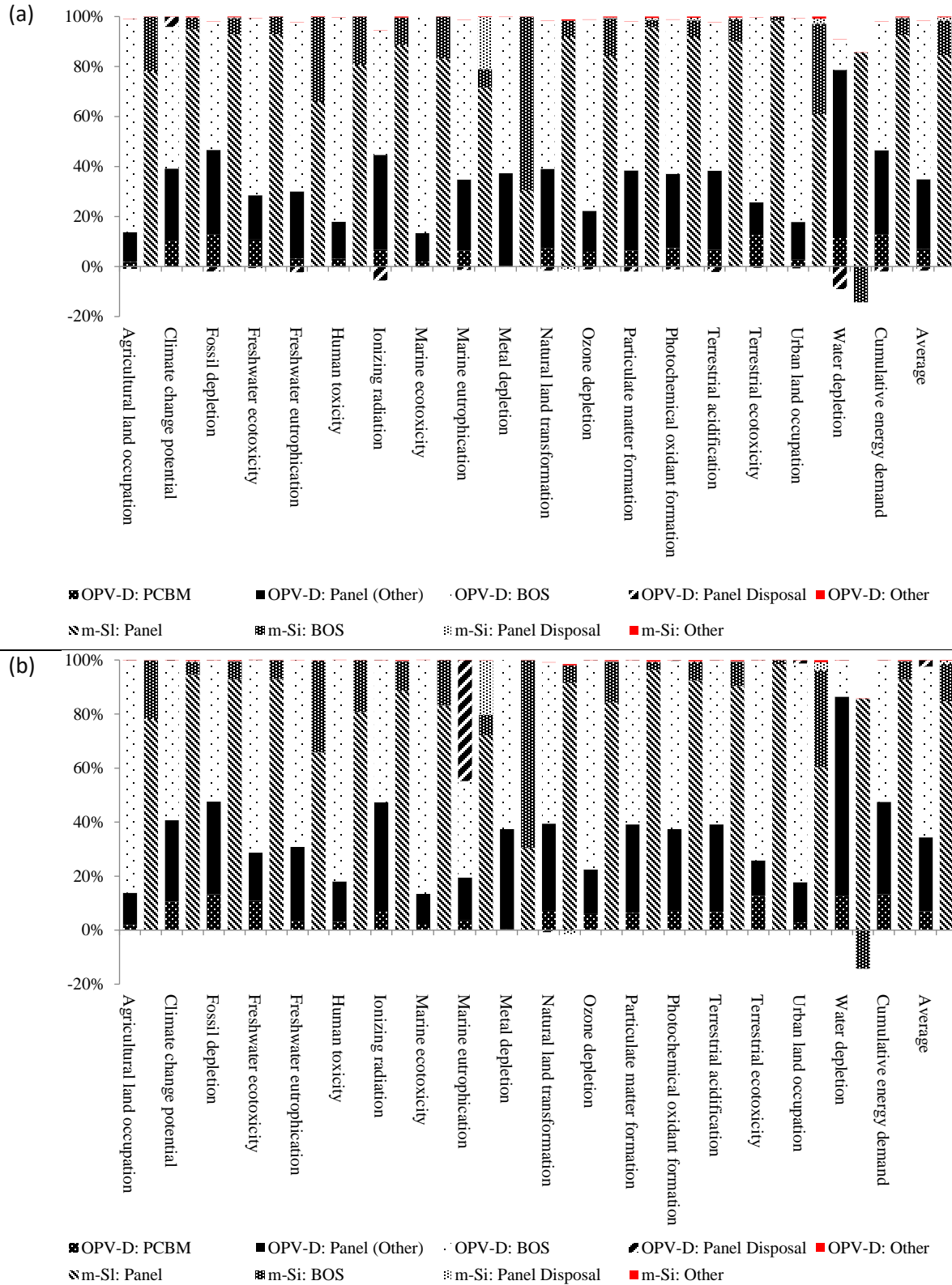
Figure A4-1 Contributions from each life-cycle stage for the OPV-D and m-Si panels when panels were (a) incinerated and (b) landfilled at their end-of-life for S1 (rooftop array).
