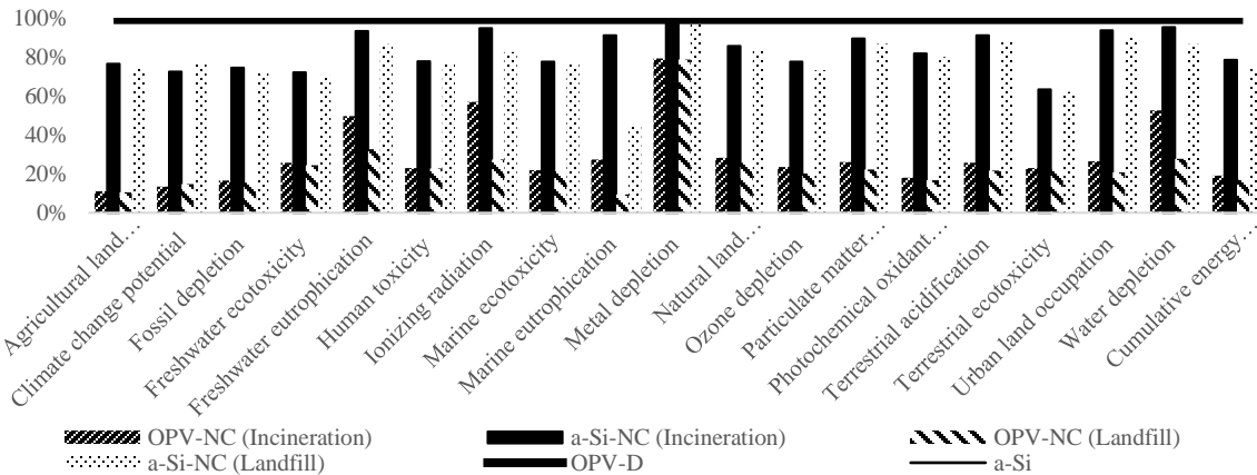
Figure A4-12 Comparison of S2 alternatives based on portable chargers without casing. The impact results in S2 are individually normalized by technology-type (i.e. OPV-NC is normalized by OPV-D and a-Si-NC is normalized by a-Si). NS: no casing materials.
