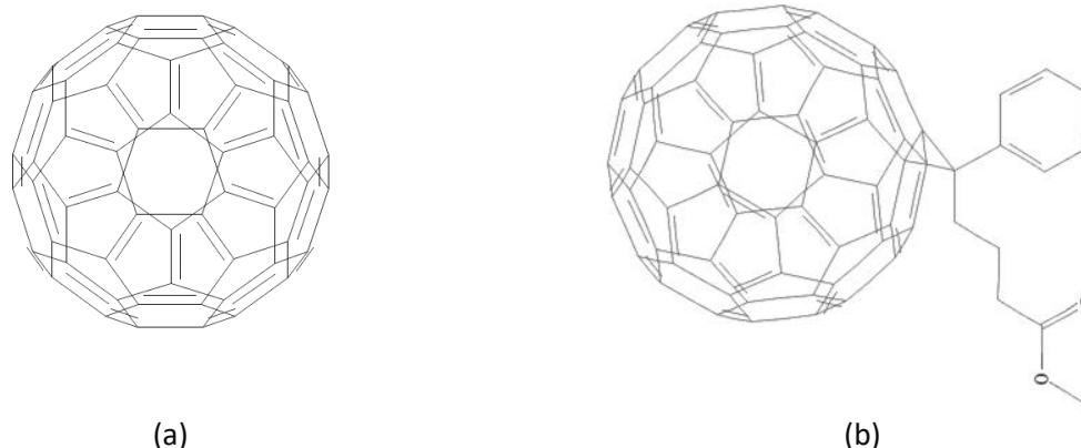
Figure 1-7 Two-dimensional structures of (a) an unmodified fullerene with 60 carbon atoms and (b) a functionalized 60-carbon ring fullerene (PCBM). (Source: PubChem Open Chemistry Online Database)
