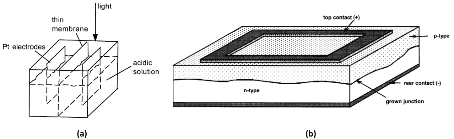
Figure 1-1 Illustrations of (a) the setup described by Becquerel in 1839 to achieve the first known, intentionally produced photovoltaic effect and (b) the oldest contemporary interpretation of the p-n silicon semiconducting cell as it is known today. (Source: Greet 2002) 12
