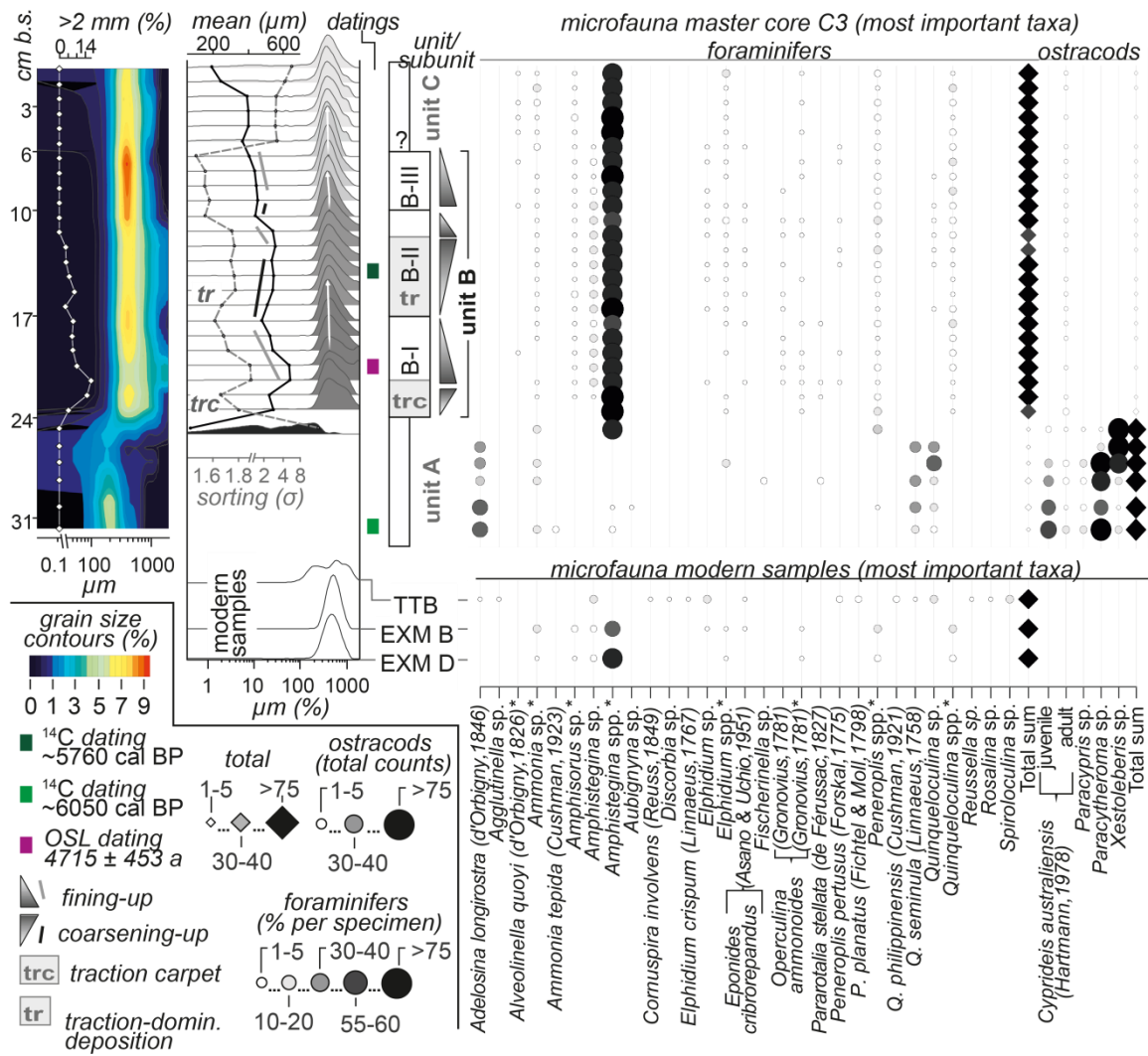
Fig. 2. Sediment characteristics, granulometry and microfossil data of master core C3 and the modern samples. * – reworked (fragmented/rounded); b.s. – below surface.
