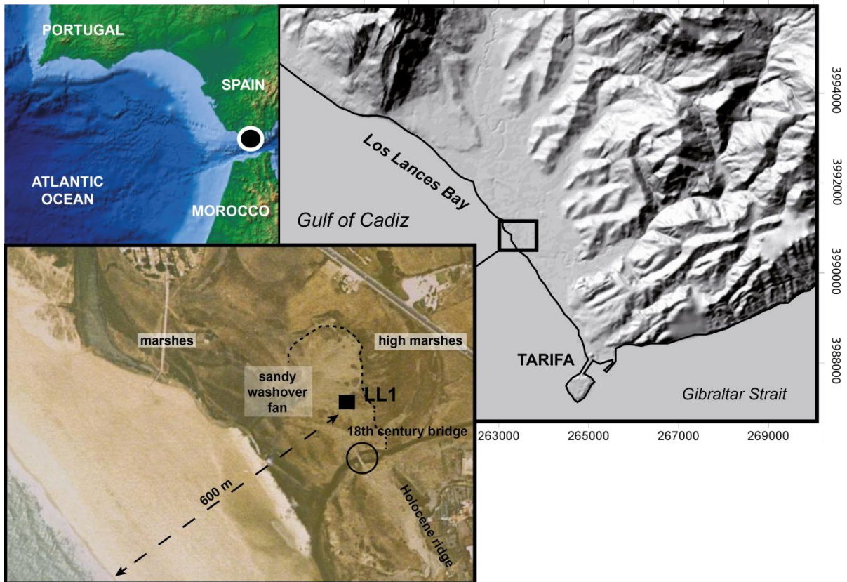
Fig. 1: Location map and satellite view of the study area. The tsunami samples were retrieved from the 1755 sandy washover fan in Los Lances Bay. The bridge was partially destroyed by the tsunami (after Cuven et al., 2013).
