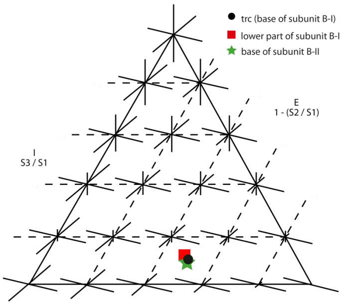
Fig. 5. Shape of the ellipsoids calculated from the orientations (longest axis) of the particles separated for each subsample using the shape triangle diagram of Benn (1994). Particle isotropy (I) and elongation (E) are calculated using the eigenvectors of the ellipsoids, S1 (max eigenvalue), S2 (intermediate) and S3 (min); see Benn (1994) for details. The eigenvalues have been calculated using Stereo32 software. All subsamples exhibit a rather prolate shape, which supports the idea of a traction-based transportation mode of the particles.
