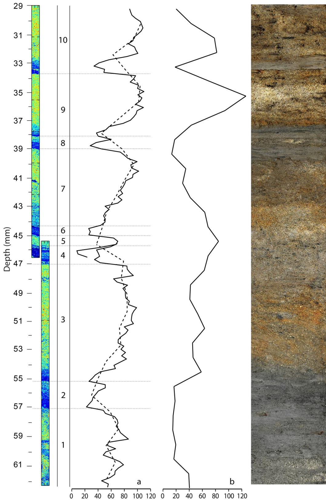
Fig. 11: Comparison of mean grain size data obtained with X- CT (a) using a 10mm step (dashed line) and a 2mm step (full line) and laser diffraction (b, 10mm step). X- CT allows using very fine measurement steps (depending only on the resolution of the scans) and precisely linking structures and subunits to GSD data.
