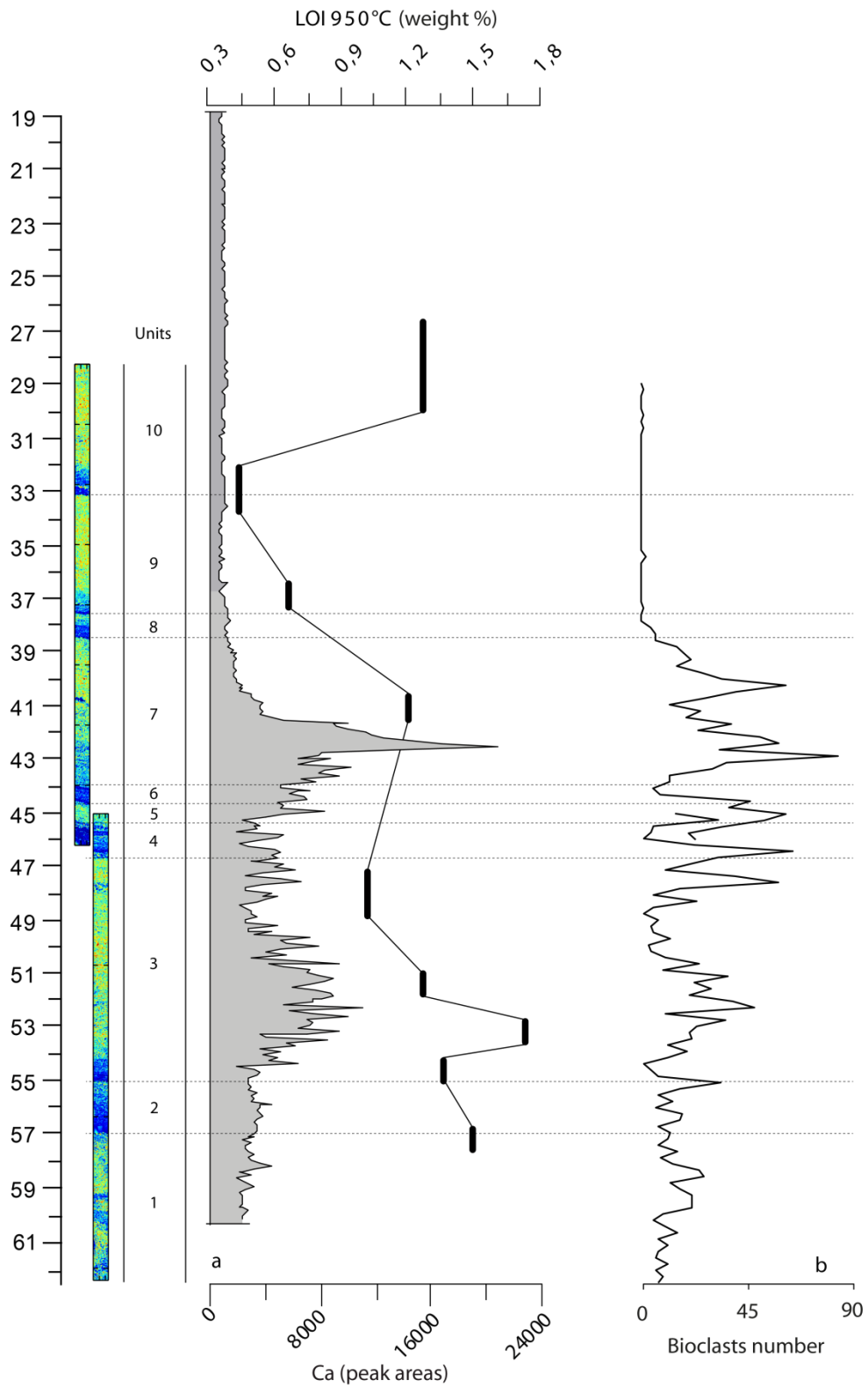
Fig. 9: Representation of the counting of bioclasts along the core, using (a) X-ray fluorescence (grey plot) and loss on ignition (Cuven et al., 2013), and (b) the bioclast code on X-CT images. While bioclasts are not located using three dimensional coordinates in the cores, they have been counted along the whole core instead of just a vertical slice, in order to ensure a good representativity of the data. Representing their quantity along a simple vertical graph allows a more straightforward reading of the data and is precise enough for stratigraphic work.
