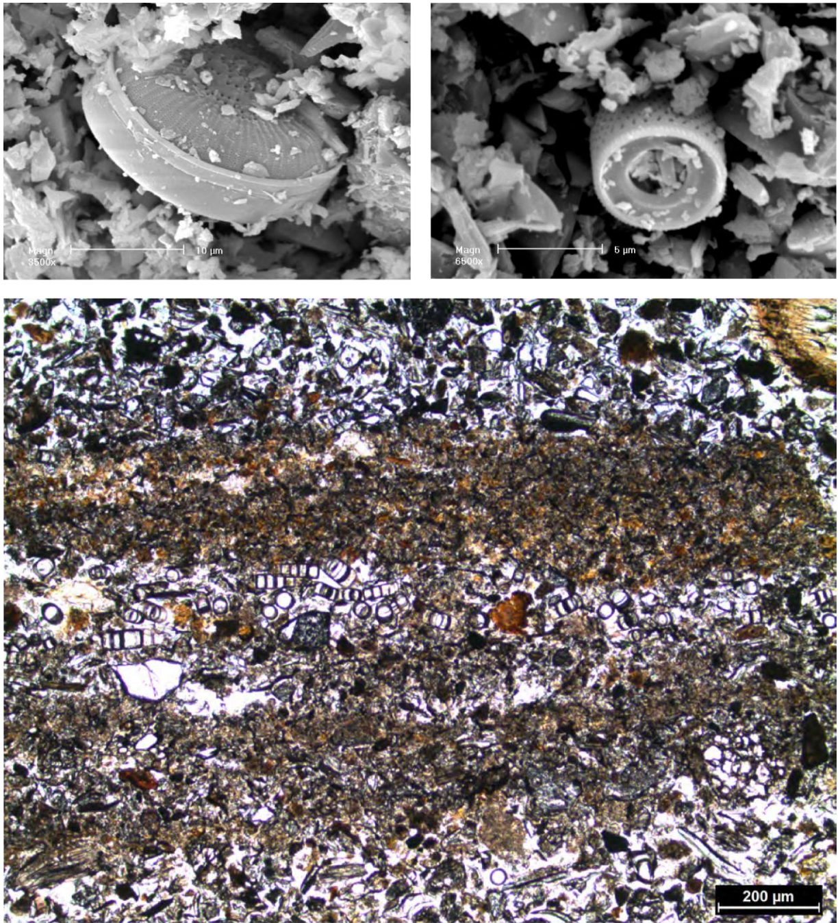
Fig. 11 - Diatoms in tsunami sample K08 viewed at the SEM and in thin sections. The distribution of diatoms in the 1996 tsunami deposits is not random, and fine-grained sub-layers or lines enriched in diatoms can be seen at the base of coarser subunits.
