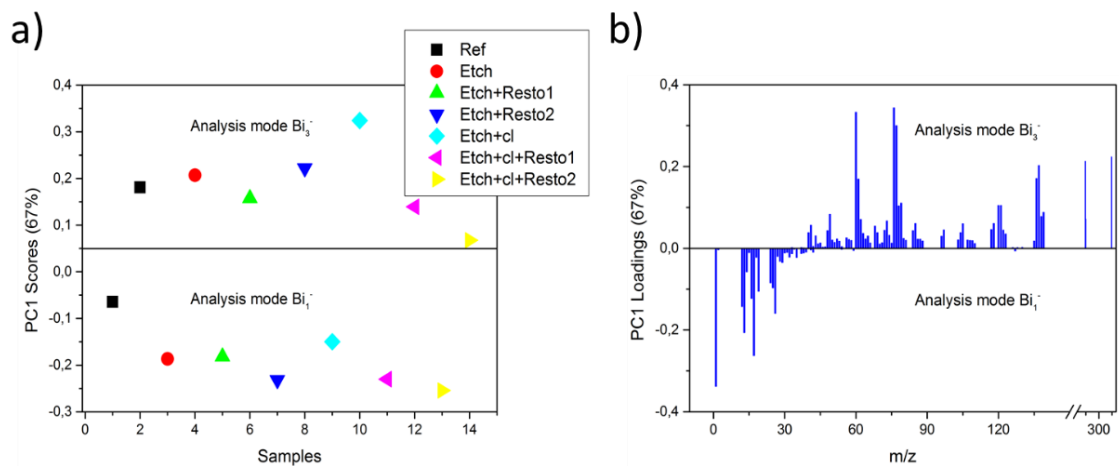
Figure 4.13: PC1 scores (a) and loadings (b) plot of low-k films data analysed with two kinds of primary ions. The PC1 Scores (67%) in the left plot show a clear separation between monoatomic Bismuth (negative scores) and Bi 3 + (positive scores). The PC1 loadings in right plot show the main peaks responsible for the separation observed on scores plot.
