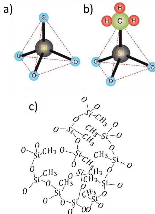
Figure 4.2: Schematic representation of a) a tetrahedral silica unit and b) the same unit of SiOCH material. c) Representation of a carbon silica doped SiOCH material cross-linked after CVD deposition [163].
