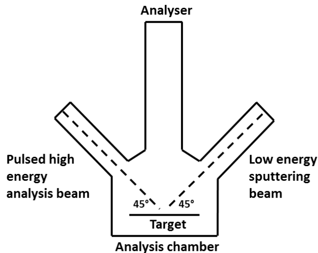
Figure 1.25: Setting of the ToF-SIMS used in this study with the two ion sources tilted of 45^\circ to the normal of the target. A third gas cluster ion gun (GCIB) equips the instrument also inclined at 45^\circ to the front of the analysis chamber upon the load lock chamber (not shown here).
