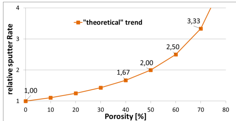
Figure 2.8: “Theoretical” sputter rate trend of a material with an increasing overall porosity rate.
