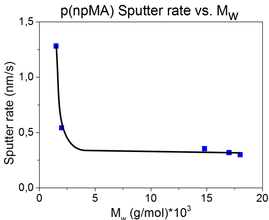
Figure 3.11: Sputter rates vs. molecular weight measured for p(npMa) samples by in-depth profiles ToF-SIMS cluster argon sputtering. Sputtering setting: \text{Ar}_{2500}^+ at 5 \text{ ke} , 0.4 \text{ nA}
