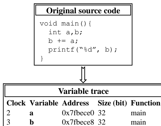
Figure 4.3: Variable Trace
