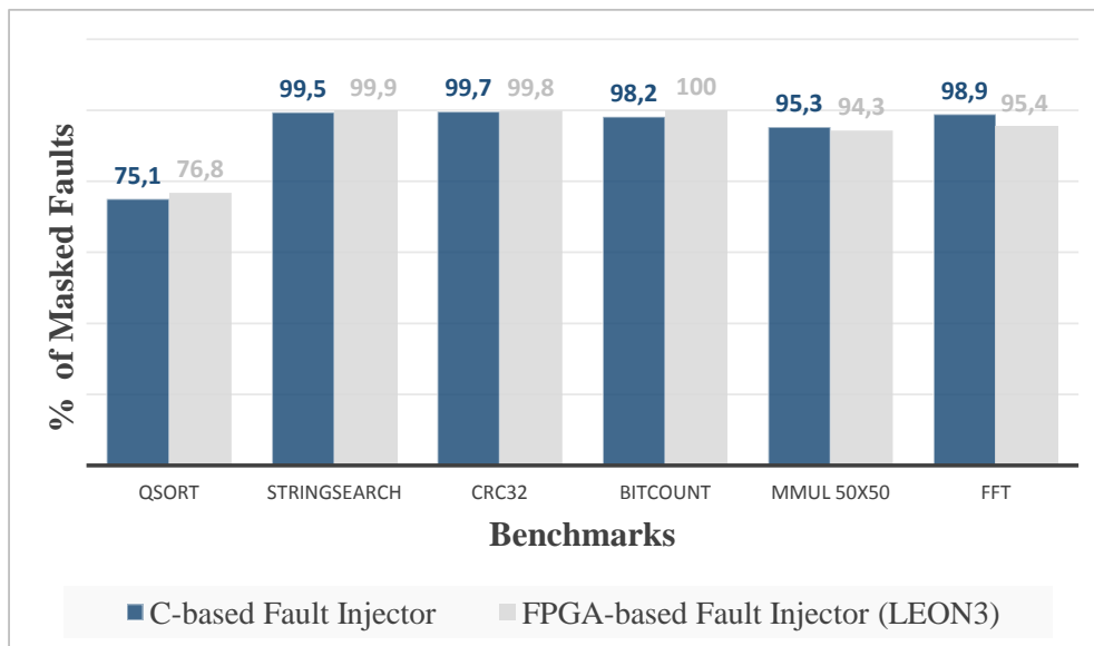
Figure 5.14: Masked Faults Injected in Data Cache using C- and FPGA-based Fault Injection
