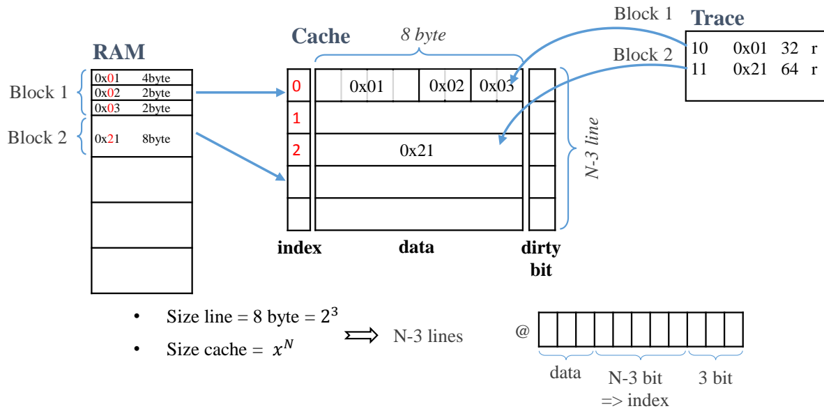
Figure 5.7: Direct-Mapped Cache
