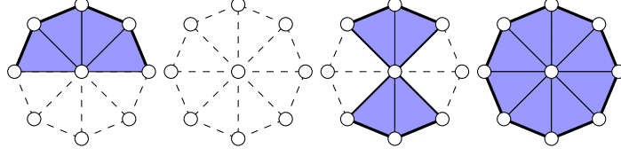
Figure 2.10: From left to right: the lower star and lower link of a regular point, a minimum, a saddle and a maximum for a bidimensional manifold.
