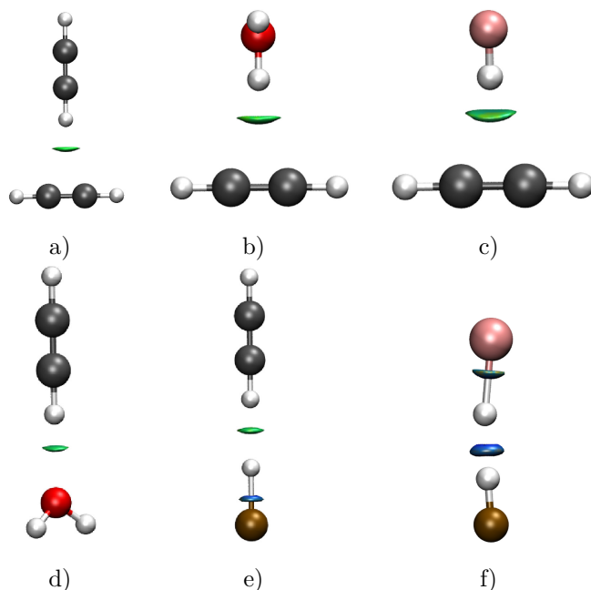
Figure 7.2: NCI isosurfaces for (a) \text{HCCH} \cdots \pi , (b) \text{HOH} \cdots \pi , (c) \text{FH} \cdots \pi , (d) (\text{HCCH}) \cdots \text{OH}_2 , (e) \text{HCCH} \cdots \text{HLi} and (f) \text{FH} \cdots \text{HLi} . 3D isosurfaces were produced using cut-off values of s(\mathbf{r}) = 0.5 and coloured over the range -0.05(\text{blue}) < \text{sign}(\lambda_2)\rho < 0.05(\text{red}) .
