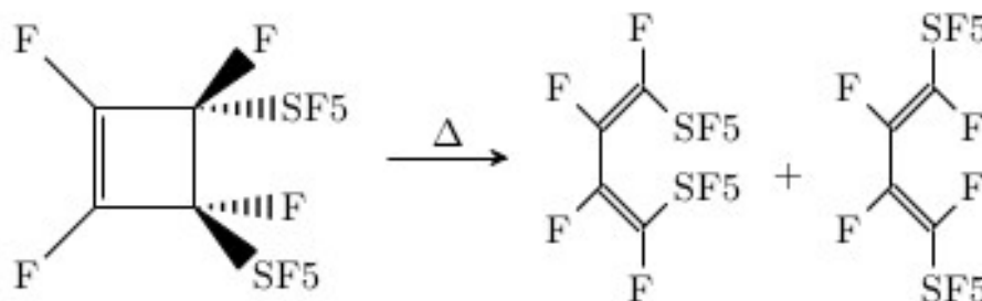
Figure 8.1: “Outwards” and “inwards” conrotatory product for the thermal ring opening of trans -1,2,3,4-tetrafluoro-3,4-bis(pentafluorosulfanyl)cyclobutene.
