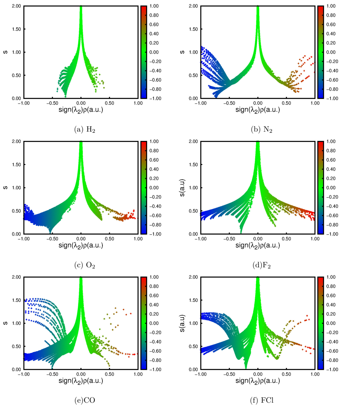
Figure 6.4: s(\mathbf{r}) along intermolecular axis for a) \text{H}_2 , b) \text{N}_2 , c) \text{O}_2 , d) \text{F}_2 , e) \text{CO} .
