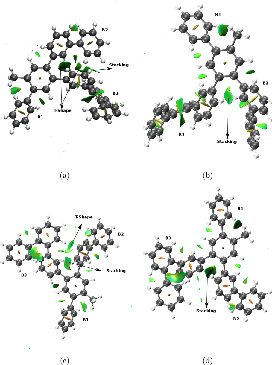
Figure 4.10: NCI results for the four sexiphenyl conformers. NCI regions corresponding to stacking and T-Shape interactions have been labelled a) structure 1, b) structure 2, c) structure 3 and d) structure 4. s(\mathbf{r}) = 0.5 isosurfaces coloured over the range and color scale -0.04(\text{blue}) > \text{sign}(\lambda_2)\rho < 0.04 (red).
