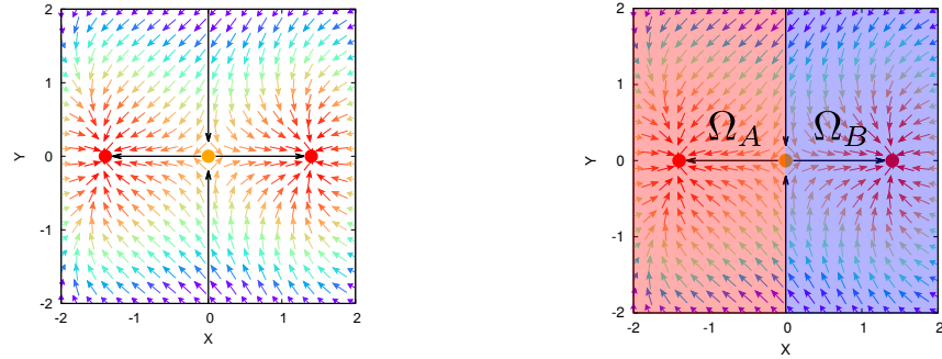
Figure 2.8: (Left) f(x, y) = -x^4 + 4(x^2 - y^2) - 3 vector field, \vec{\nabla} f(x, y) . The thick black lines are symbolic representations of the integral lines connecting the CPs. (Right) Topological partition obtained from \vec{\nabla} f(x, y) . \Omega_a and \Omega_b stand for the stable manifolds of each of the maxima of f(x, y) .
