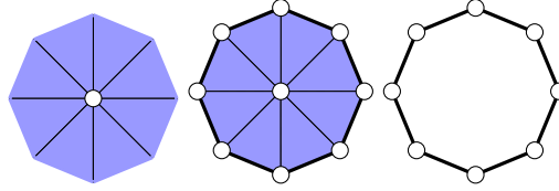
Figure 2.9: From left to right: the star, the closed star and the link of a point in a bidimensional manifold.
