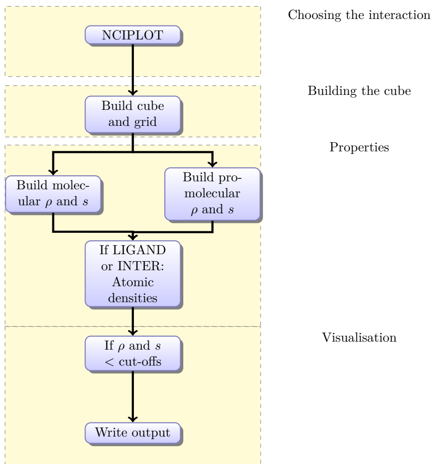
Figure 5.1: Flowchart for program routines for non-covalent interactions visualisation in NCIPlot. The flow is divided into four main algorithmic parts: input, cube construction, properties, and visualisation
