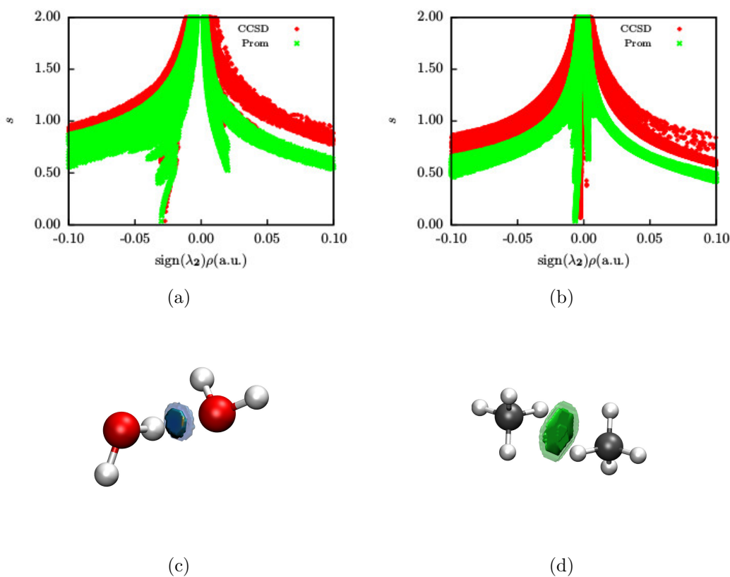
Figure 5.7: Comparison of NCI CCSD/6-311G and promolecular for test molecules. CCSD and promolecular integrated volumes are displayed as solid and transparent iso-surfaces respectively: (a, c) water dimer and (b, d) methane dimers
