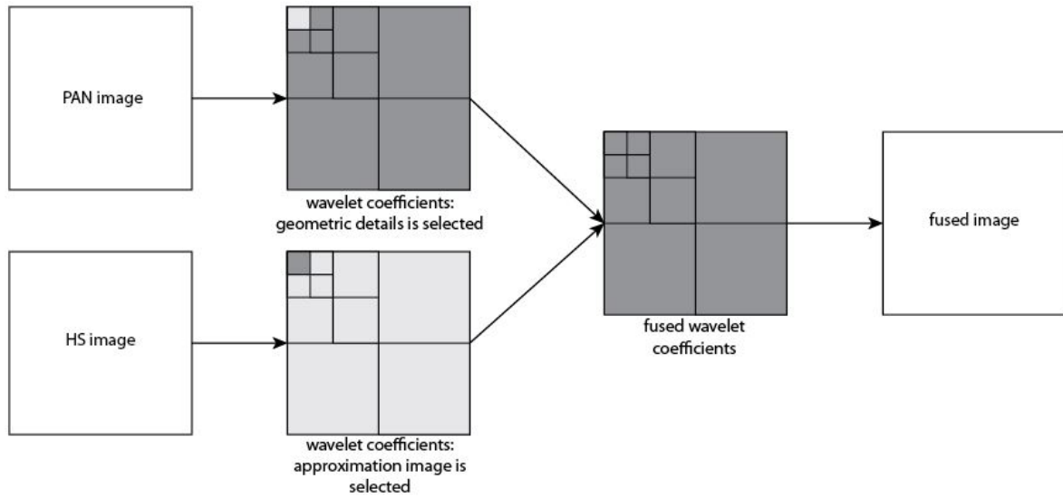
Figure 2.5: Wavelet concept
