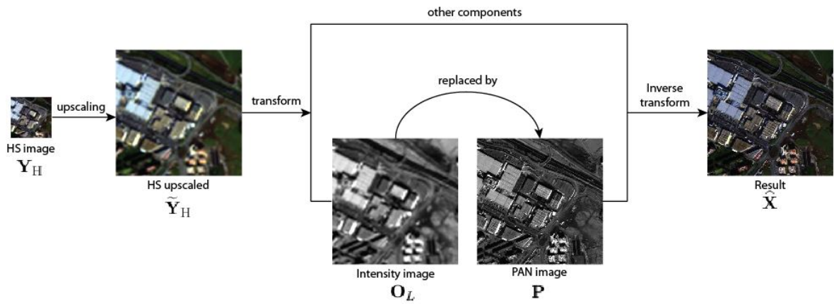
Figure 2.1: CS concept
