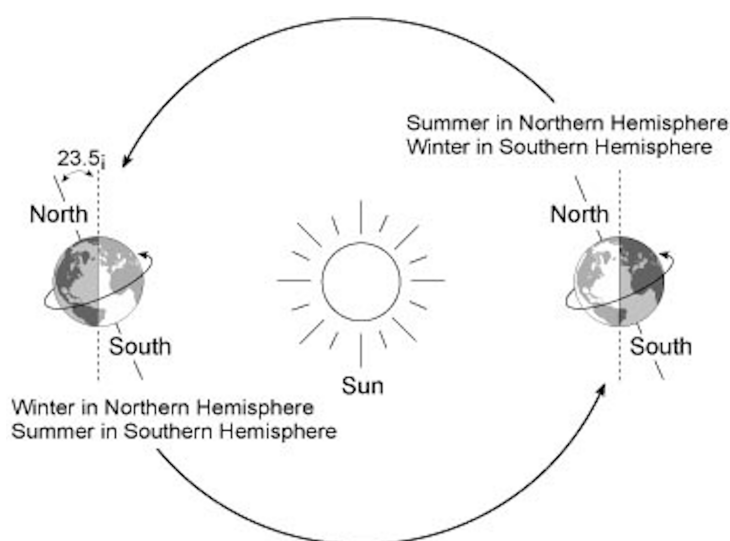
Figure 10. Geophysical properties of the earth's rotation and seasonal changes.
