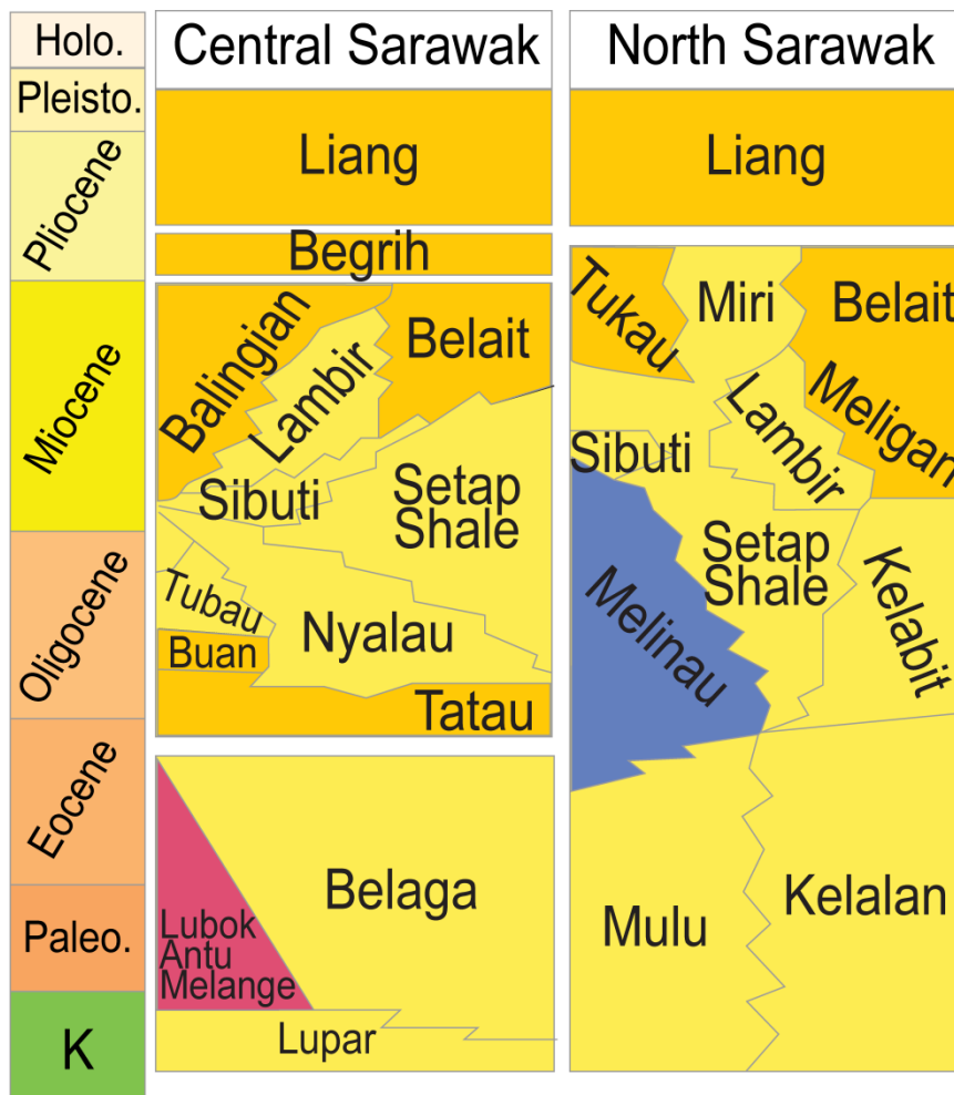
Figure 2.5. Generalized stratigraphy of central and north Sarawak.
