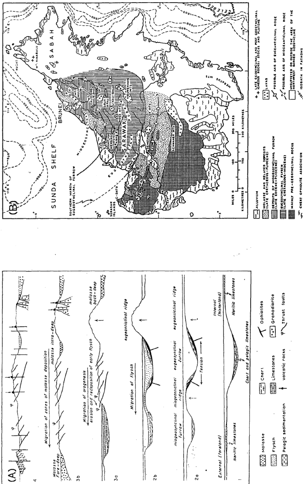
Figure 2.4. The Northwest Borneo Geosyncline (Haile, 1968).
