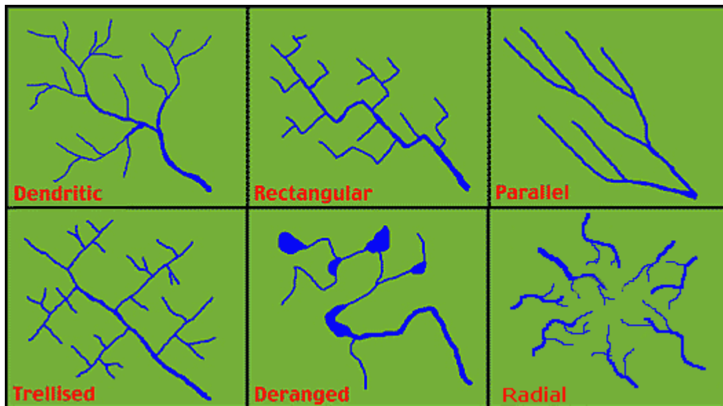
Figure 1.1 Some of the most commonly encountered drainage patterns. Figure source: https://laulima.hawaii.edu .
