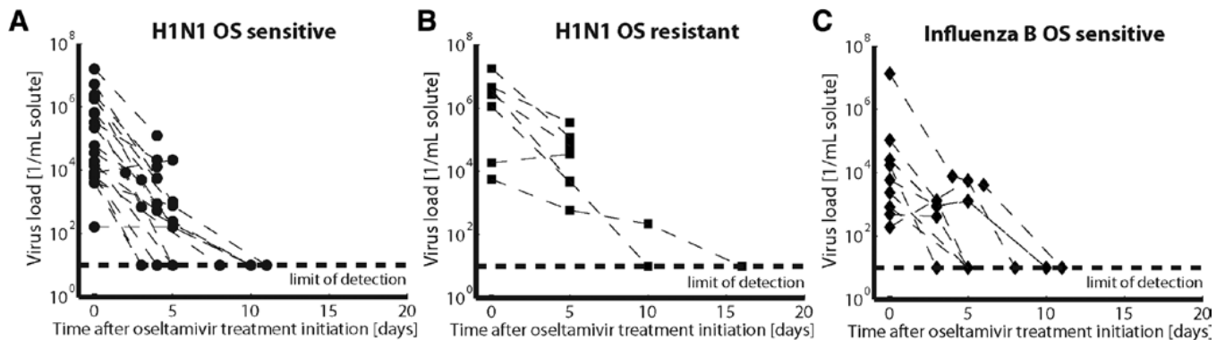
FIGURE 2. Viral dynamics after treatment initiation. A, Viral kinetics in patients infected with drug-sensitive influenza A(H1N1) 2009 (filled circles). B, Viral kinetics in patients infected with drug-resistant influenza A(H1N1) 2009 (filled squares). C, Viral kinetics in patients infected with drug-sensitive influenza B (filled diamonds).
