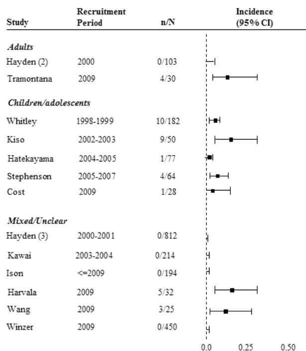
Figure 1 A: Forest plot of incidence of drug resistance in adult, pediatric and mixed trials (Source: Thorlund 2011 116 )
