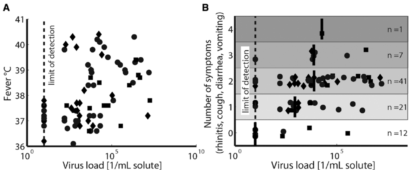
FIGURE 4. Observed correlation between virus load and fever and between the number of symptoms and virus load in nasopharyngeal secretions. A, Correlation between virus load and fever in all patients. B, Correlation between the number of symptoms observed and the measured virus load. The solid vertical bars denote the respective median virus load for each category. The number of data points available for each category is denoted at the right side of the illustration. Data from patients infected with influenza B are displayed by filled diamonds, whereas data from patients infected with drug-sensitive or drug-resistant A(H1N1) 2009 influenza viruses are depicted by filled squares and circles, respectively.
