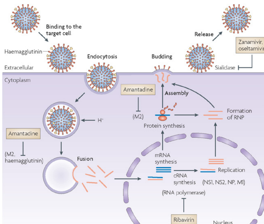
Figure 4 A: Influenza life cycle and potential drug targets (Source: von Itzstein, 2007 232 )
