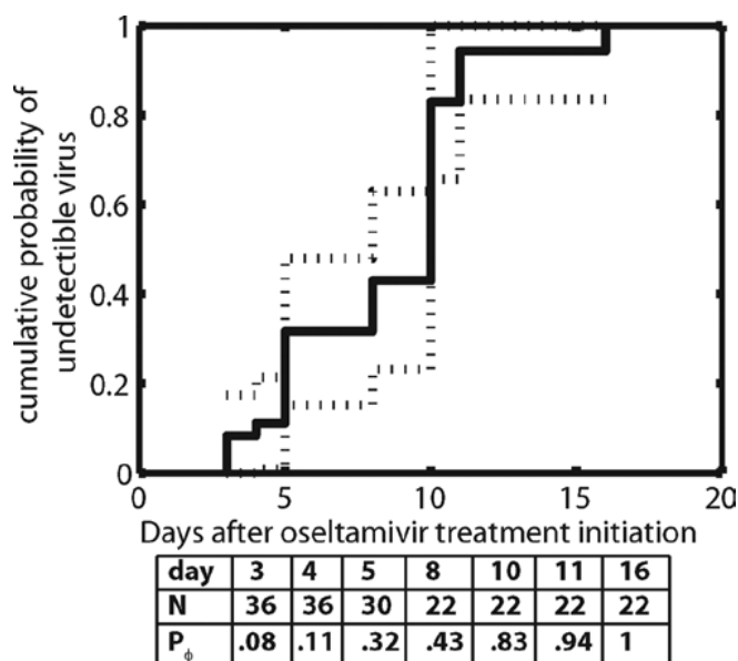
FIGURE 1. Kaplan-Meier estimate of the cumulative probability to achieve undetectable virus load. The solid lines indicate the empirical estimate of the cumulative probability to achieve undetectable virus in nasopharyngeal secretions. The dashed lines are the confidence bounds, which were computed using the Greenwood formula.
