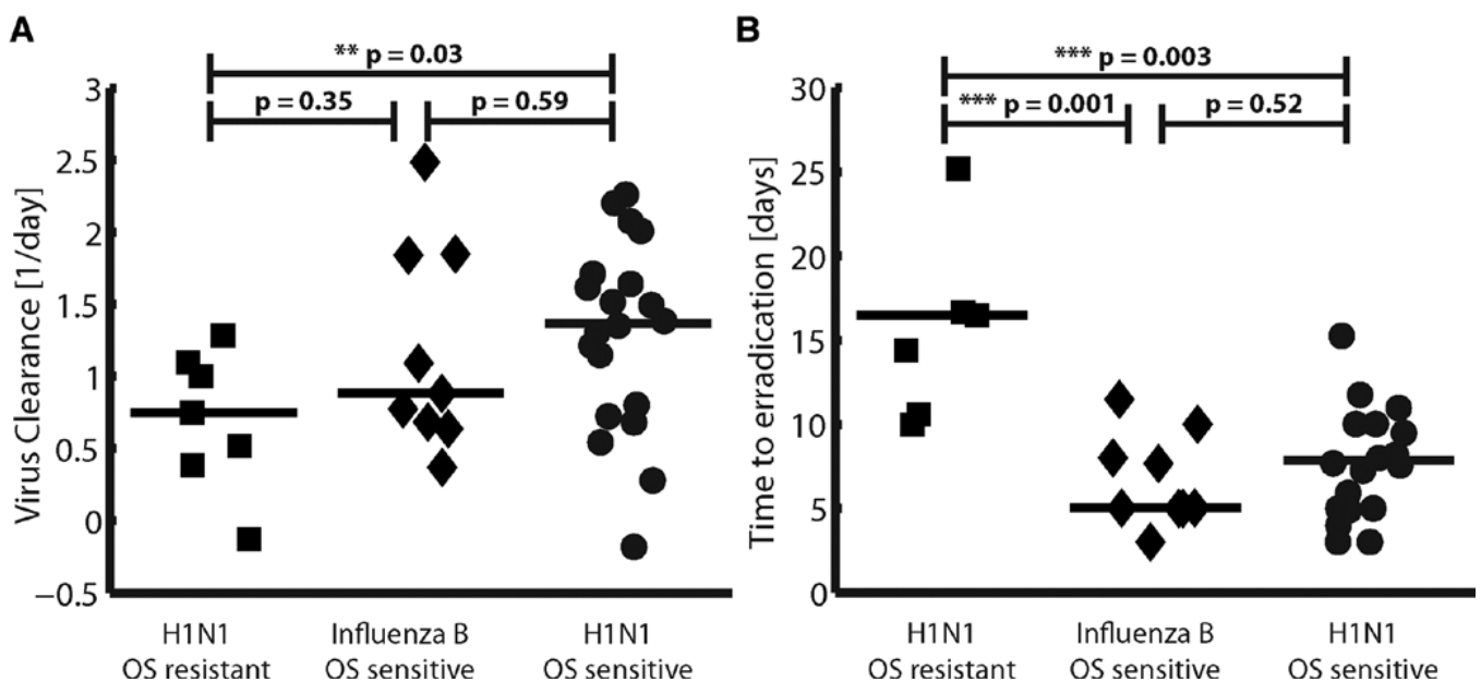
FIGURE 3. Estimated viral clearance CL_v(i) and time required to achieve nondetectable viral load in nasopharyngeal secretions. A, Estimated viral clearance. B, Estimated time to achieve nondetectable virus load after initiation of oseltamivir treatment. Estimates in patients infected with drug-resistant A(H1N1) 2009, drug-sensitive influenza B and drug-sensitive A(H1N1) 2009 viruses are depicted by filled squares, filled diamonds and filled circles. OS indicates oseltamivir.
