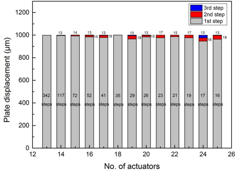
Figure II- 18: Steps to realize 1000±1 μm plate displacement with different number of controlled MPMs
