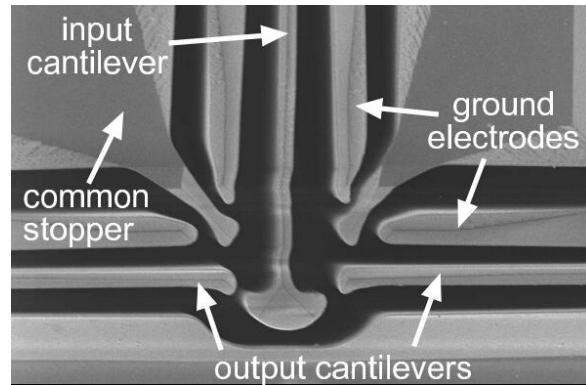
Figure I- 11: Tri-stable switch based on electrostatic actuator [OBER 2006]
