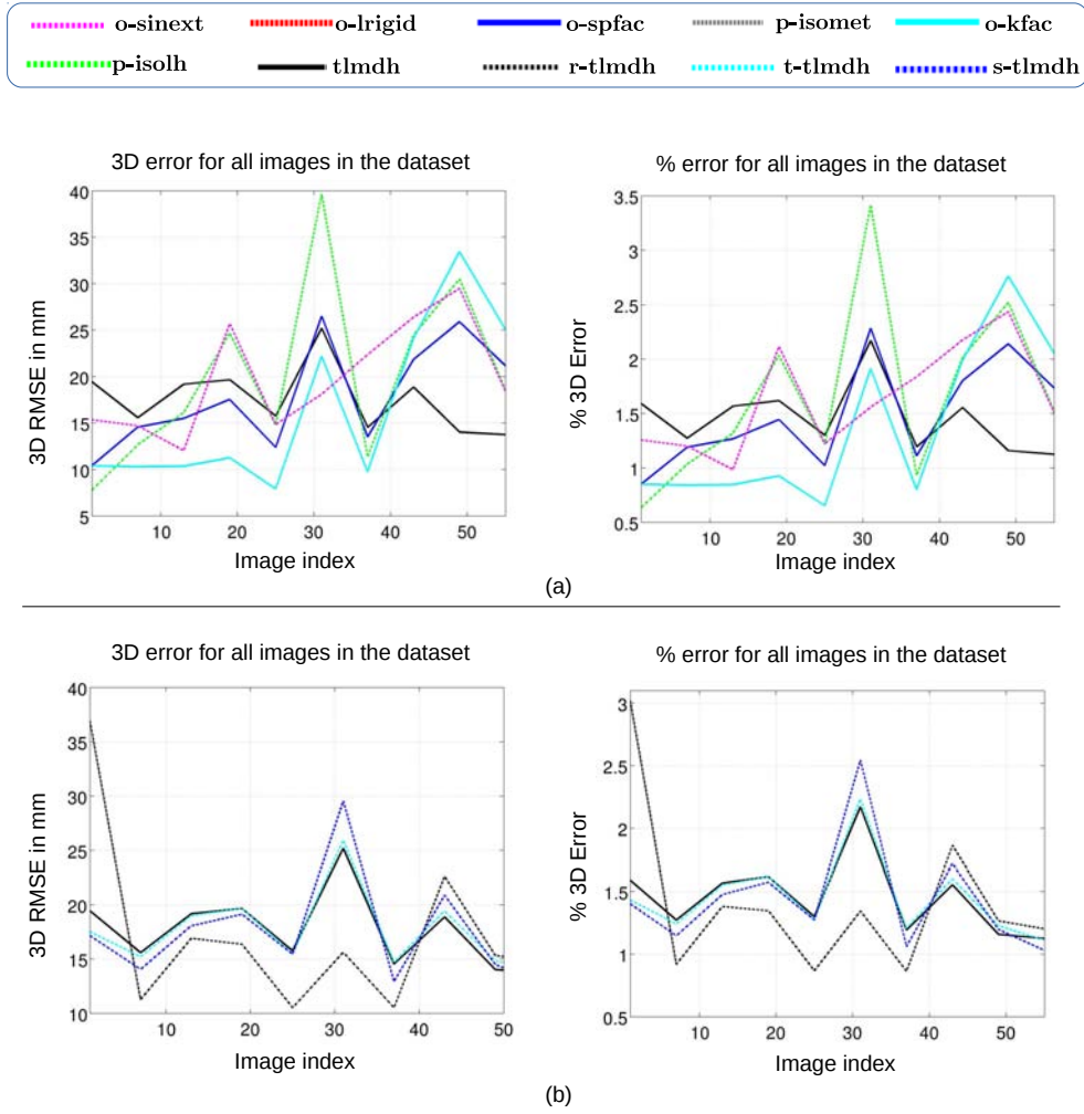
Figure 6.10: Mean 3D errors and percentage errors for all the images in the Table-mat dataset. The top row shows errors for tlmdh against the compared methods and the bottom row shows tlmdh against our other methods.
