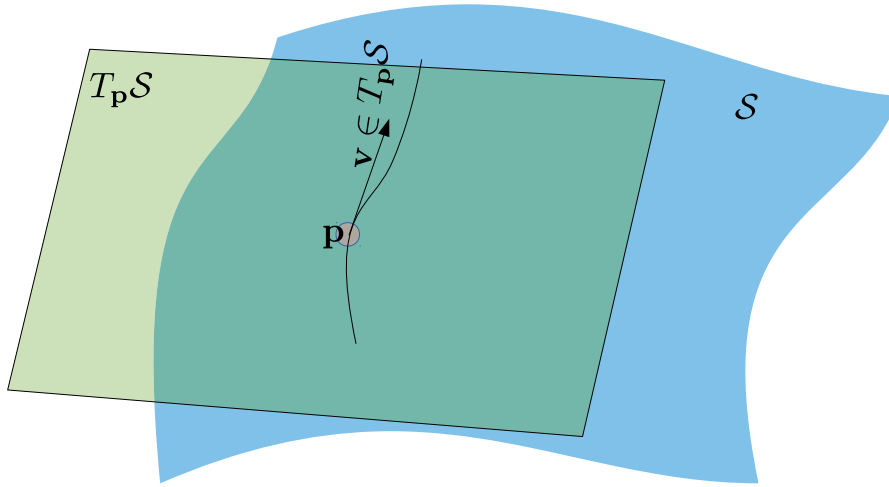
Figure 2.9: A surface \mathcal{S} and its tangent space T_p \mathcal{S} at a point \mathbf{p} .
