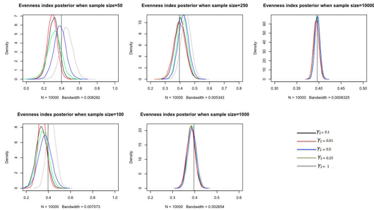
Figure 2.7: Estimated posterior densities of H(\theta) considering sample sizes of 50, 100, 250, 1000, 10,000. They correspond to the priors on \theta shown in Figure 2.6 and are based on 10^4 posterior simulations. The vertical line indicates the mode of all posteriors when sample size is large enough.
