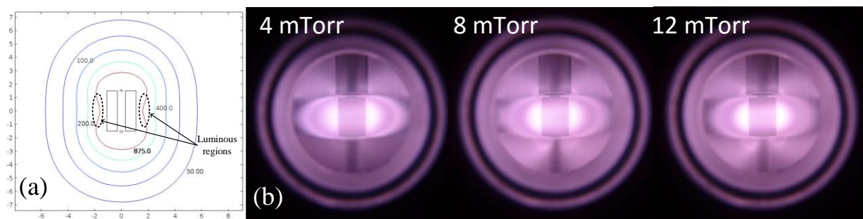
Figure 4.1. (a) Magnetic field of a single source (b) Operation of a single source for nominal power (180 W/source) and three indicative pressures.
