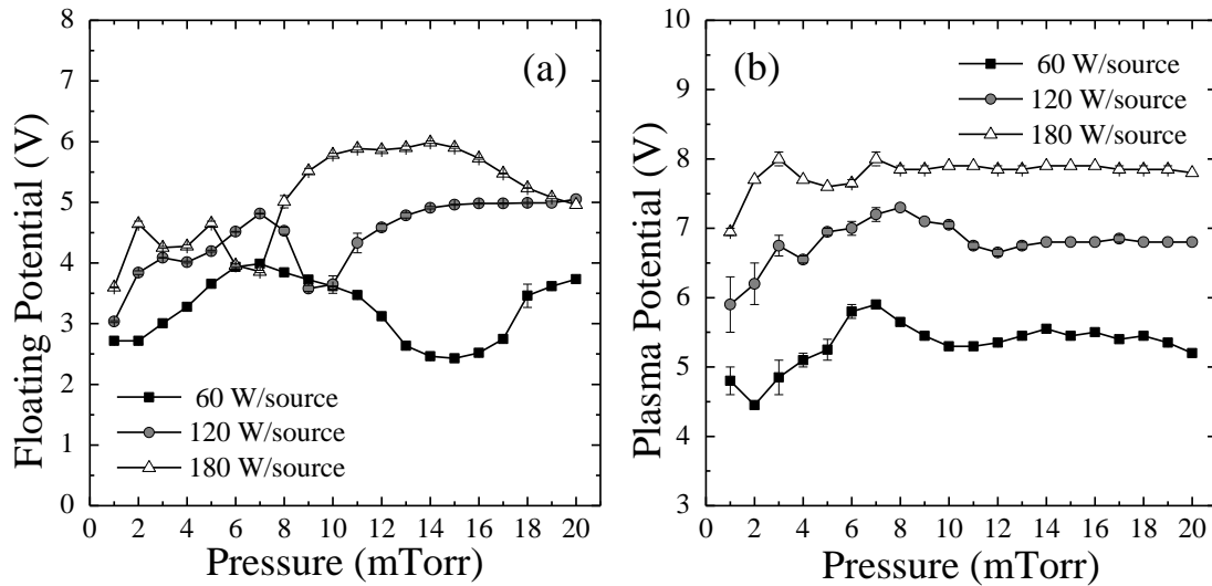
Figure 4.30. Pressure dependence of (a) floating and (b) plasma potential for configuration B. Error bars are calculated from two series of measurements.
