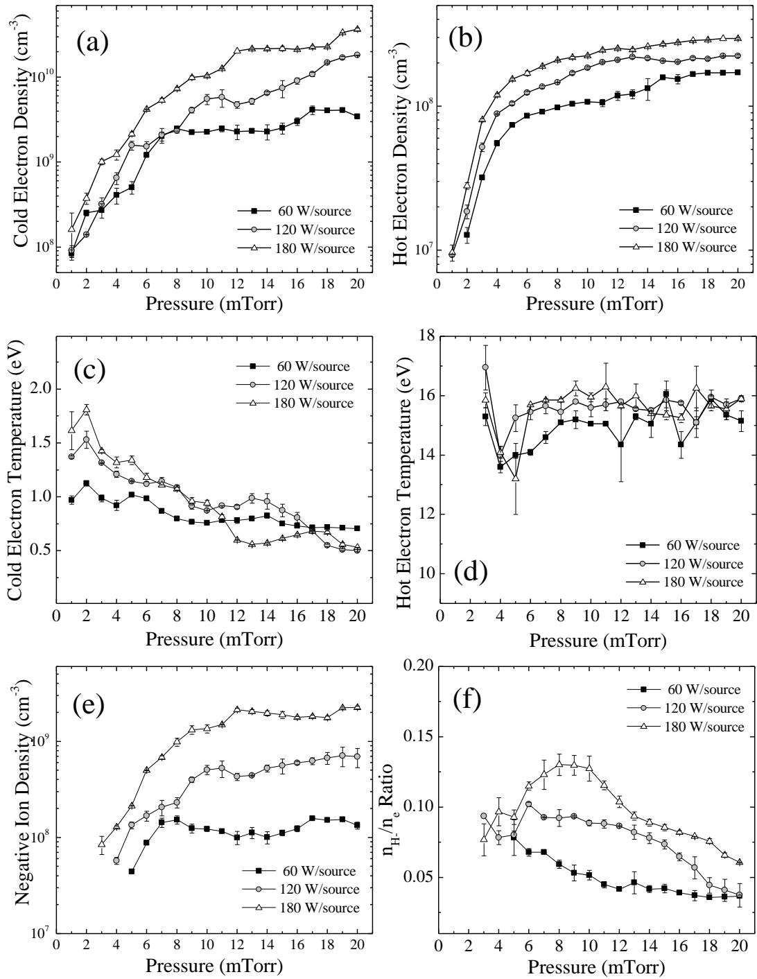
Figure 4.34. Pressure dependence of (a) cold electron density (b) hot electron density, (c) cold electron temperature, (d) hot electron temperature (e) negative ion density and (f) n_{\text{H}^-}/n_e ratio for the configuration C(Center). Error bars are calculated from two series of measurements.
