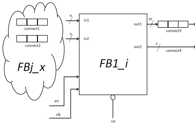
Figure 5.6 – FB equivalent architecture.
