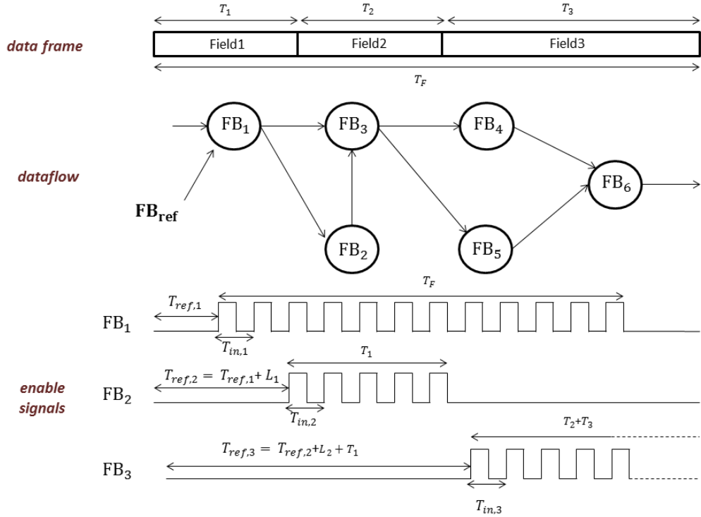
Figure 5.10 – Control algorithm illustration.
