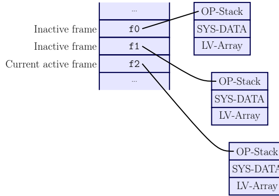
Figure 4.3: Stack Structure
