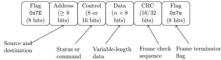
Figure 6.18: HDLC frame format
