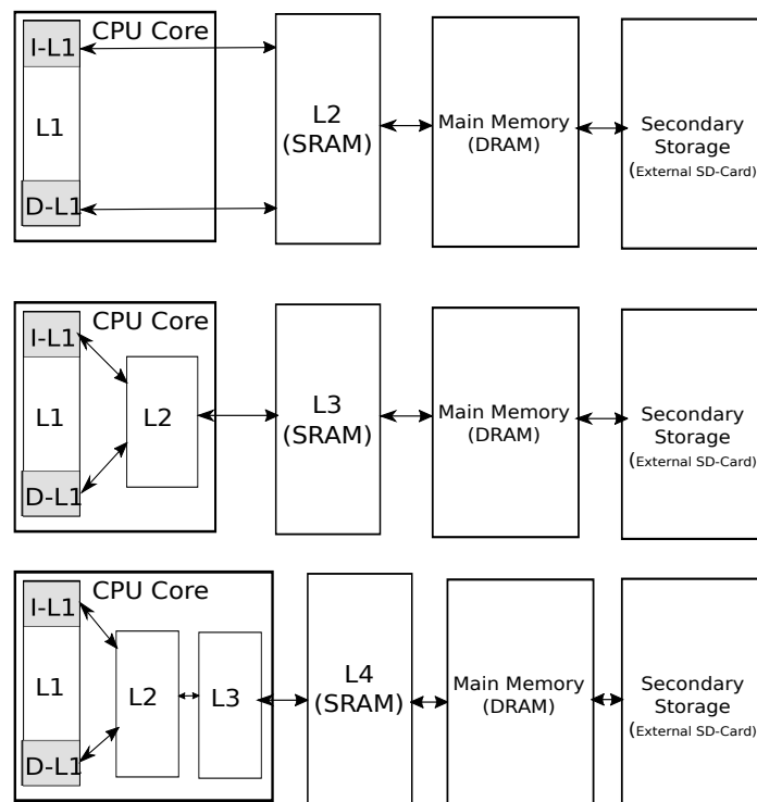
Figure 7.4: Possible Cache Levels
