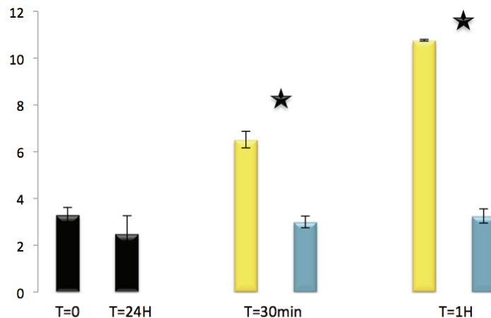
Figure 45: AsA content in tomato leaves soaked in a solution of AsA (10mM) or MS \frac{1}{4} (control). Four points are shown in graph. T=0 is the expression when leaves were harvested in the greenhouse. Before starting the experiment, leaves remained in the growth chamber during 24H to recover and to reduce any stress signal induced by the cutting; it corresponds to T=24H. Next step, leaves were soaked in solution of AsA (yellow bar) or MS \frac{1}{4} (blue bar) during 30 min or 1 hour. For each time, three leaves were analysed in technical triplicate ( \pm SD) and asterisks indicate significant differences between treatments (Student test, P < 0,05 ). AsA content is expressed in \text{nmol.mg FW}^{-1} .
