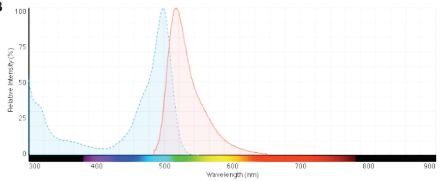
Figure 64: 2',7'-dichlorodihydrofluorescein diacetate. A. Chemical structure B. Fluorescent spectrum with in bleu excitation ( \lambda=490\text{nm} ) and red emission ( \lambda=520\text{nm} ) spectra.
