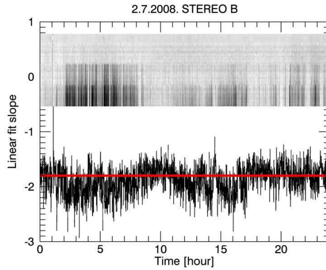
Figure 4.5: The linear fit criteria applied to 2233 spectra during 2.7.2008. on STEREO B. Daily dynamic spectrum is shown at the top while the slopes from \lg f, \lg V^2 linear fitting are given in black. Red line represents the slope equal to -1.8 and all the spectra below the line are excluded. The time shown on the x axis is also valid for the summary plot
