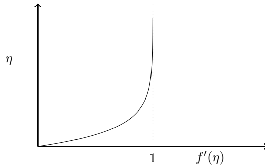
Figure 2.4: The Blasius profile.
