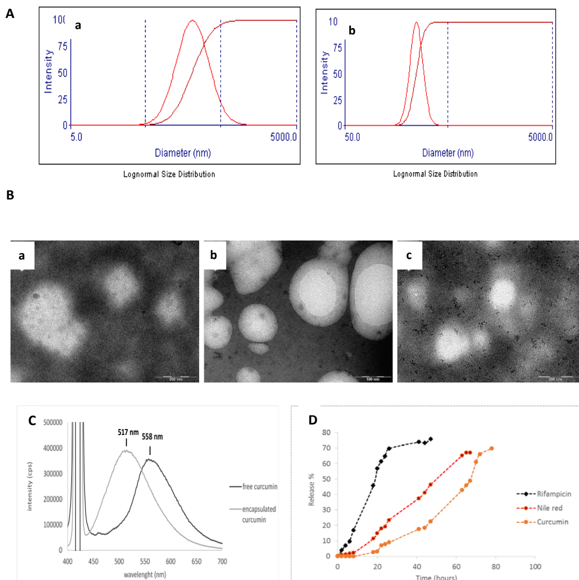
Figure 4: Characterization of Carrageenan-graft-PCL: (A) Size distribution of empty micelles (a) and curcumin-loaded micelles (b) by Dynamic Light Scattering (DLS); (B) TEM images of empty micelles (a) Nile red loaded micelles (b) and curcumin-loaded micelles registered at a concentration of 0.5 or 1 mg.mL -1 ; (C) Characterization of free curcumin and encapsulated curcumin by fluorescence. Excitation was performed at 420 nm, and the maximum emission wavelength of free curcumin and curcumin-loaded micelle was detected at 558 nm and 517 nm respectively. (D) kinetics of release of curcumin, Nile red and rifampicin from Carrageenan-graft-PCL micelles. The concentrations of lipophilic molecule released in the medium during time was measured either by fluorescence (excitation wavelength = 550nm – emission wavelength = 630nm) for Nile Red, or by absorbance (at 420nm for curcumin and 475nm for rifampicin).
