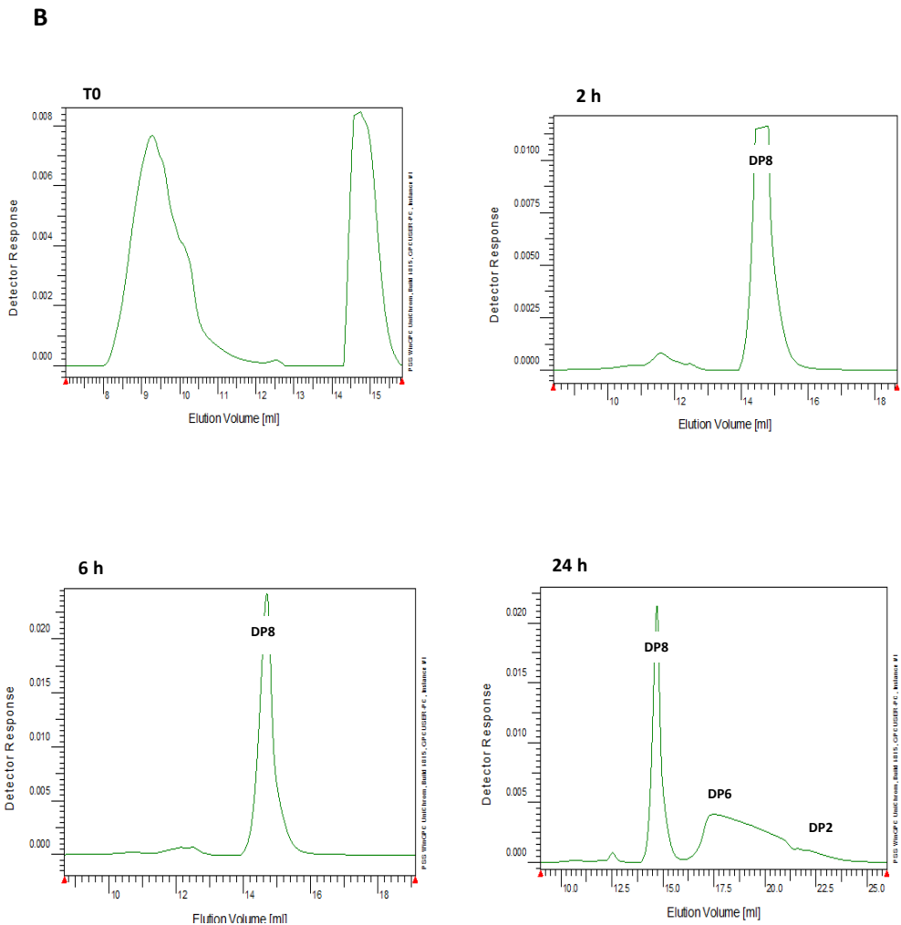
Figure 1: Hydrolysis of \kappa -carrageenan using \kappa -carrageenases isolated from Pseudoaltermonas carrageenovora . Degradation was analysed by quantification of reducing ends of carrageenan (A). Size exclusion chromatography allowed to determine carrageenan chain length after hydrolysis (B). DP correspond to the degree of polymerisation (or number of repeat unit).
