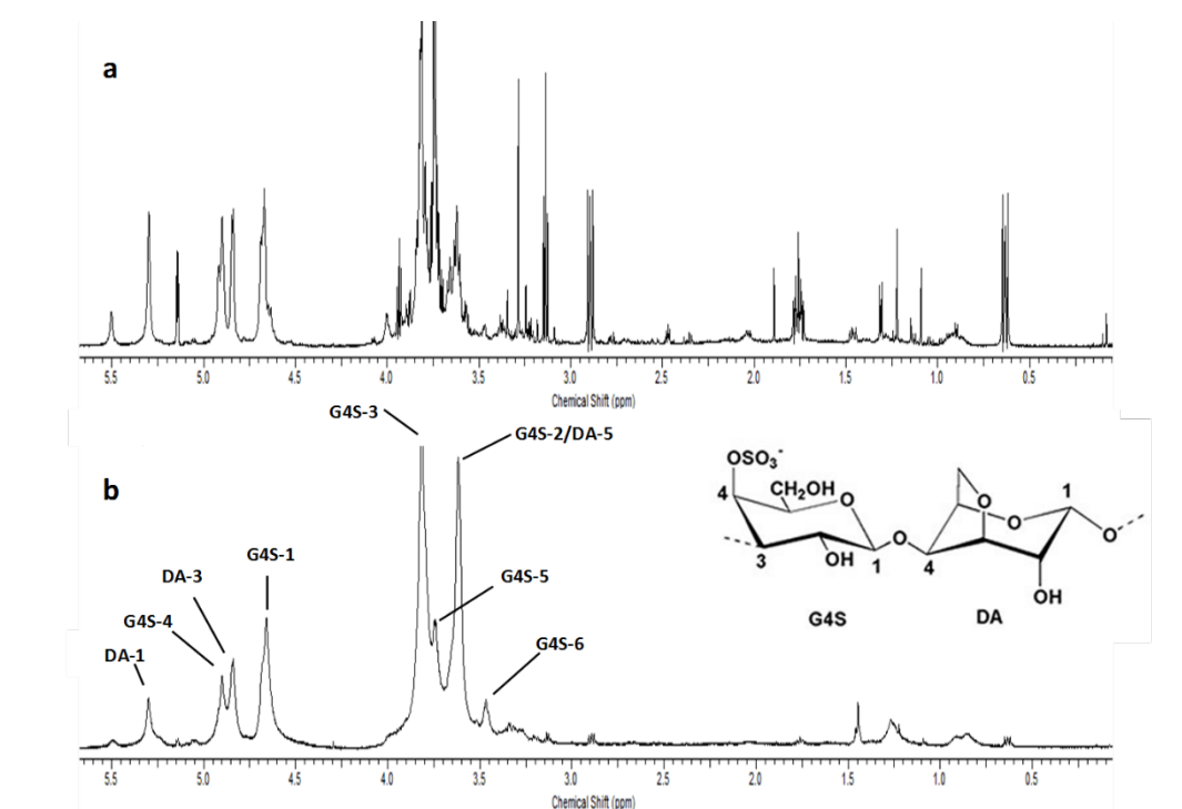
Fig. 5. 1 H NMR Spectra of an extract of Eucheema Denticulatum obtained using ultrasounds: (a) Untreated algae, (b) pre-treated algae with 80% ethanol. Signals corresponding to kappa-carrageenan monomers (letter coded G4S-DA) are identified.
