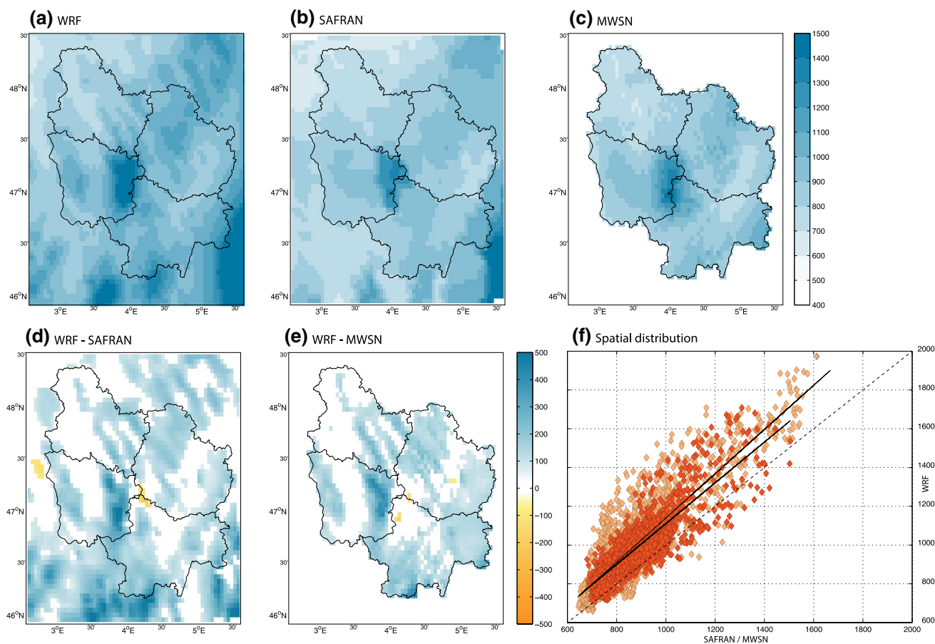
Fig. 10 As Fig. 2 but for annual mean precipitation amounts (mm)
