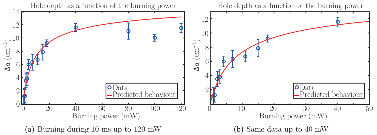
Figure 6.18 – Evolution of the absorption hole depth as a function of the increasing burning power. (a) Power increased up to 120 mW. It seems that there is a deviation from the predicted behaviour at high burning power. (b) Zoom over the low burning powers. The model seems to be in good agreement with experimental data up to 40 mW.
