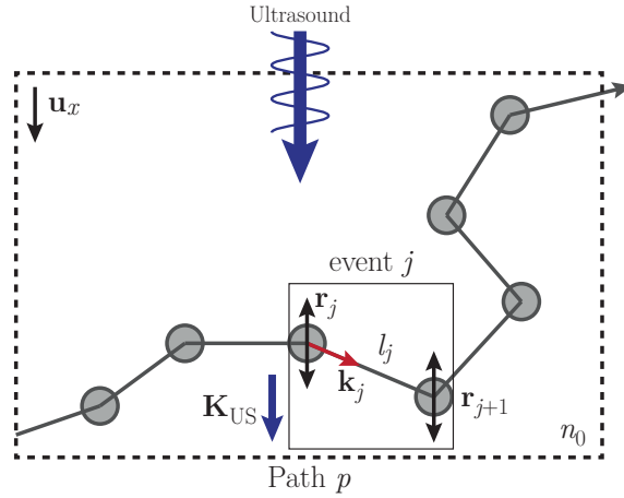
Figure 2.5 – Schematic of the parameters used in the acousto-optic effect model.
