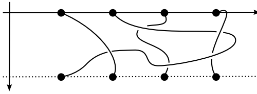
FIGURE 1. A physical braid \beta .
