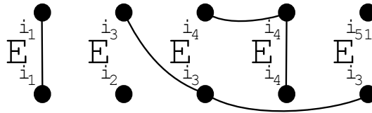
FIGURE 10. \sum_{i_1, i_2, i_3, i_4, i_5} E_{i_1}^{i_1} \otimes E_{i_2}^{i_3} \otimes E_{i_3}^{i_4} \otimes E_{i_4}^{i_4} \otimes E_{i_3}^{i_5} = \rho_N^{\mathcal{P}_5}(p_1) .
