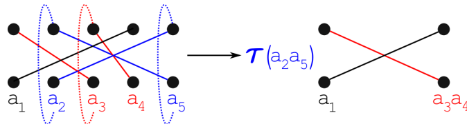
FIGURE 2. Graphical computation of tr_{\{2,3,5\}}(\sigma_1, \mathbf{a}_1) .
