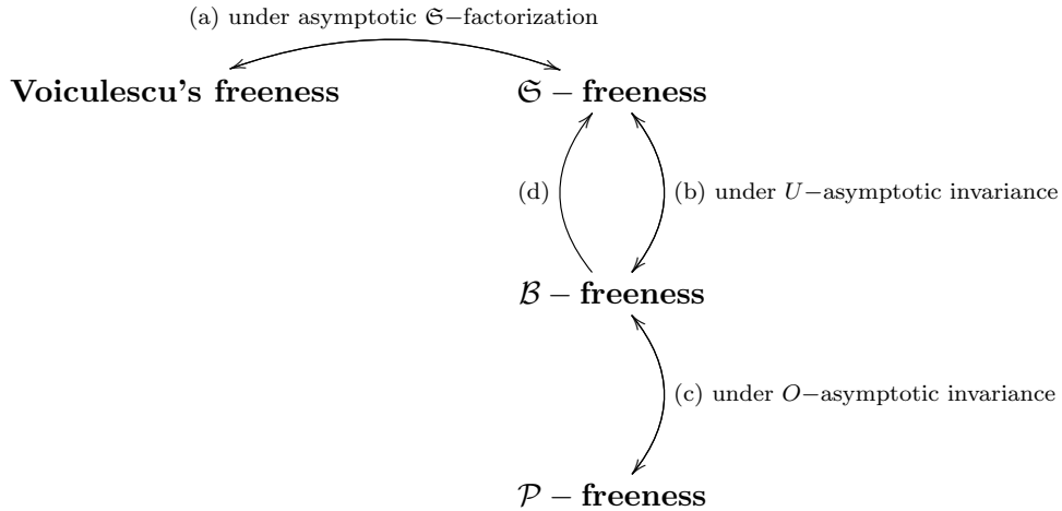
Diagram 1. The different notions of freeness.
