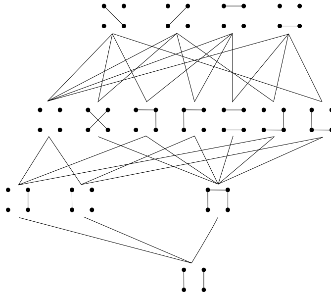
FIGURE 11. The graph \mathbb{G}'_2 .
