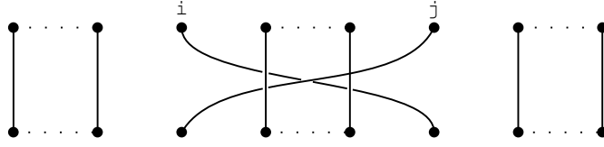
FIGURE 17. The braid \beta_{(i,j)} .
