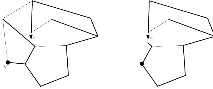
FIGURE 12. The restriction of \mathbb{G} used in Proposition 6.1.
