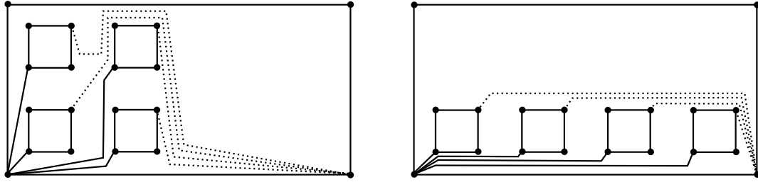
FIGURE 20. Graphs \mathbb{G}_1 and \mathbb{G}_2 .
