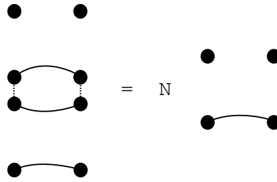
FIGURE 7. Example of a product which involves the counting of loops.
