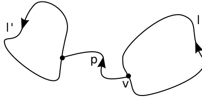
FIGURE 8. Two simple loops l, l' with a path p joining l to l' .
