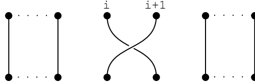
FIGURE 4. The elementary braid \beta_i .
