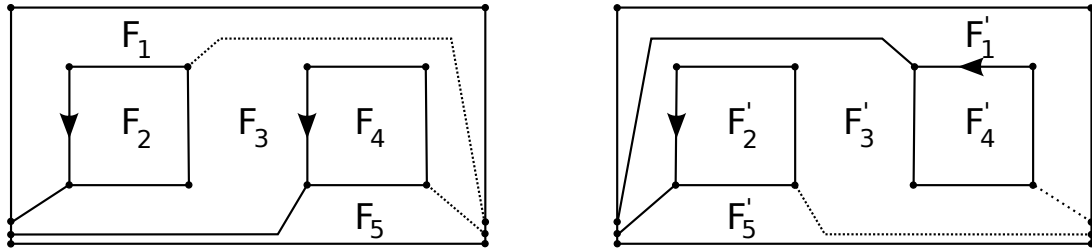
FIGURE 21. The graphs \mathbb{G}_1 and \mathbb{G}_2 .
