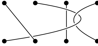
FIGURE 3. A diagram associated with \beta .
