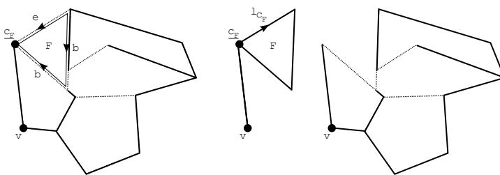
FIGURE 14. Decomposition when \mathbb{G}_l has as many faces as \mathbb{G} .
