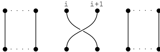
FIGURE 8. La tresse \beta_i
