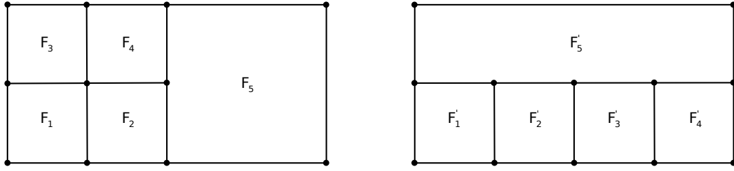
FIGURE 19. Graphs \mathbb{G} and \tilde{\mathbb{G}} .
