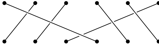
FIGURE 18. The braid \beta_{\mathbf{k}} , \mathbf{k} = (2, 3, 6) .
