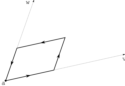
FIGURE 3. Chemin p_a^{v,w}(\epsilon)
