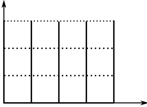
FIGURE 10. The spanning tree T .
