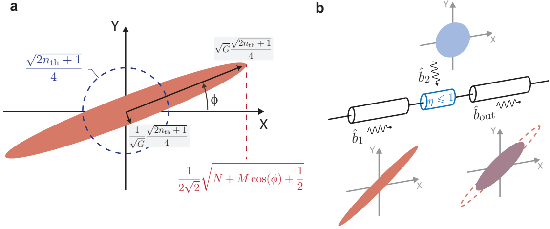
FIGURE 9.4: Squeezed vacuum. a Squeezed state produced by a phase-sensitive amplifier of power gain G whose input is a thermal state of occupancy n_{th} , fully characterized either by G and n_{th} or by the numbers N and M defined in Eqs. 2.17 & 2.18. b Attenuation of a squeezed state.
