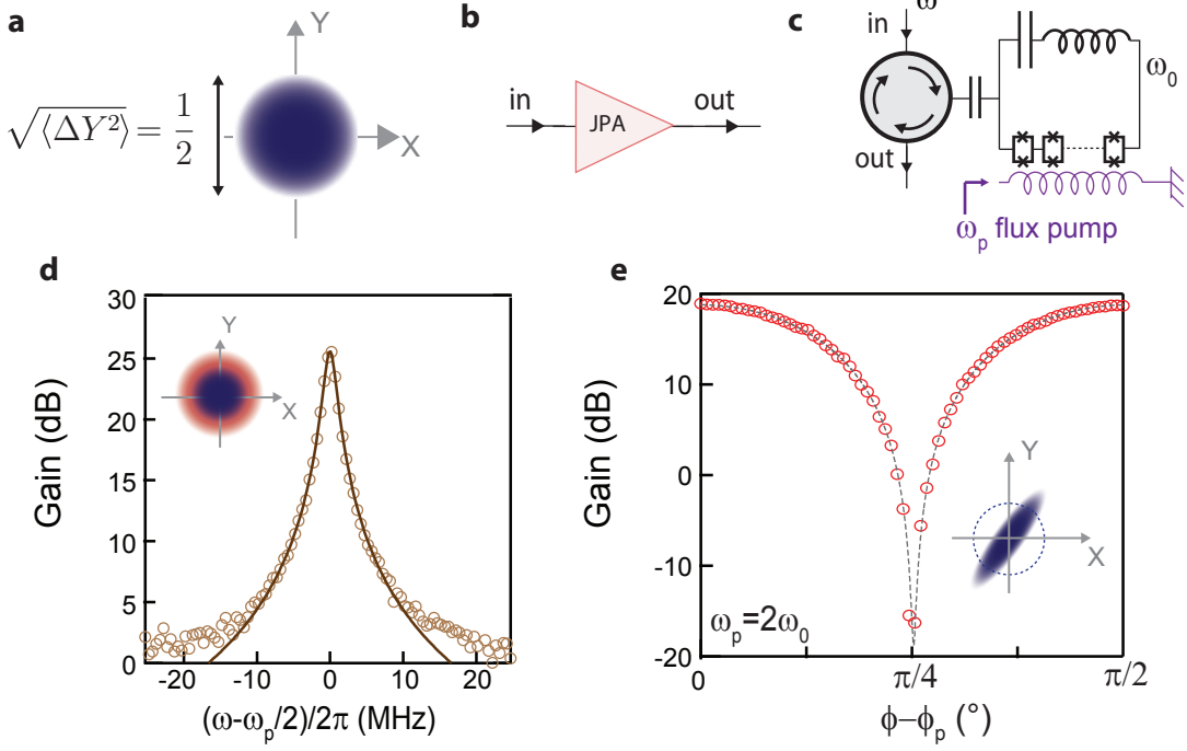
FIGURE 1.1: Quantum fluctuations and quantum-limited amplification. a At temperatures k_B T \ll \hbar\omega , the ground state of the microwave field is reached, with its quadrature variances given by \sqrt{\langle\Delta X^2\rangle} = \sqrt{\langle\Delta Y^2\rangle} = 1/2 imposing a minimum to the field fluctuations (blue shade). b-c A Josephson Parametric Amplifier, here implemented by a flux-pumped SQUID resonator, can be used to detect quantum microwave fields. d When employed in non-degenerate mode ( \omega_p \neq 2\omega ), the JPA adds half a noise photon (red shade) to the half-noise photon (blue shade) arising from the input vacuum fluctuations. e When operated in its degenerate mode ( \omega_p = 2\omega ), it amplifies one quadrature at the expense of the other; in this case the amplification is noiseless. Acting on a vacuum state, it produces a squeezed state, with fluctuations deamplified for one quadrature but amplified on the other one (blue shade).
