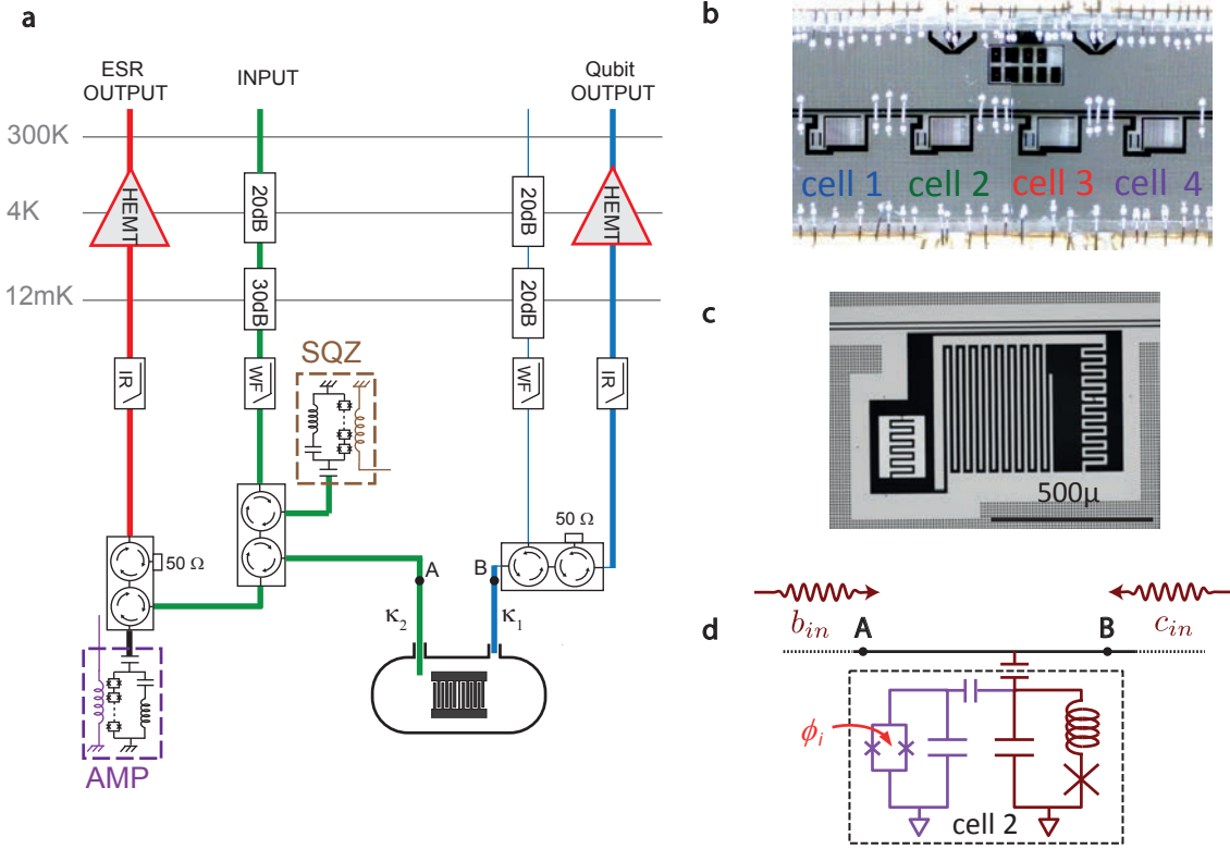
FIGURE A.1: a Microwave setup used during the squeezing experiment (see ch. 9) b Optical micrograph of the device used for estimating the number of thermally excited photons in \hat{b}_{in} . Four cells, each one composed of a transmon qubit with an attached readout resonator are probed with a single microwave feedline. c Zoom on one of the cells, showing the tunable transmon qubit (to the left) capacitively coupled to the readout resonator (to the right), itself capacitively coupled to the feedline (to the top). d Simplified electric circuit of the cell used for the calibration. The qubit contains a split Josephson junction and its resonance frequency can be tuned by threading the loop with a magnetic flux \varphi . The resonator, which contains an array of junctions, is slightly non linear. Thermal excitations in the resonator are due to both right and left traveling modes \hat{b}_{in} and \hat{c}_{in} in the feedline.
