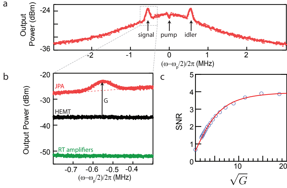
FIGURE 5.7: SNR enhancement brought by the JPA as measured by a spectrum analyser. a Output power spectrum with acquisition bandwidth 100 kHz for a coherent signal sent at \omega while the JPA is pumped at \omega_p \approx 2\omega , evidencing signal and idler as well as the noise added by the JPA. b Zoom on the signal showing the rise of the noise level compared to amplification with the HEMT and compared to amplification with the room-temperature amplifiers. It evidences a reduction of the noise referred to the input of the amplification chain when turning on the JPA. c SNR as a function of the JPA gain.
