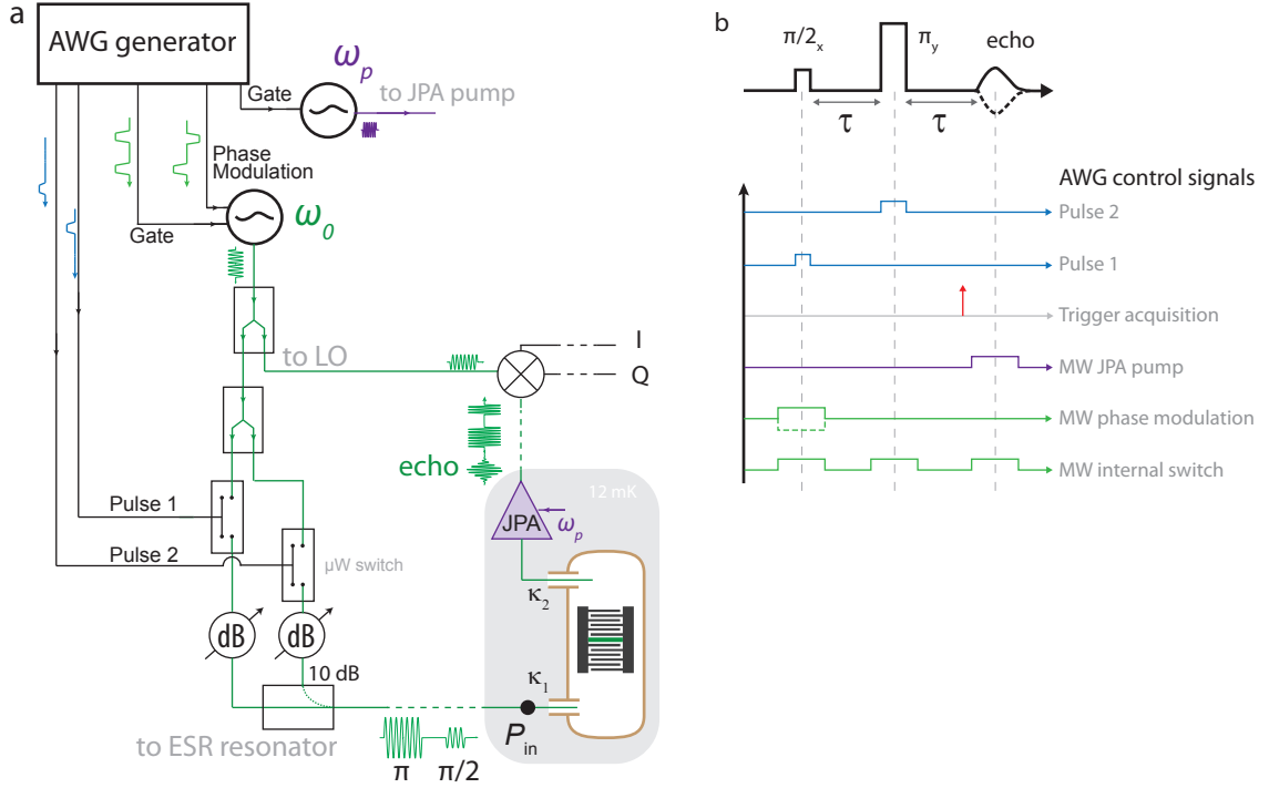
FIGURE 6.1: Pulsed ESR implementation. a Two independent microwave pulses can be generated via two microwave switches in parallel, each being in series with a tunable attenuator to control the pulse input power P_{\text{in}} referred to port 1 of the resonator. The pulses' phases are set via phase modulation of the microwave source. All signals are controlled via an AWG generator. b Control signals for a Hahn-echo sequence. The JPA is switched on only during the echo emission.
