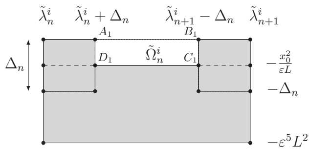
Figure 7.2: Resonance free region as \Delta_n \geq \frac{x_0^2}{\varepsilon L}
