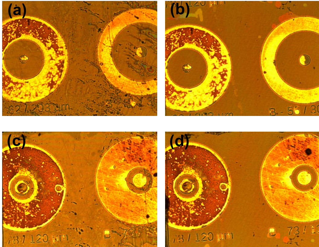
Figure D.7: (a)–(b). Surface treatment by HCl:H 2 O before and after lithography respectively, (c)–(d). Surface treatment by KOH before and after lithography respectively.
