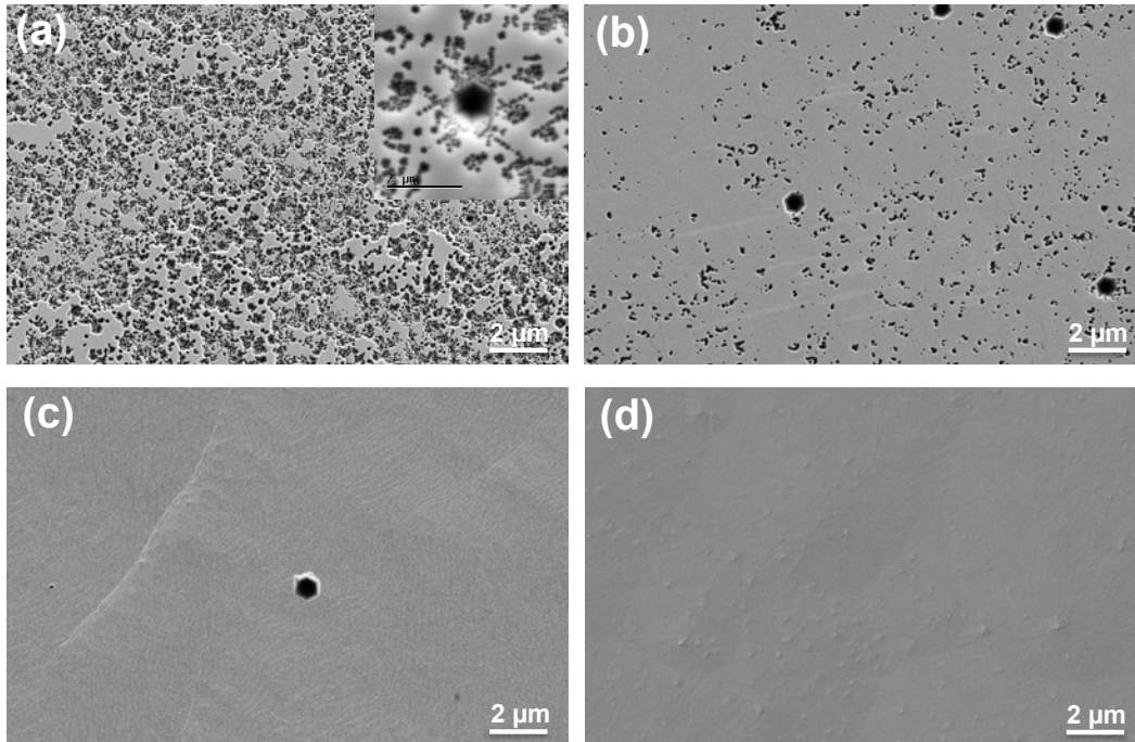
Figure 3.3: SEM image of the top surface of the different InGaN PV structures with p-GaN grown at, (a) 800°C, (b) 850°C, (c) 900°C, (d) 1000°C.
