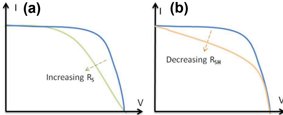
Figure B.7: Effect of (a). increasing the series resistance while keeping R_{sh}=\infty , (b). decreasing the shunt resistance while keeping R_s = 0 . In each case the effect of parasitic resistances is to reduce the FF
