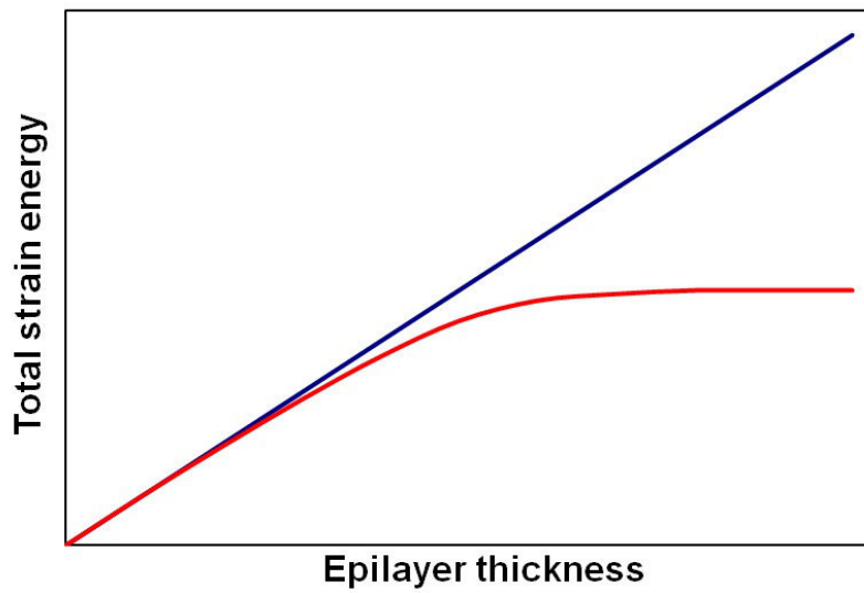
Figure C.4: Total strain energy stored in the system versus the thickness of the epilayer grown by (a) conventional growth and (b) nano selective area growth [223].
