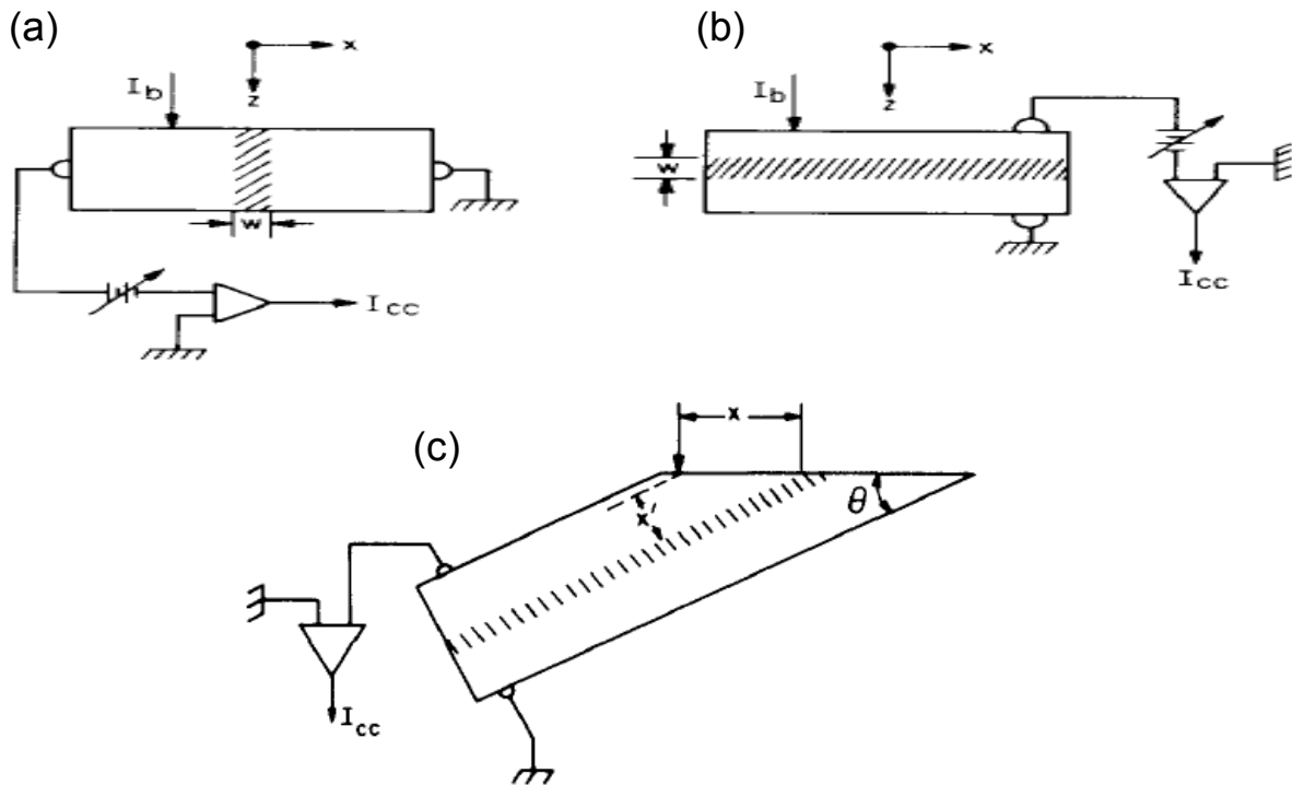
Figure E.1: Different EBIC geometries where the depletion region is denoted by cross hatching, (a) crosssectional geometry, (b) Planar geometry and (c) beveled geometry [278].
