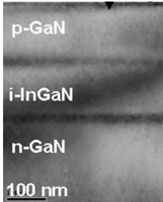
Figure 2.7: Cross-sectional TEM image obtained from GaN/InGaN/GaN epilayers. The dark background within the up and down interfaces of InGaN/GaN exhibits a strain contrast due to the stored misfit strain energy [56].
