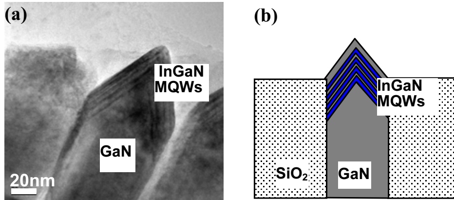
Figure 2.29: (a) Cross-sectional transmission electron microscopy (TEM) image of a single GaN nanorod with 4 periods of InGaN/GaN MQWs, showing high crystal quality with low defect density, resulting in an improvement in internal quantum efficiency [117].
