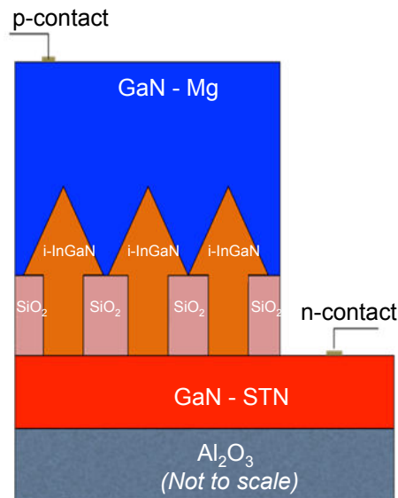
Figure 2.30: Schematic of bulk InGaN nano-structure approach proposed by our team.
