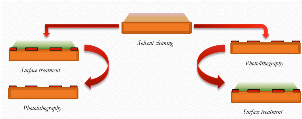
Figure D.5: Surface treatment processes used in this thesis.
