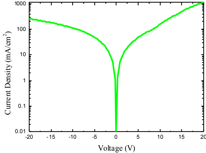
Figure 5.13: Current density versus voltage characteristic of the \text{In}_{0.09}\text{Ga}_{0.91}\text{N}/\text{GaN} nano-structure solar cell under dark conditions.
