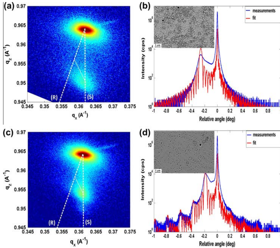
Figure 2.24: (10.5) reciprocal space maps and (00.2) \omega - 2\theta scans of the (a and b) bulk structure and (c and d) semibulk structure. The isocomposition lines connect the theoretical lines of fully strained (S) and fully relaxed (R) InGaN. The inset on (b and d) shows SEM images of the bulk InGaN and semibulk InGaN surfaces, respectively [112].
