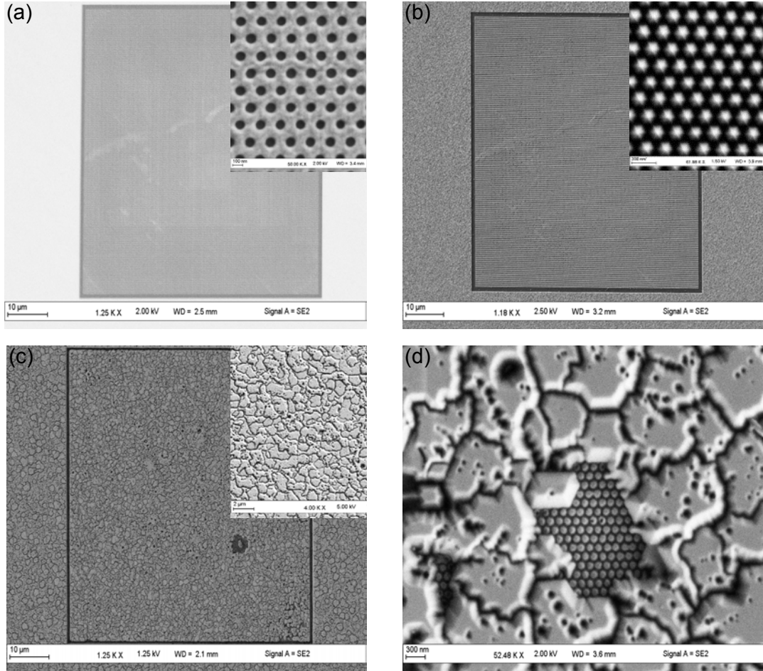
Figure 5.8: InGaN nano-structure PV cell surface morphology, (a) before InGaN growth, (b) after InGaN growth, (c) after p-GaN growth and (d) High magnification SEM image of the p-GaN.
