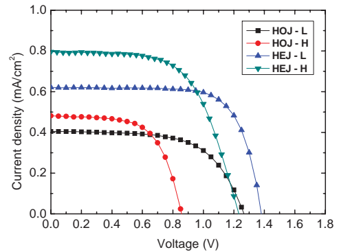
Figure 2.21: J - V characteristics for InGaN PIN homojunction (HOJ) and heterojunction (HEJ) solar cells [106].
