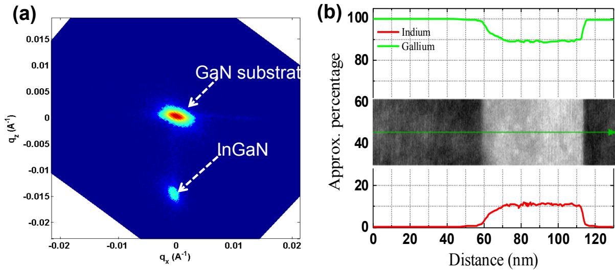
Figure 3.4: (a) (11-24) RSM, indicating GaN substrate diffraction spot and InGaN diffraction spot, (b) EDX measurements showing average In concentration of 12%.
