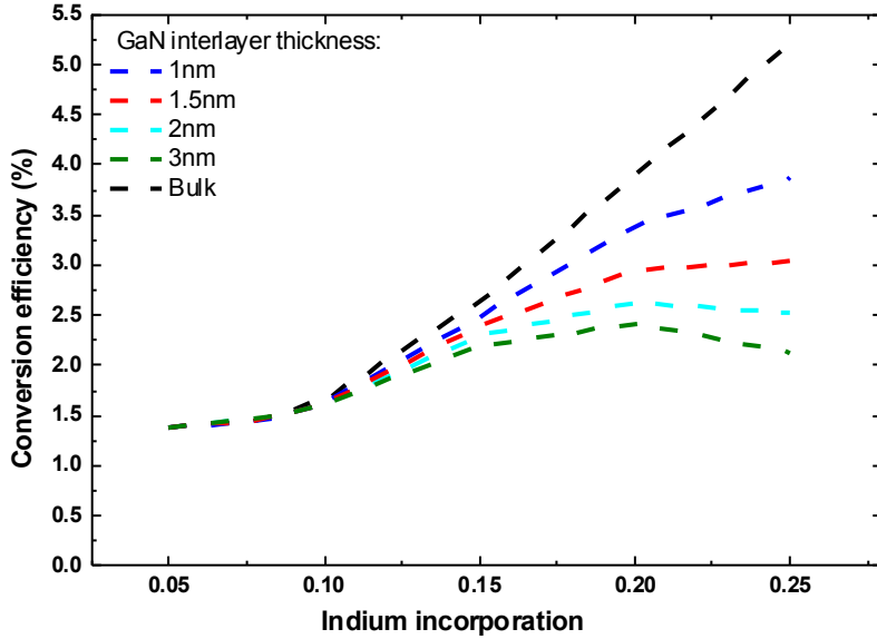
Figure 4.2: Simulated power conversion efficiency dependence on indium incorporation for bulk and semibulk structures with different NID-GaN interlayer thicknesses for semibulk InGaN PV structure.
