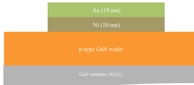
Figure D.10: A typical metallization scheme consisting of Ni(10nm)/Au(10nm).
