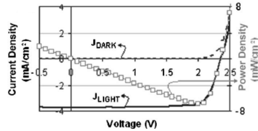
Figure 2.6: Current-voltage characteristic obtained by Jani et al. [51] showing V_{oc} of 2,4 V, a J_{sc} 3,7 \text{mA}/\text{cm}^2 and fill factor 78% under concentrated UV light source.
