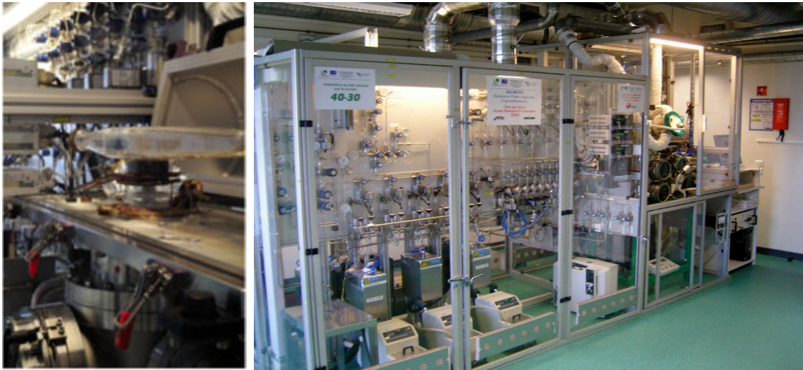
Figure C.2: The reaction chamber (left) and the gas panel of the MOVPE reactor (right) at UMI Georgia Tech Lorraine.
