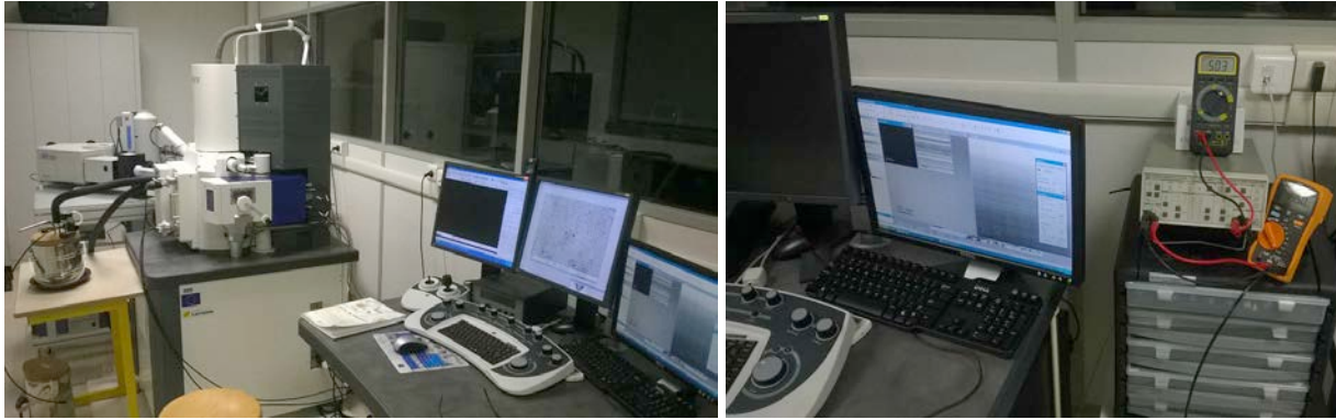
Figure E.3: EBIC setup used for the measurements in this thesis.
