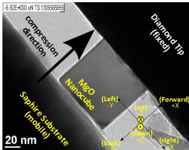
Figure 46: MgO nanocube ready to be compressed in situ TEM. Arrows show possible movements of the sample
