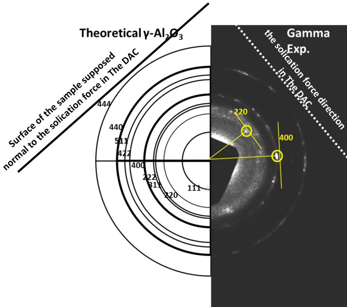
Figure 98: Theoretical Debye Scherrer pattern of \gamma - \text{Al}_2\text{O}_3 compared with the experimental Debye Scherrer pattern of the sample compacted at 20 GPa.
