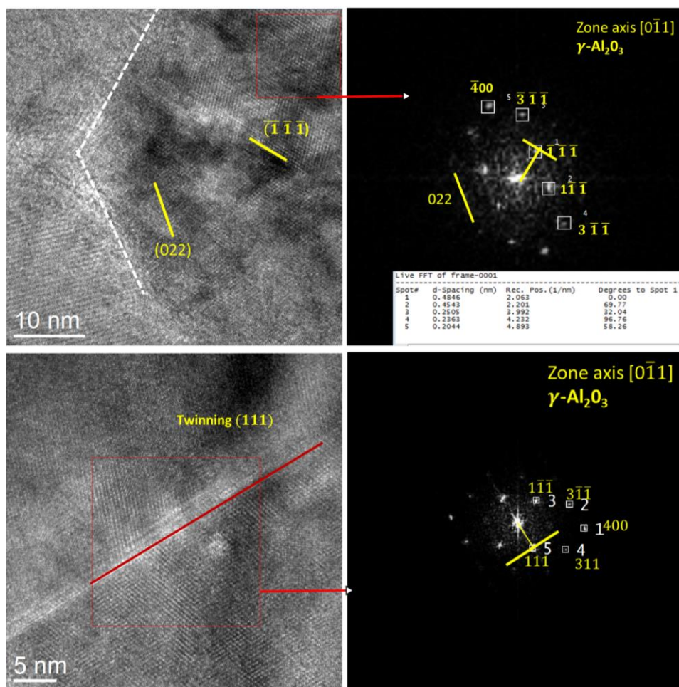
Figure 101: HRTEM images of nanoparticles showing twins. FT indexations reveal that these twins occur in \{111\} planes.
