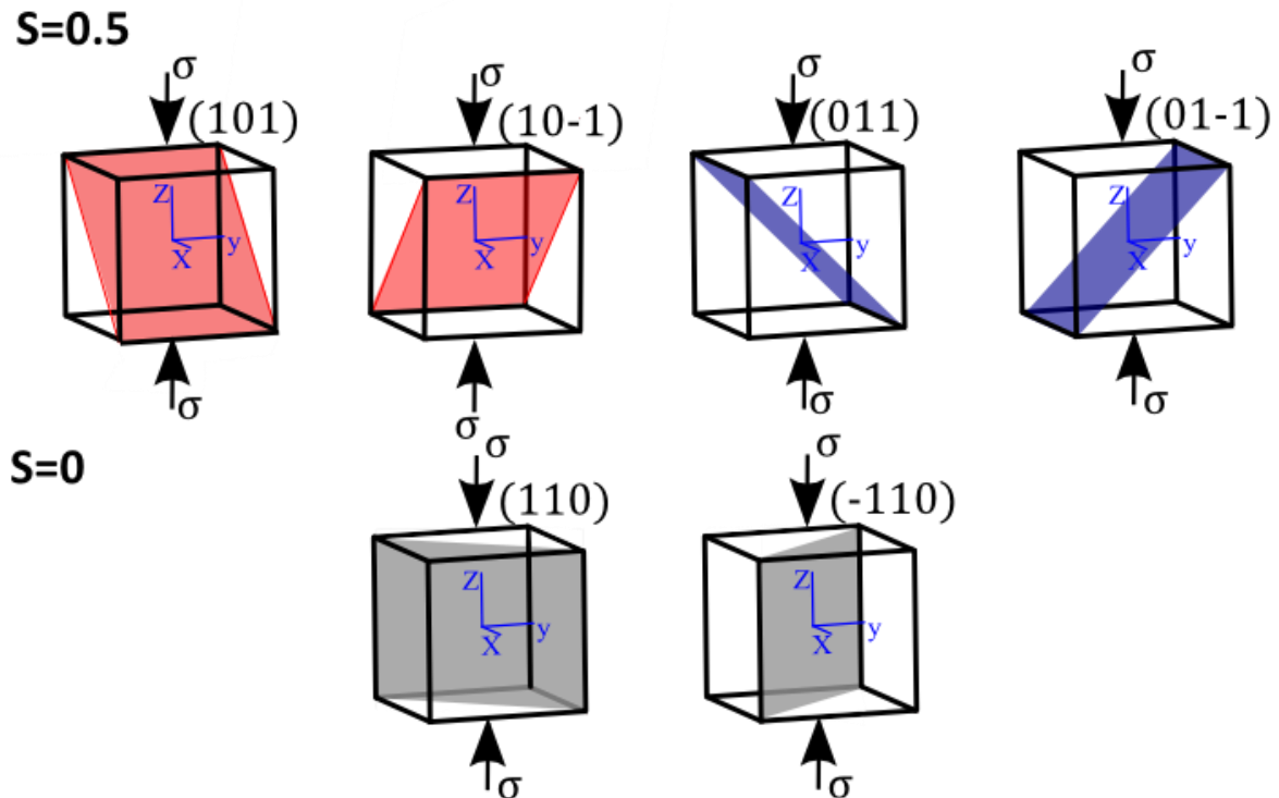
Figure 28: 6 systems of the soft slip system type \frac{1}{2}\langle 110 \rangle \{110\} . Solcitation direction is [001] (Z direction). 4 slip planes ( (101) , (10\bar{1}) , (011) & (01\bar{1}) ) over 6 are active in this case, with a Schmid factor 0.5. The two other systems, with (110) and (\bar{1}10) planes have a Schmid factor = 0.
