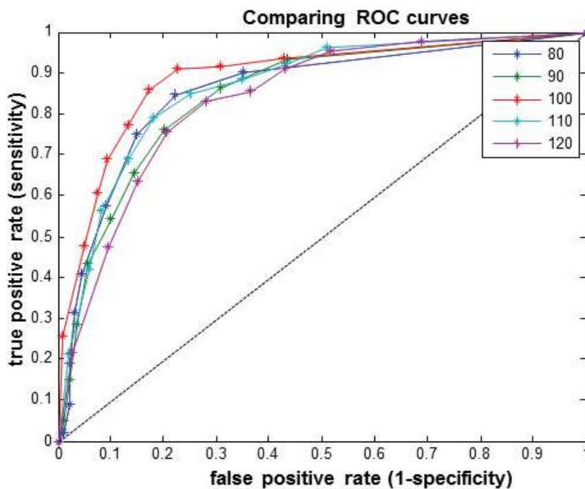
Figure 4. 5: Cross Validation results
