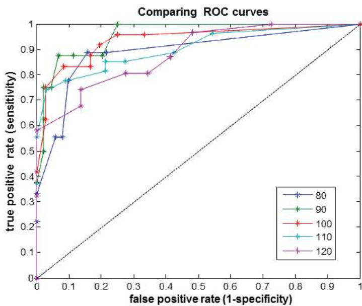
Figure 4. 3: ROC comparison through the variation of DET_{thresh} and BG_{thresh}
