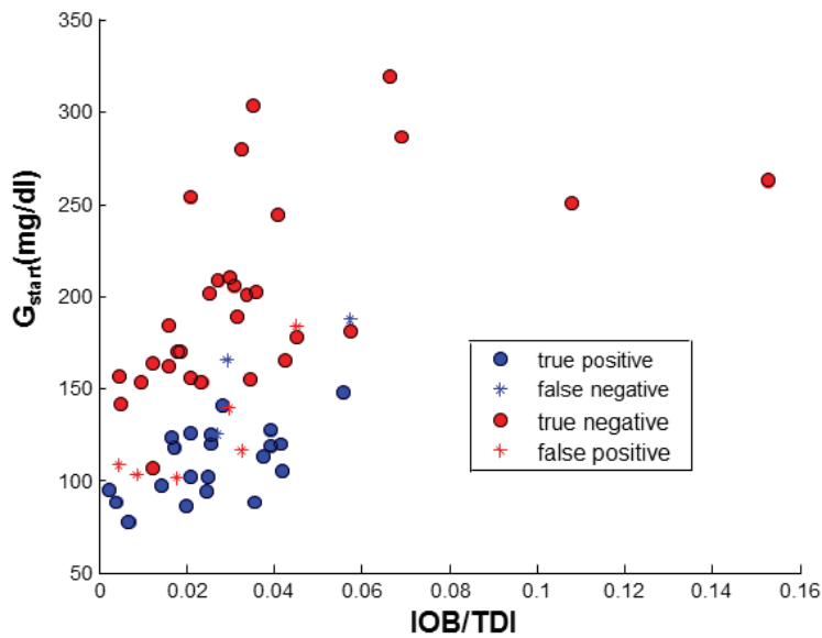
Figure 4. 2: Classification results on training data
