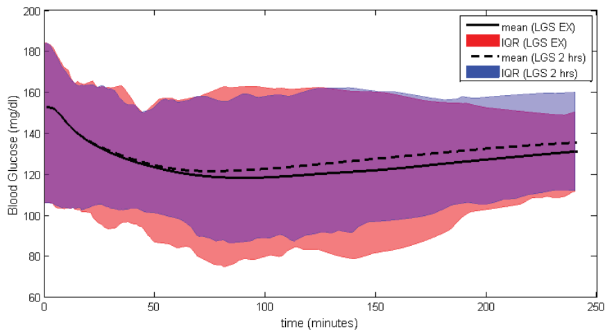
Figure 5. 7: Comparison of S2-a and S2-c
