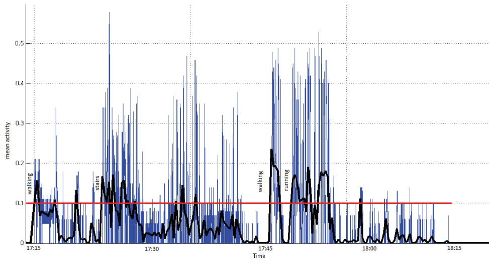
Figure 5.3: Mean activity over time. (the red line is the detection threshold, the bold dark line is the average)
