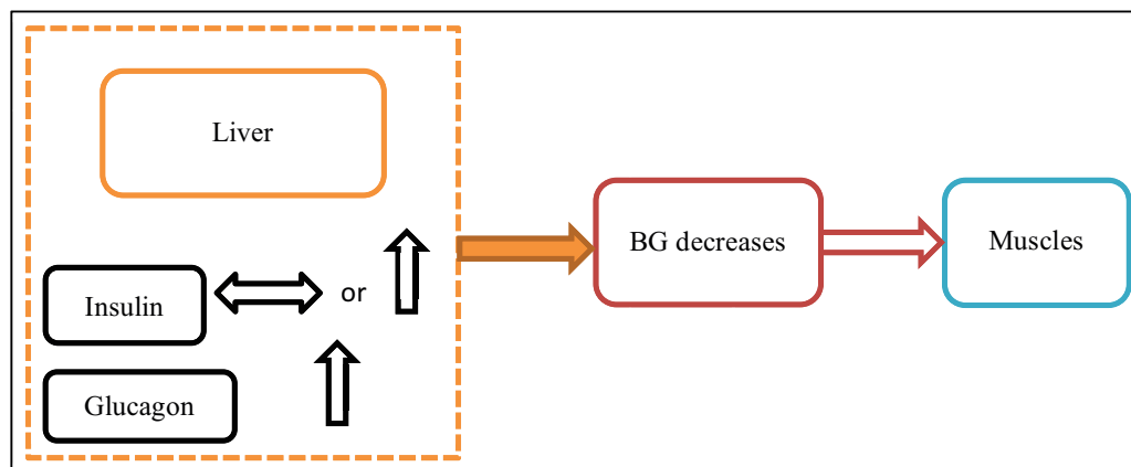
Figure 2. 4: Aerobic exercise physiology in T1DM
