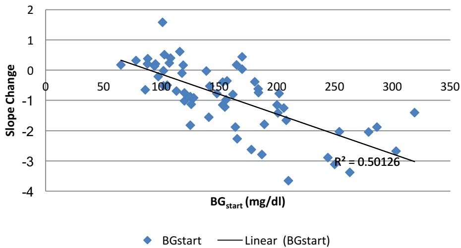
Figure 3. 2. – Correlation between the slope change of blood glucose levels at exercise and the blood glucose levels at the beginning of exercise in patients with type 1 diabetes.
