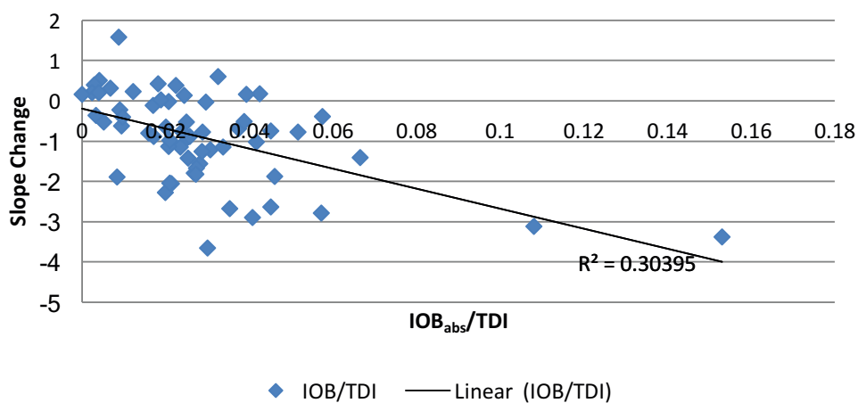
Figure 3. 3. Correlation between the slope change of blood glucose levels at exercise and the body exposure to insulin, expressed as IOB_{abs}/TDI , at the beginning of exercise in patients with type 1 diabetes.
