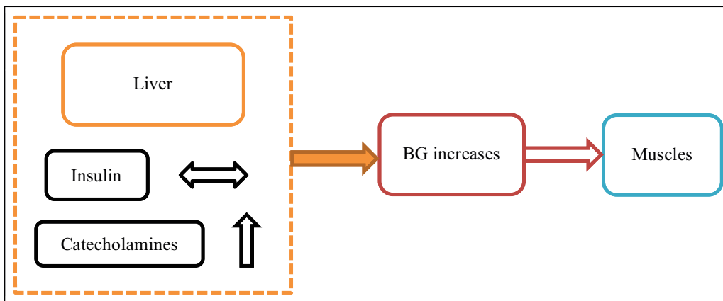
Figure 2. 5: Anaerobic exercise physiology in T1DM
