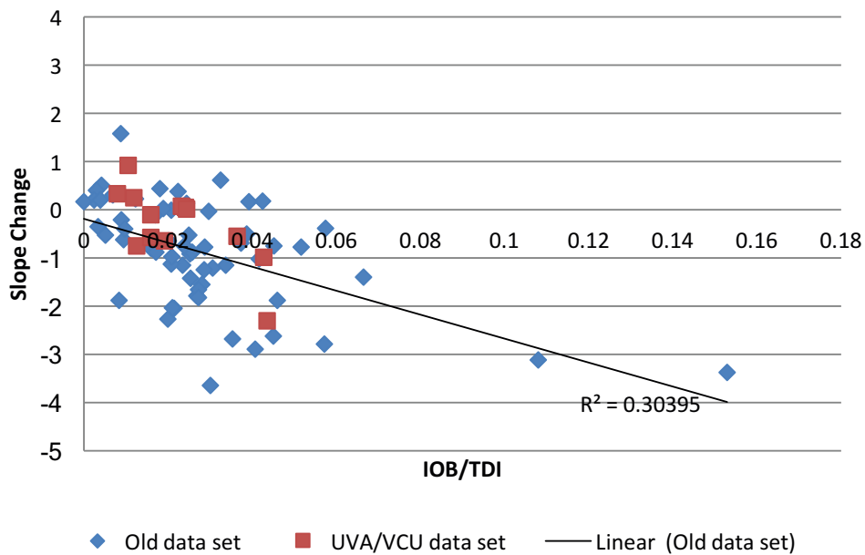
Figure 3. 6. Observation of the UVA/VCU ongoing trial data-Correlation between the slope change and IOB/TDI
