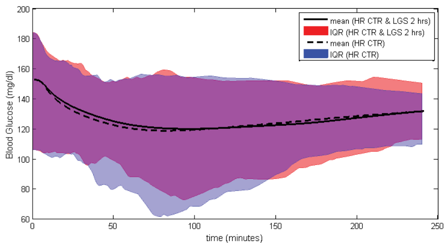
Figure 5. 19: Comparison of the combination of S2-c/HR CTR and HR CTR
