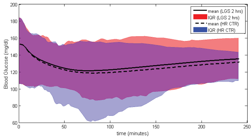
Figure 5. 15: Comparison of S2-c and S1
