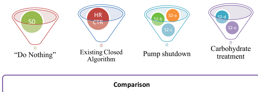
Figure 5. 5: Actions' strategies to prevent exercise-induced hypoglycemia
