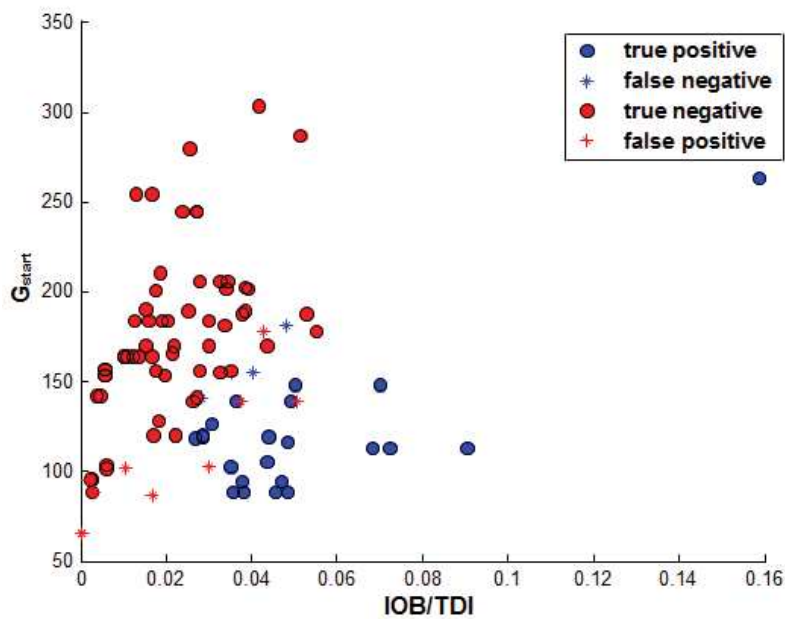
Figure 4. 6: Simulation results
