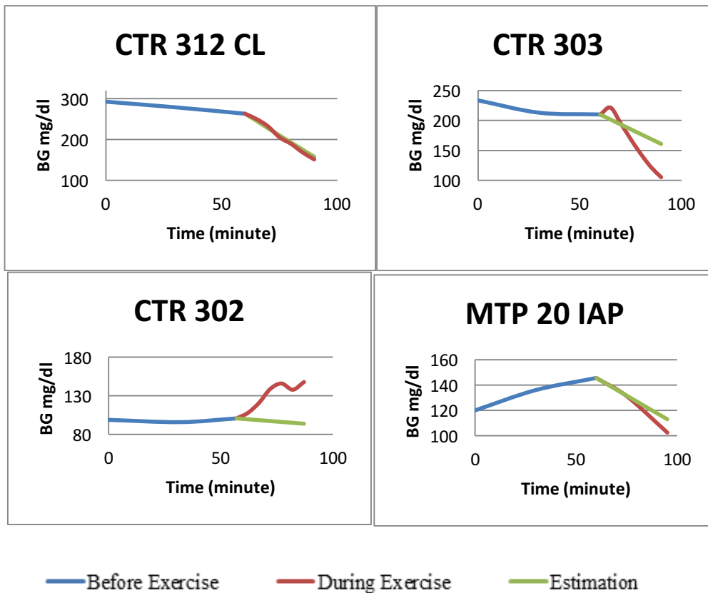
Figure 3. 5. Prediction of blood glucose based on the multiple linear regression model
