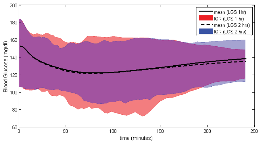
Figure 5. 8: Comparison of S2-b and S2-c
