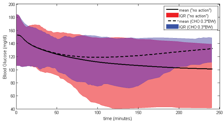
Figure 5. 13: Comparison of S0 and S2-e
