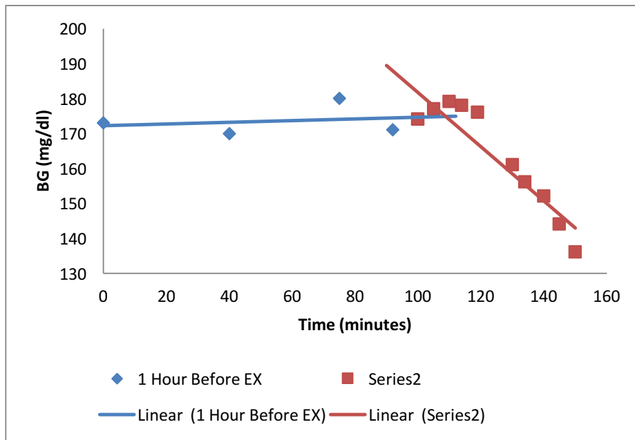
Figure 3. 1. Slope change calculation
