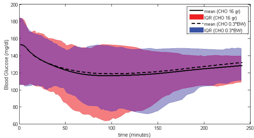
Figure 5. 11: Comparison of S2-d and S2-e
