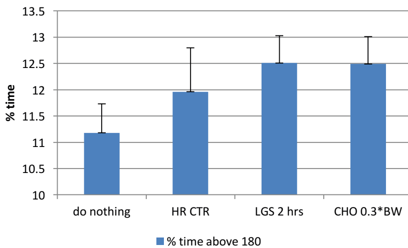
Figure 5. 18: Percentage time above 180 mg/dl
