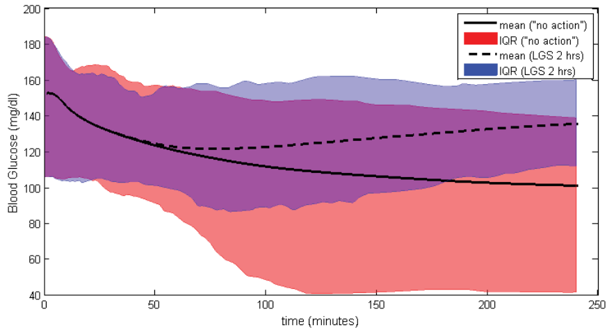
Figure 5. 12: Comparison of S0 and SS2-c
