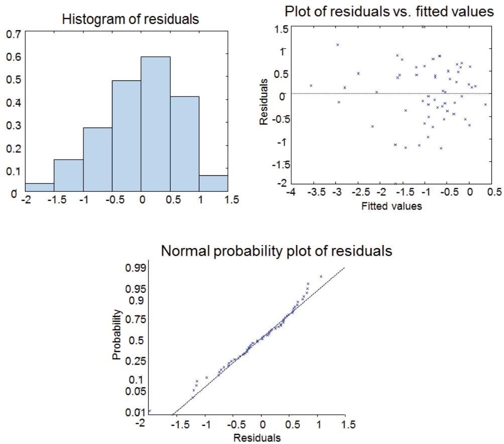
Figure 3.4. Model residuals
