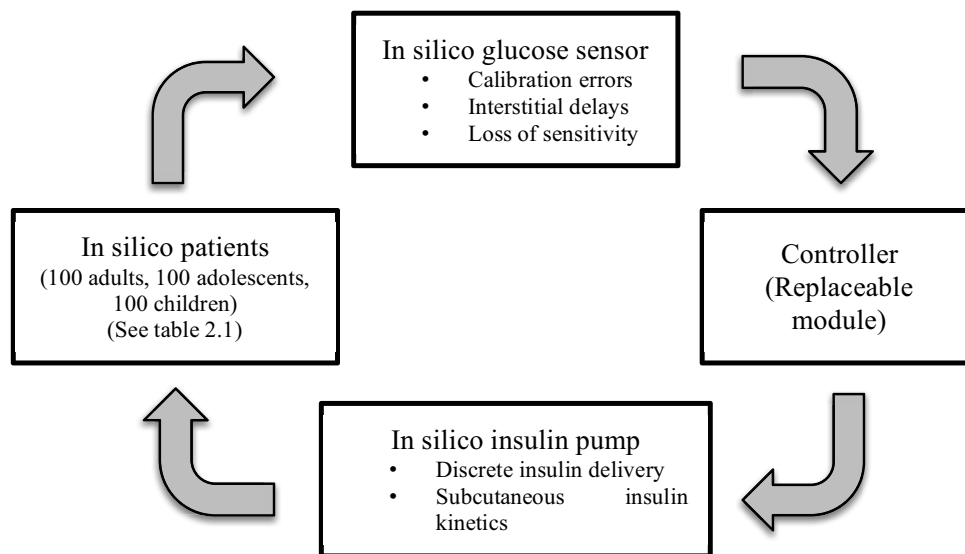
Figure 2. 2: Principal components of T1DM simulator
