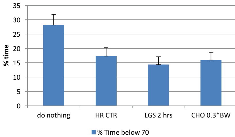
Figure 5. 17: percentage time below 70
