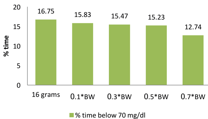
Figure 5. 9: Comparison of the percentage time below 70 mg/dl for different CHO treatment values as a function of the BW and the fixed value of 16 grams
