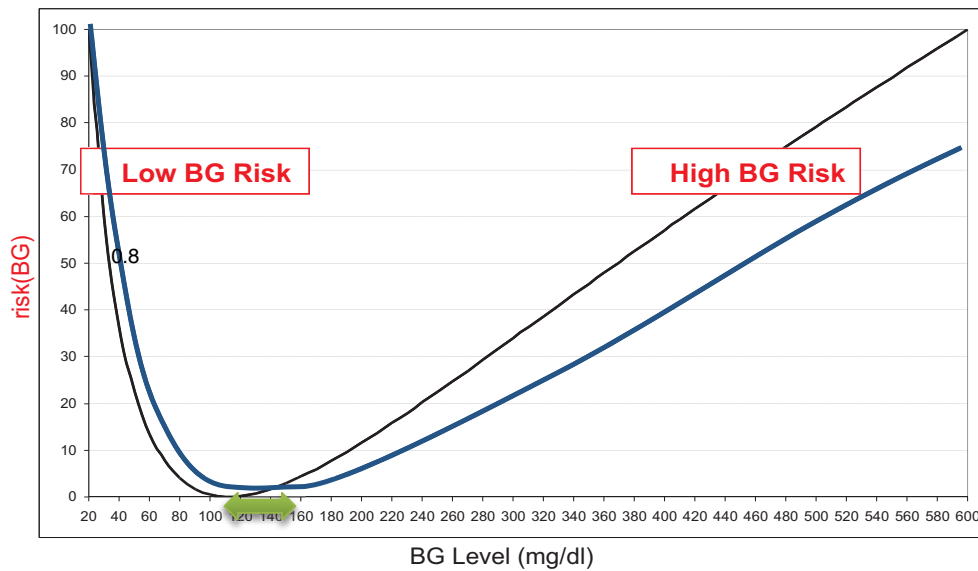
Figure 5. 4: The risk function in the original BG scale: original risk function in black, shifted exercise-induced risk function in blue
