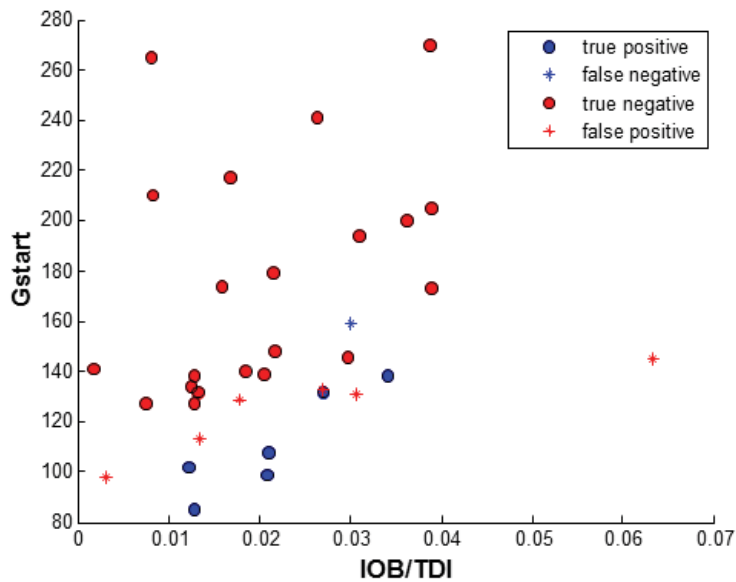
Figure 4. 4: Classification results on testing data set
