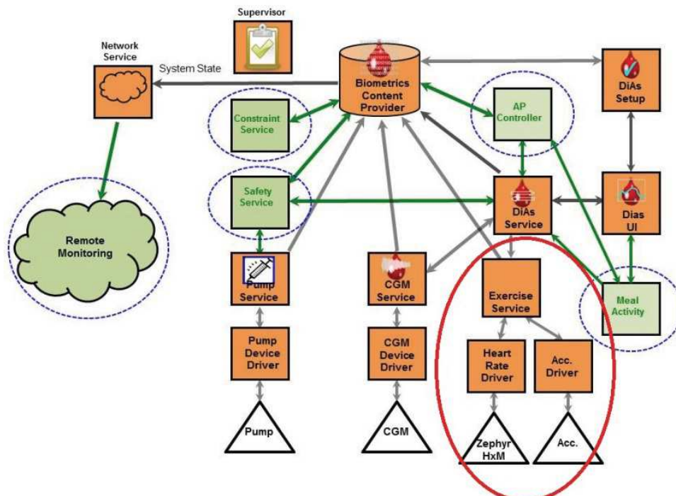
Figure 5. 2: DiAs architecture
