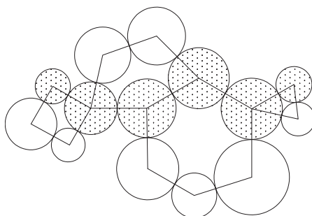
FIGURE 4.16: Force-chain (particles marked with dotted pattern) with attached grain-loops
