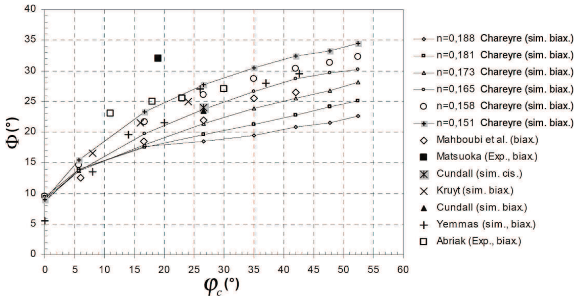
FIGURE 2.6: Macroscopic friction angle in terms of microscopic friction angle, results from Mahboubi et al. [1996] and Chareyre [2003] , assembled by Sibille [2006a] , with n is the porosity of the specimen
