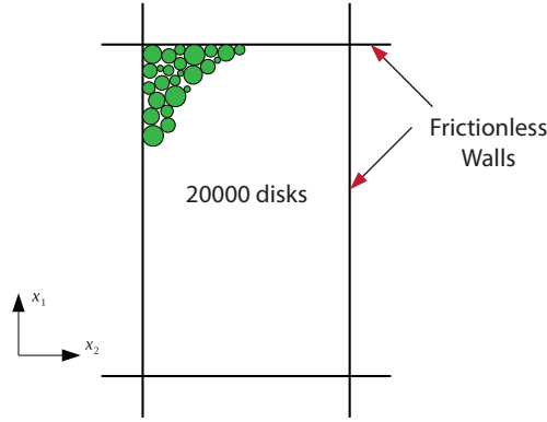
FIGURE 4.1: The 2D model in YADE
