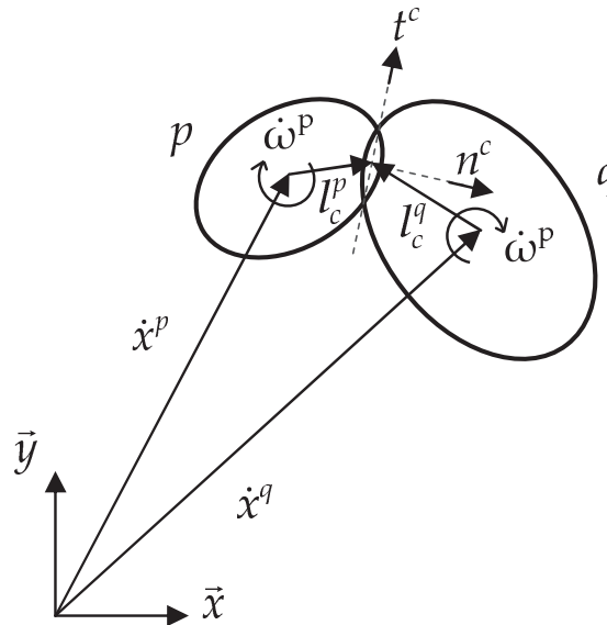
FIGURE 2.2: Positions of two particles in contact ( Hadda et al. [2013] )
