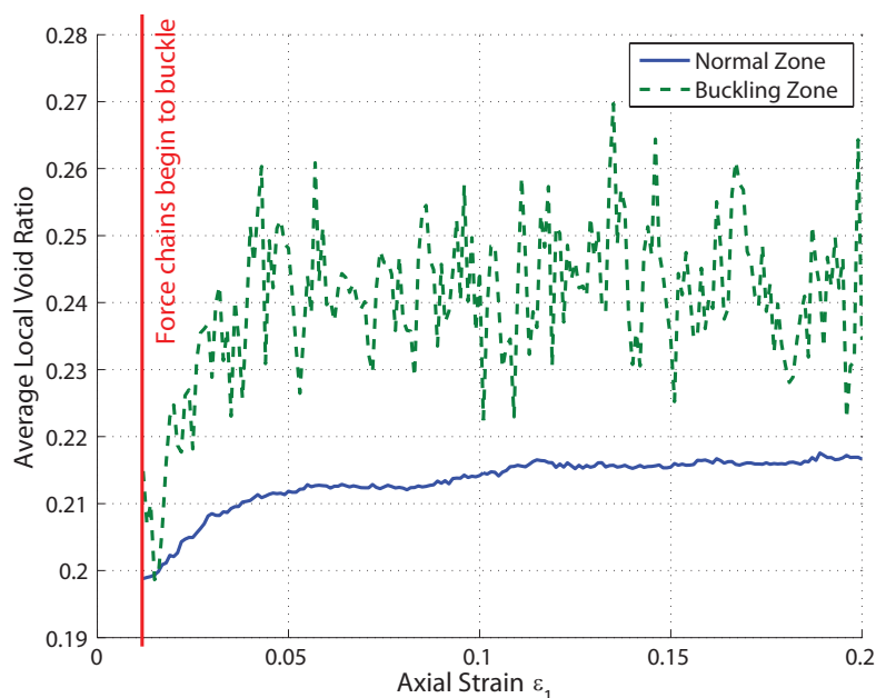
FIGURE 4.25: Comparison of the local void ratio between the buckling zone and non-buckling zone
