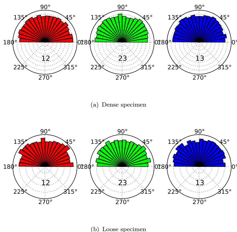
FIGURE 2.13: Isotropy of the distribution of contact orientations of the specimens: (a) dense, (b) loose in three planes “12”, “23” and “13” (See Figure 2.5 for the definition of the axis 1, 2 and 3)
