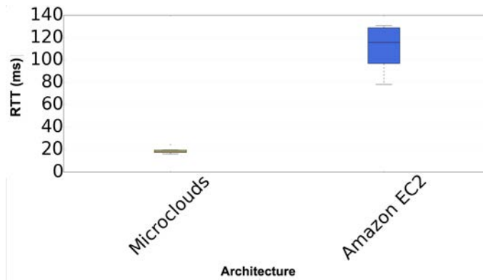
Figure 5.3: Microclouds vs Amazon EC2 RTT
