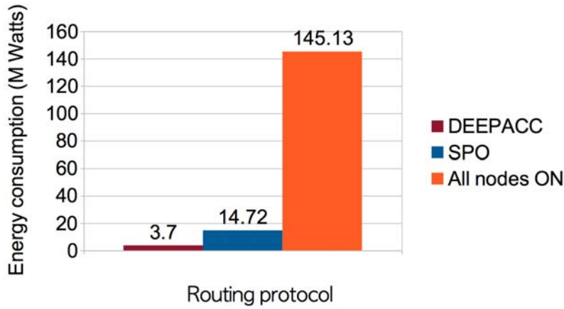
Figure 4.5: Energy consumption of DEEPACC when considering two clients close to each other
