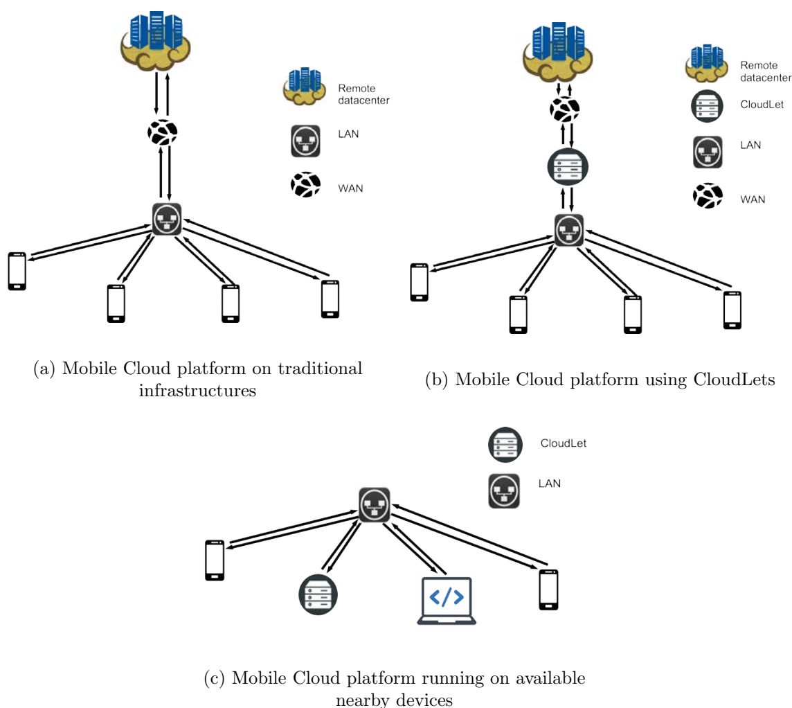
Figure 2.6: P2P schemas
