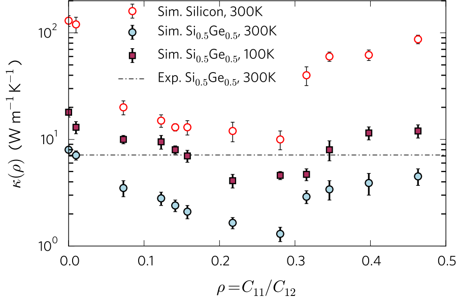
Figure 5.2: Thermal conductivity \kappa of bulk Si at 300 K (red open circles) and \text{Si}_{0.5}\text{Ge}_{0.5} alloy at 100 K (dark red squares) and at 300 K (blue solid circles) versus the relative strength of the second phonon path \rho . For the \text{Si}_{0.5}\text{Ge}_{0.5} alloy, the thermal conductivities were obtained by averaging five different random atomic distributions. Our first-principle calculations show that natural SiGe alloys has \rho \approx 5.7\% .
