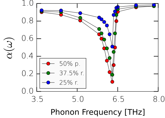
Figure 3.6: Transmission coefficient \alpha(\omega) for longitudinal phonons through the planar defect in a Si crystal, which contains randomly (r) distributed embedded Ge atoms with f_d = 37.5\% and 25\% , compared with \alpha(\omega) through the planar defect, which contains periodically (p) distributed embedded Ge atoms with f_d = 50\% . The computed \alpha(\omega) was averaged over different random distributions
