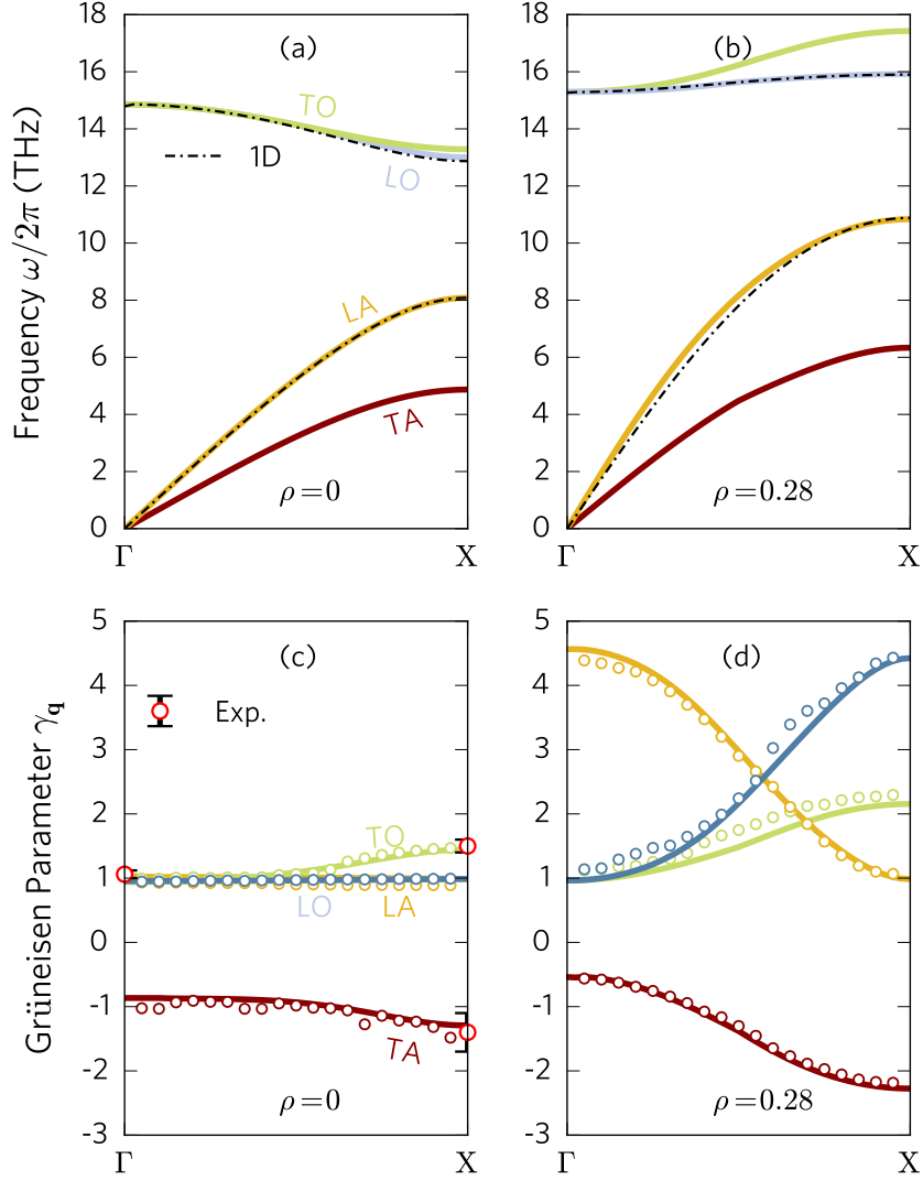
Figure 5.4: Phonon band structure \omega - \mathbf{k} in the \langle 001 \rangle direction of a \text{Si}_{0.5}\text{Ge}_{0.5} crystal for different relative strengths of the second phonon path: (a) \rho = 0 (b) \rho = 0.28 corresponding to the minimum thermal conductivity. The letters “T, L, A, O” represent transverse, longitudinal, acoustic and optical modes, respectively. For example, “TA” denotes the transverse acoustic phonon branch. Black dotted-dashed curves are phonon dispersion of a diatomic lattice of alternating Si and Ge atoms, where only longitudinal modes are present. Mode-dependent Grüneisen parameters \gamma_{\mathbf{q}} of the same \text{Si}_{0.5}\text{Ge}_{0.5} crystal for (c) \rho = 0 (d) \rho = 0.28 . Open circles and lines from the two different methods. Experimentally measured Grüneisen parameters on the Brillouin zone edge and center are for comparison.
