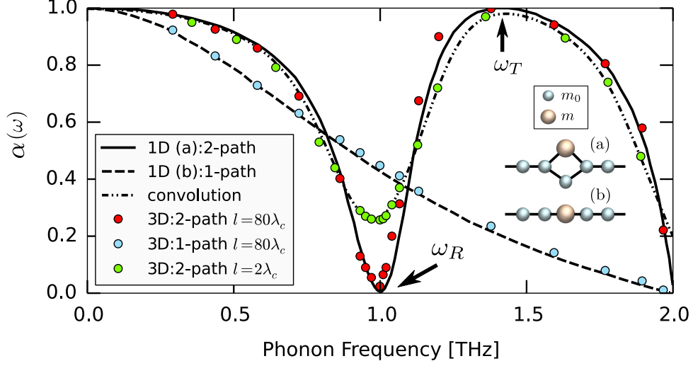
Figure 3.2: Spectra of the energy transmission coefficient \alpha(\omega, l) predicted by equivalent quasi-1D model (solid and dashed lines) and by MD simulations (symbols) for a 3D Ar metamaterial with defect crystal plane containing heavy isotope impurities, with mass m = 3m_0 . Dashed-dotted line is the convolution Eq. (3.2) of the plane-wave transmission coefficient \alpha(\omega) from Eq. (3.1) with a Gaussian wave packet in frequency domain with l = 2\lambda_c . Red and blue symbols present transmission of the wave packet with l = 20\lambda_c through the two paths and through one path in the Ar metamaterial with planar defect, respectively; green symbols present transmission of the wave packet with l = 2\lambda_c through the two paths. (Inset) Two possible quasi-1D lattice models describing phonon propagation through the lattice region containing the local defect: (a) phonons can propagate through the defect and host atoms bonds; (b) phonons can propagate only through the defect atom bonds. Black sticks between the atoms present atom bonds. In the case of Ar lattice, the coefficients in Eq. (3.1) are \omega_R = 1.0 , \omega_T = 1.4 , \omega_{max} = 2.0 and C = 0.25 . The quasi-1D model (a) is equivalent to a 2D crystal plane partially filled with periodically alternating isotopes with different masses, with f_d = 50\% , in a 3D Ar lattice. The 1D model (b) is equivalent to a 2D crystal plane completely filled with heavy isotopes, with f_d = 100\% , in a 3D Ar lattice.
