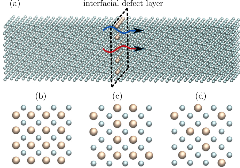
Figure 3.1: (a) Interference Phonon Metamirror: 3D face-centered cubic lattice containing an internal (001) crystal plane in which an impurity-atom array is embedded. The brown atoms are the defect atoms and the green ones are the atoms of the host lattice. The red and blue curves refer to the phonon paths through the impurity atom bonds and through the host atom bonds, respectively. The presence of the two possible phonon paths can result in the two-path destructive-interference transmission antiresonance. (b) Periodic distribution of defect atoms with filling fraction f_d = 50\% . Randomly distributed defect atoms with (c) f_d = 37.5\% and (d) f_d = 25\%
