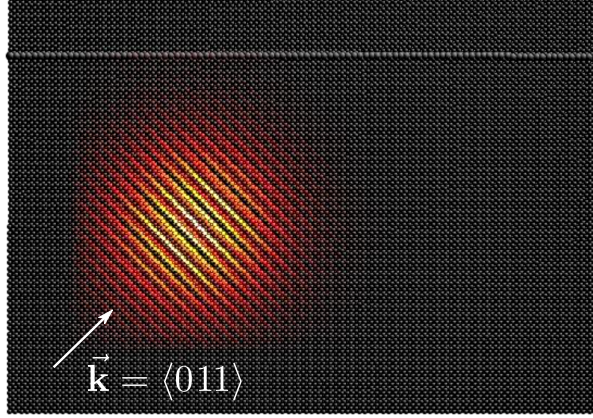
Figure 2.3: Oblique phonon wave-packet of the same mode as in Fig. 2.1 in the \langle 011 \rangle direction.
