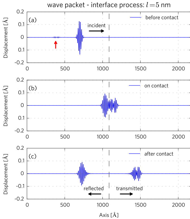
Figure 2.2: Elastic scattering of a phonon wave-packet at an internal interface of bulk Stillinger-Weber silicon. The wave-packet corresponds to the same phonon mode as in Fig. 2.1 except that the coherence length is much shorter, l = 5 nm. The red arrow denotes the back scattering of the WP.
