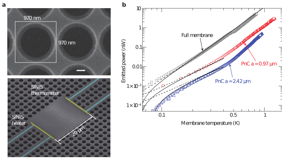
Figure 1.3: Thermal phonon engineering in porous films. (a) Top: Scanning electron microscopy (SEM) image of a periodic porous thin-film made from a square array of air cylinders with periodicity a_0 = 970 nm on a silicon nitride matrix [Zen et al. (2014)]. Scale bar: 200 nm. Bottom: SEM image showing the Al (blue) and Cu (yellow) wires that form the heater and thermometer at the centre of the periodic porous film sample with a_0 = 2.42 μm. SINIS: superconductor/insulator/normal metal/insulator/superconductor. (b) Emitted thermal power measured as a function of temperature. Phononic crystal (PnC) samples with a_0 = 0.97 μm and a_0 = 2.42 μm are shown. Uniform (unperforated) film is shown with grey squares. Theoretical calculations with and without back radiation from the substrate are shown by solid and dashed lines, respectively.
