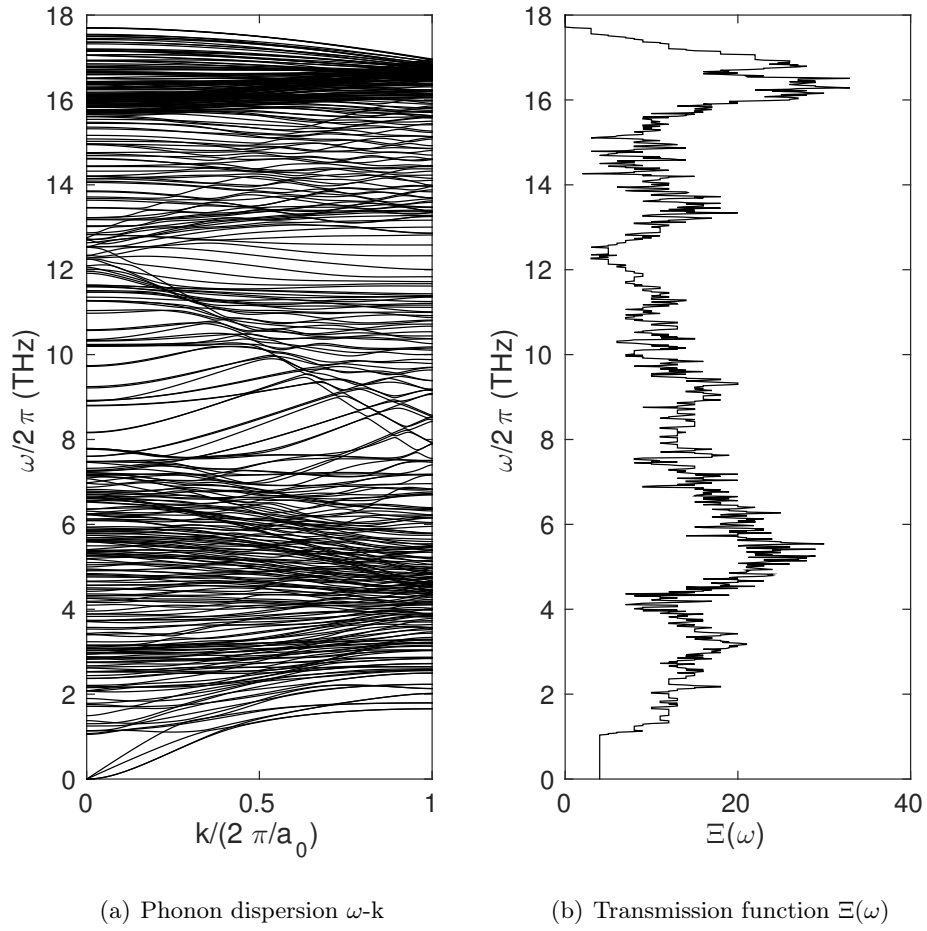
Figure 2.4: Phonon dispersion relation and transmission function \Xi(\omega) along the axial direction of a \langle 001 \rangle Stillinger-Weber silicon nanowire with a cross section of 21.72 \times 21.72 \text{ nm}^2 .
