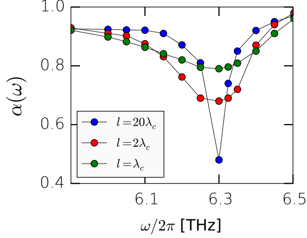
Figure 3.8: Broadening of the antiresonance dip in the energy transmission coefficient \alpha(\omega, l) in the limit of small filling fraction f_d = 5\% for the wave packets with short coherence lengths ( l = \lambda_c and l = 2\lambda_c , green and red circles), in comparison with that for an almost plane-wave wave packet ( l = 20\lambda_c , blue circles)
