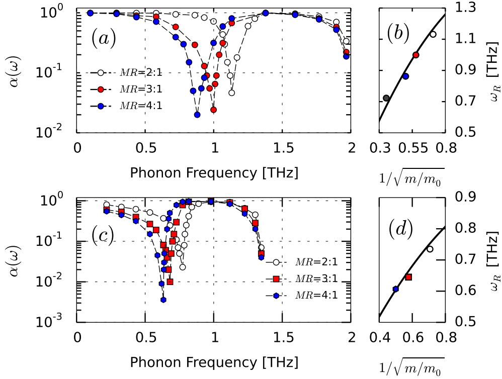
Figure 3.3: (a) and (c): Spectra of phonon transmission coefficient \alpha(\omega) of longitudinal (a) and transverse (c) acoustic waves through the phononic metamaterial, which consists of 2D crystal plane filled with periodically alternating isotopes with different mass ratio (MR) m/m_0 with f_d = 50\% in a 3D Ar lattice. Dashed lines are the guides to the eye. (b) and (d): Isotopic shift of the two-path phonon interference antiresonance versus the inverse square root of the mass ratio for longitudinal (b) and transverse (d) acoustic waves. Symbols present the resonances predicted by MD simulations for a 3D lattice, solid line shows the analytical prediction of the equivalent quasi-1D lattice model given by Eq. (4)
