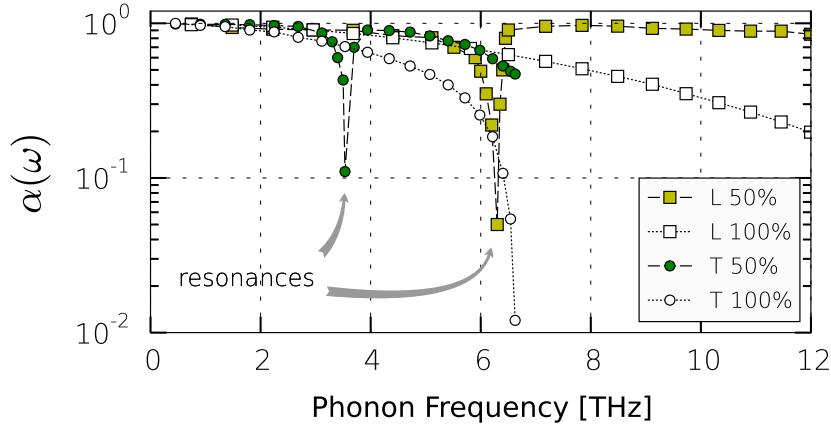
Figure 3.5: Two-path interference phonon antiresonances for transverse and longitudinal phonons across a partially-Ge-filled defect crystal plane (green circles and yellow squares) plotted along with the non-resonant transmission across a completely-Ge-filled defect crystal plane (open squares and circles) in a Si crystal as phononic metamaterial
