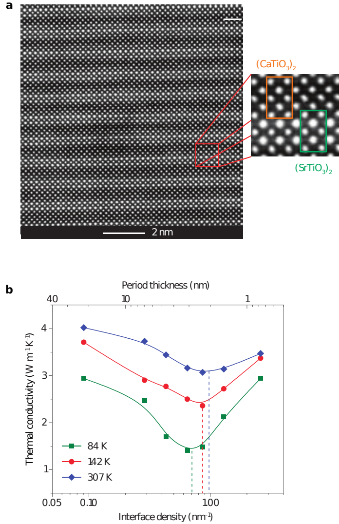
Figure 1.2: Wave-like heat transport and wave interference in \text{SrTiO}_3/\text{CaTiO}_3 superlattices. (a) Transmission electron microscopy (TEM) image of a \text{SrTiO}_3/\text{CaTiO}_3 superlattice with atomically sharp interfaces [Ravichandran et al. (2014)]. (b) Measured thermal conductivity of the superlattice as a function of the period thickness (or interface density) at different temperatures. The solid lines are visual guides. The presence of a local minimum value (vertical dashed lines) for the thermal conductivity reveals wave interference effects for thermal vibrations within the superlattice. Wave effects become stronger as the temperature is decreased.
