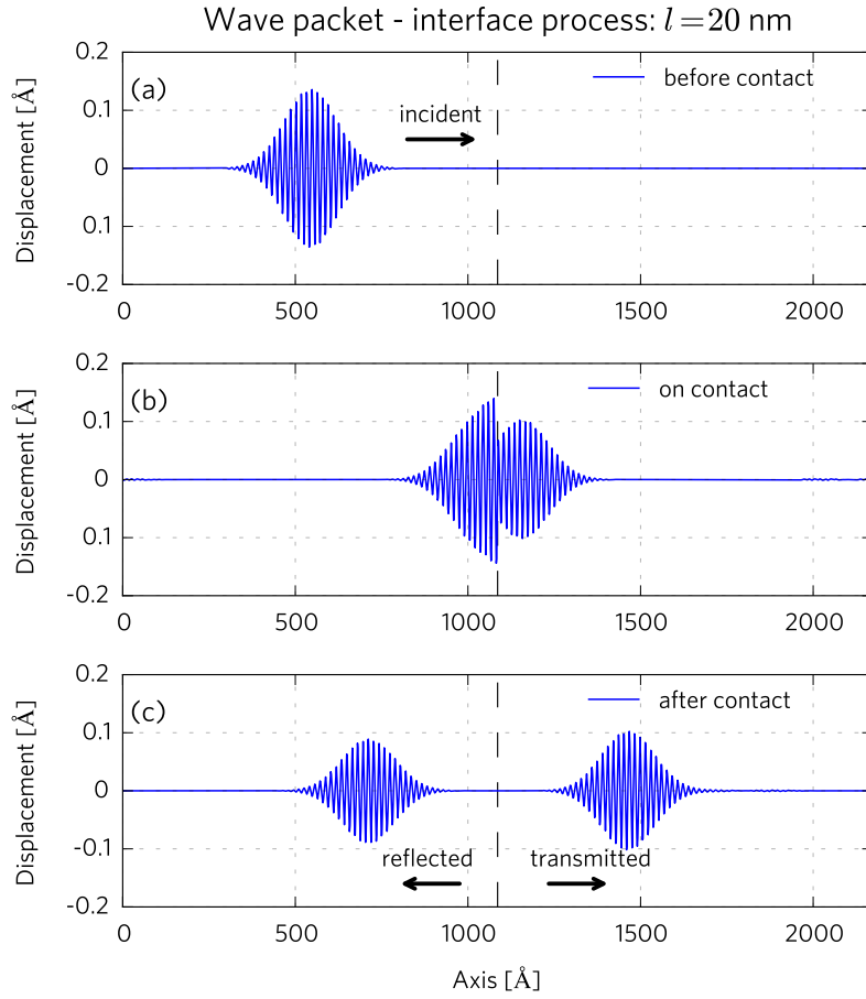
Figure 2.1: Elastic scattering of a phonon wave-packet at an internal \langle 001 \rangle interface of bulk Stillinger-Weber silicon. A longitudinal acoustic phonon WP is generated by following the form in Eq. (2.12) and corresponds to the wave vector \mathbf{k} = \frac{5}{20} \langle 001 \rangle and the frequency \omega = 5.1128 THz. The corresponding central wavelength is \lambda_c = 1.56 nm and the coherence length is l = 20 nm.
