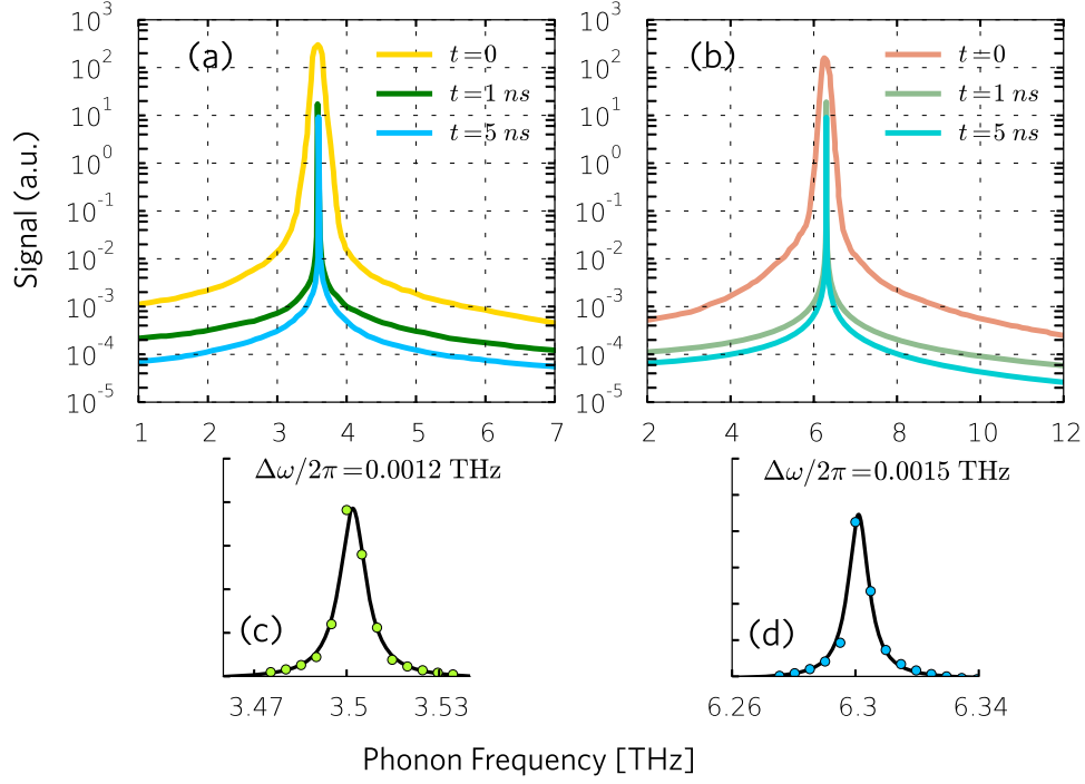
Figure 4.5: Power spectral density of atomic kinetic energy in the capacitor after excitation of the transverse (a) and longitudinal (b) phonon WP as a function of time delay t . The peaks centered at \omega_{1,2} demonstrate a continuous linewidth narrowing as a function of t . At t = 5 ns, the widths narrow down to \Delta\omega_1/2\pi = 1.2 \times 10^{-3} THz and \Delta\omega_2/2\pi = 1.5 \times 10^{-3} THz, which correspond to the cavity Q factors of Q_1 = 2916 and Q_2 = 4208 , respectively. Gaussian fit of the capacitor phonon peaks to measure FWHM \Delta\omega at t = 5 ns for the transverse (c) and longitudinal (d) modes.
