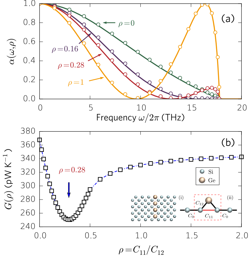
Figure 5.1: (a) Spectral transmission coefficients \alpha(\omega, \rho) predicted by MD simulations (open circles) of a Si host crystal with a single atomic layer of Ge atoms and by Green's Function calculations of an equivalent quasi-1D model (solid lines). Only the longitudinal polarization is shown for the MD prediction. (b) Thermal conductance G(\rho) versus the relative strength of the second nearest-neighbour bond \rho at T = 300 K. Inset (i): host silicon lattice with a single (001) atomic layer of guest Ge atoms. Inset (ii): quasi-1D tight-binding model which incorporates the second nearest-neighbour bonds C_{11} bypassing the nearest-neighbour bonds C_{12} between the host atom with mass m_1 and the guest atom with mass m_2 . The host atoms are coupled through the nearest-neighbour bonds C_0 . Black (red) sticks represent the NN (second NN) bonds. The region inside the red dashed rectangle is the scattering region.
