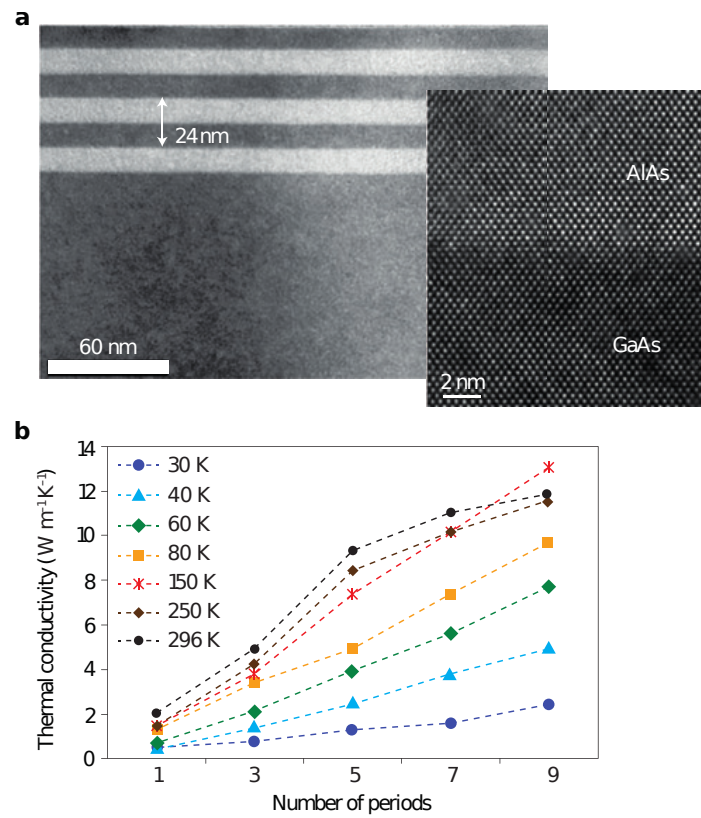
Figure 1.1: Wave-like heat transport and wave interference in GaAs/AlAs superlattices. (a) Transmission electron microscopy (TEM) image of a 3-period GaAs/AlAs superlattice with periodicity a = 24 nm, where the inset shows a high-resolution image of one of the interfaces [Luckyanova et al. (2012)]. (b) Experimental thermal conductivity as a function of the number of periods at different temperatures. Thermal conductivity rises as the number of periods increases, which indicates that phonons cross the interfaces coherently.
