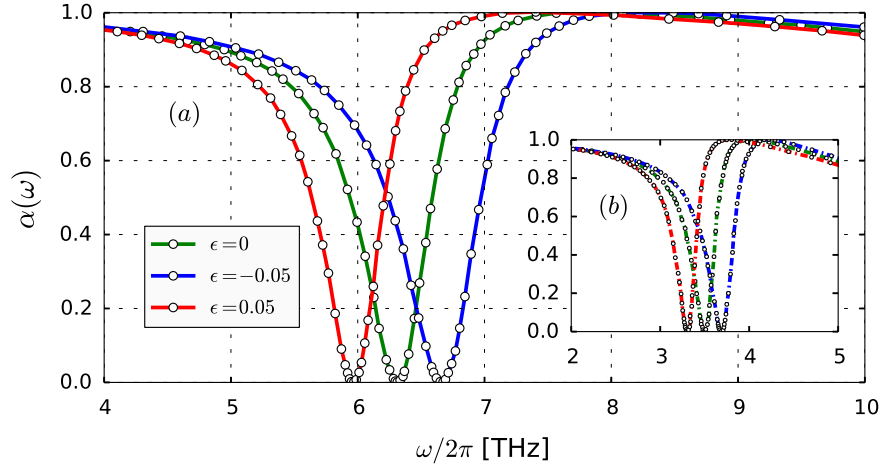
Figure 4.7: Shift of interference antiresonance spectral loci caused by tunable strain \epsilon in the capacitor. Antiresonance frequency shifts for longitudinal (a) and transverse (b) plane waves, normally incident on interference mirror. Interference cavity is exposed to the uniaxial strain \epsilon in the \langle 001 \rangle direction. Negative strain \epsilon < 0 , corresponding to a compression of the cavity, results in a blue shift of mirror’s antiresonance frequencies in accordance with positiveness of the Grüneisen parameter. In a similar manner, positive strain red-shifts antiresonance frequencies.
