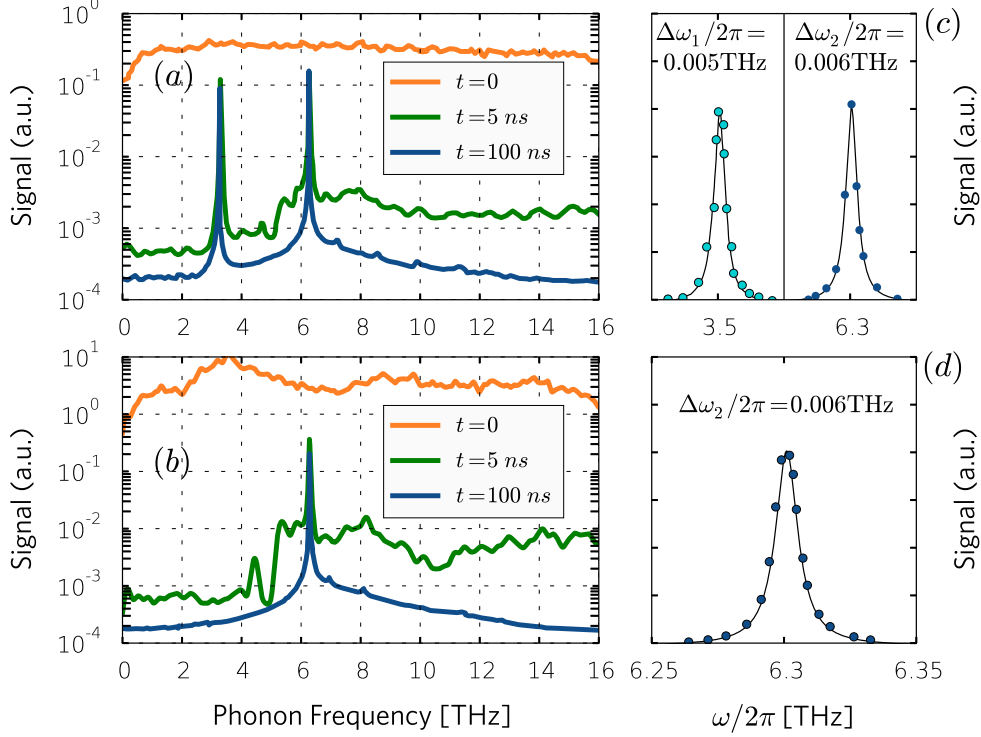
Figure 4.2: Power spectral density of atomic kinetic energy in the nanocapacitor initially thermalized at T = 300K as a function of time delay t after the cooling onset. Nanocapacitor dimensions are L_x^c = L_y^c = 8 nm and L_z^c = 35 nm (a), and L_x^c = L_y^c = 33 nm and L_z^c = 35 nm (b). (c) and (d): Gaussian fit of the capacitor phonon peaks to measure FWHM \Delta\omega at t = 100 ns for the peaks in (a) and (b), respectively.
