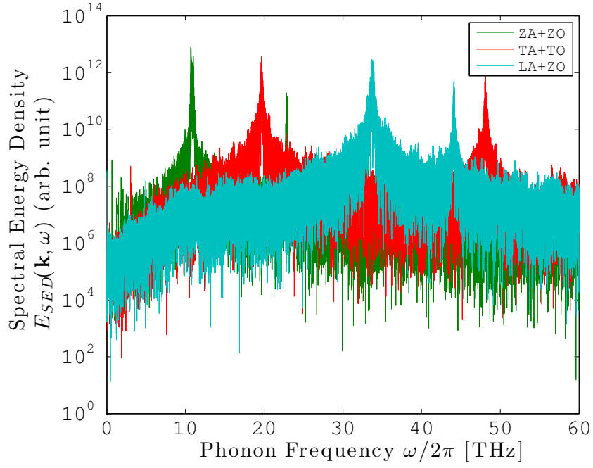
Figure 2.6: Semilogarithmic plot of the spectral energy density function E_{SED}(\mathbf{k}, \omega) along the \Gamma -K direction with \mathbf{k} = \frac{4}{5} \frac{2\pi}{a_0} [100] of a supported graphene sheet. Different colors stand for the corresponding phonon branches.
