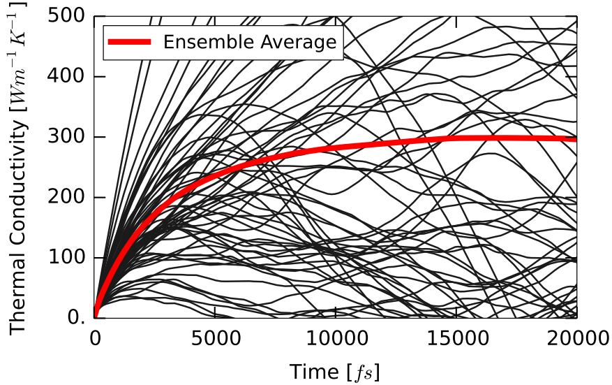
Figure 2.7: Thermal conductivity proportional to the time integrals of the heat flux autocorrelation functions from Eq. (2.57). Black curves are the running integral of a single trajectory and the red curve refers to the ensemble average of different trajectories.
