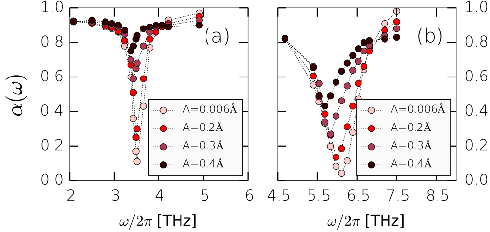
Figure 3.7: Evolution of the interference antiresonance in the phonon transmission coefficient \alpha(\omega) through the partially-Ge-filled, with f_d = 50\% , internal crystal plane in Si lattice versus the increasing wave amplitude for (a) transverse and (b) longitudinal phonons
