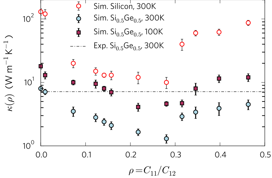
Figure 5.2: Thermal conductivity \kappa of bulk Si at 300 K (red open circles) and \text{Si}_{0.5}\text{Ge}_{0.5} alloy at 100 K (dark red squares) and at 300 K (blue solid circles) versus the relative strength of the second phonon path \rho . For the \text{Si}_{0.5}\text{Ge}_{0.5} alloy, the thermal conductivities were obtained by averaging five different random atomic distributions. Our first-principle calculations show that natural SiGe alloys has \rho \approx 5.7\% .
