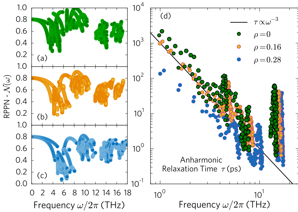
Figure 5.5: Relative Phonon Participation Number (RPPN) \mathcal{E}_i(\omega) of \text{Si}_{0.5}\text{Ge}_{0.5} crystals with relative second-NN interactions (a) \rho = 0 , (b) \rho = 0.16 , (c) \rho = 0.28 . (d) Anharmonic phonon lifetimes \tau(\omega) in \text{Si}_{0.5}\text{Ge}_{0.5} crystal for different relative second-NN interactions \rho . The band shift is consistent with the phonon dispersion in Fig. 5.4.
