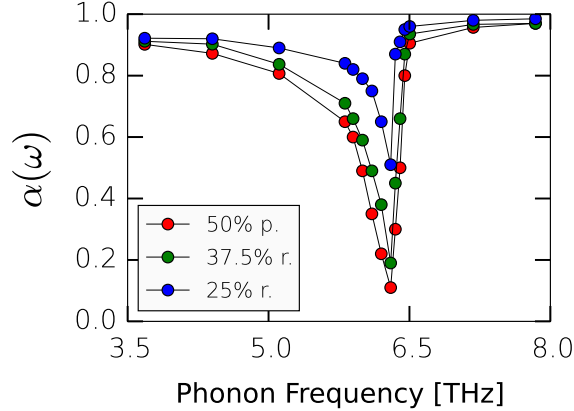
Figure 3.6: Transmission coefficient \alpha(\omega) for longitudinal phonons through the planar defect in a Si crystal, which contains randomly ( r ) distributed embedded Ge atoms with f_d = 37.5\% and 25\% , compared with \alpha(\omega) through the planar defect, which contains periodically ( p ) distributed embedded Ge atoms with f_d = 50\% . The computed \alpha(\omega) was averaged over different random distributions
