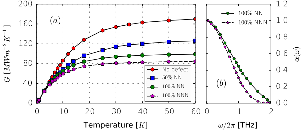
Figure 3.4: (a) Temperature dependence of interfacial thermal conductance across a crystal plane, 50%-filled with periodic array of heavy isotope defects (rectangles), and across a uniform defect crystal plane with (pentagons) and without (circles) the second phonon path induced by the non-nearest-neighbor (NNN) bonds in addition to the nearest-neighbor (NN) bonds, in comparison with that across an atomic crystal plane without defects (hexagons). (b) Transmission coefficient \alpha(\omega) for a uniform defect crystal plane with (pentagons) and without (circles) the second phonon path induced by the NNN bonds
