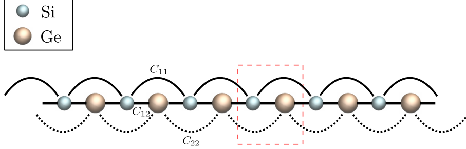
Figure 5.3: Diatomic 1D model which incorporates the second nearest-neighbour (NN) bonds C_{11} and C_{22} bypassing the nearest-neighbour bonds C_{12} between the host atom with mass m_1 and the guest atom with mass m_2 . The host atoms are coupled through the NN bonds C_{12} . The region inside the red dashed rectangle refers to the primitive cell.
