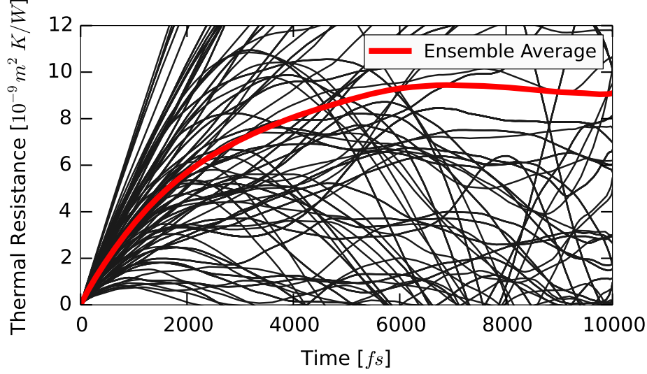
Figure 2.5: Thermal resistance proportional to the time integrals of the normalized autocorrelation functions of the temperature difference from Eq. (2.35). The black curves are from different trajectories and the red curve is the ensemble average.
