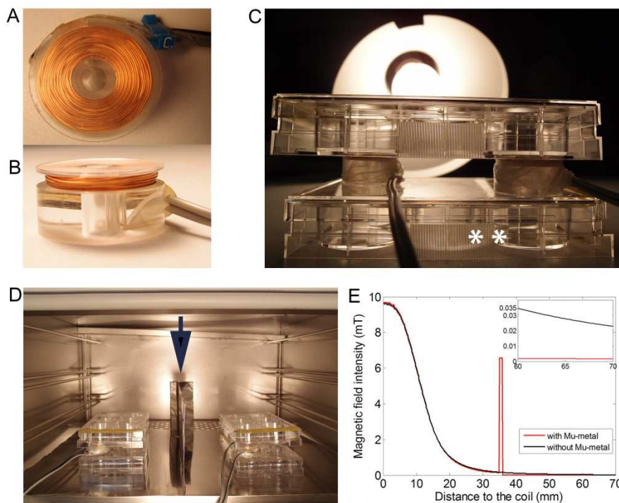
Figure 3.8 Coil set-up and magnetic shielding. A, B) View of a single coil from the top (A) and the side (B). C) View of the coils located on supporting cell plates underneath the tissue (**). Coils were wrapped in Parafilm M (Bemis, USA) to ensure stability and sterility. D) View of the coil set-up within the incubator. A sheet of (min 1mm thickness) of Mu-metal is also placed between adjacent cultures (vertical arrow). To ensure complete shielding also to the top and bottom of different incubator levels, a sheet of Mu-metal is also placed under the supporting cell plates. Mu-metal was never in direct contact with the coils as they were placed on supporting plastic plates (see C). E) Effect of the Mu-metal on the magnetic field. Black lines indicate a produced magnetic field without Mu-metal shielding at a horizontal distance from the centre of the active coil. Red line shows the magnetic field in correspondence with a Mu-metal shielding at 35 mm from the coil. Magnetic field intensity is concentrated by Mu-metal, leading to complete shielding with no detectable magnetic field at adjacent cultures (> 60 mm distance (small inset)).
