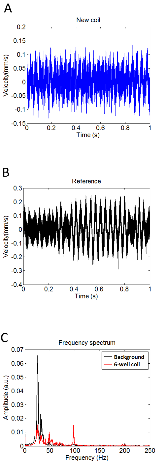
Figure D.2 Vibration measurement of the 6 well coil (A, blue) and background surface (B, black) in mm/s as measured by a single point vibrometer with OFV-534 compact sensor head for high optical sensitivity. Vibration velocity of coil is below background vibration. C) Fourier transform of the frequency spectrum confirming total below background amplitude vibrations.
