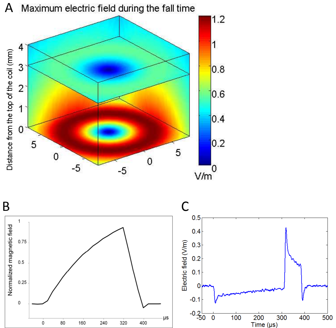
Figure C.1 Magnetic waveform and modelled electric field induced by 24 well coil (Chapter 2). A) Modelled 3D overview of the induced electric field from the top of the coil wiring (horizontal plane at 0 mm). Plane at 3 mm corresponds to average horizontal location of target cells. Colours indicate the electric field strength (V/m). B) Single magnetic pulse waveform in normalized units measured via hall effect. The stimulation device was programmed to cease current flow at 300 \mu\text{s} (pulse ON) but due to technical imprecision, pulse ceased at 320 \mu\text{s} . C) Modelled induced electric field strength during one pulse in a round conductor at a radius of 4.5 mm from the central axis and 3 mm vertical distance from top of the coils wiring. Maximum electric field strength at target cells \sim 0.4 V/m during down time of pulse waveform.
