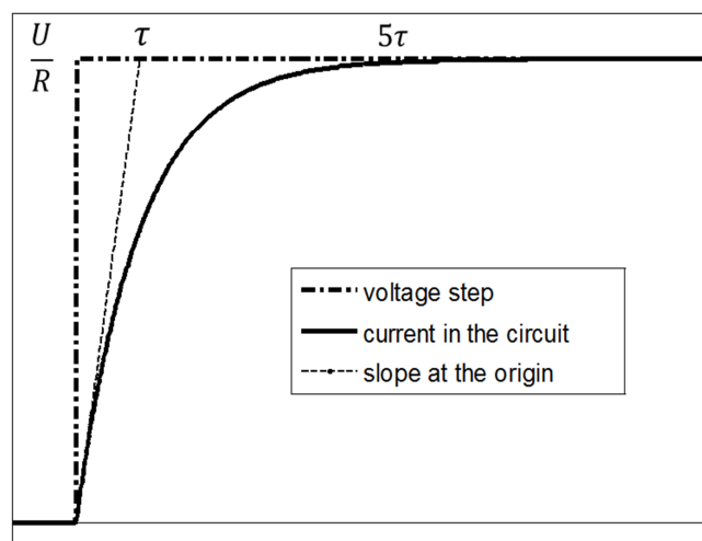
Figure 3.4 Definition of the characteristic time Tau ( \tau ). Current intensity inside the circuit in response to increasing voltage steps reaches more than 99.9% of its maximum after a time of \sim 5\tau .
