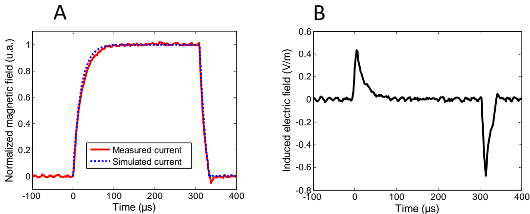
Figure 3.7 A) Single pulse waveform in normalized, arbitrary units (a.u.). Intensity inside the coil modelled in Tina (blue dotted line) and magnetic field strength measured via hall effect (red line), showing a tight correspondence between predicted and measured waveform. B) Calculated, single pulse induced electric field in a round conductor at a radius of 2 mm from the central axis and 4 mm vertically above the top of the coil's wiring.
