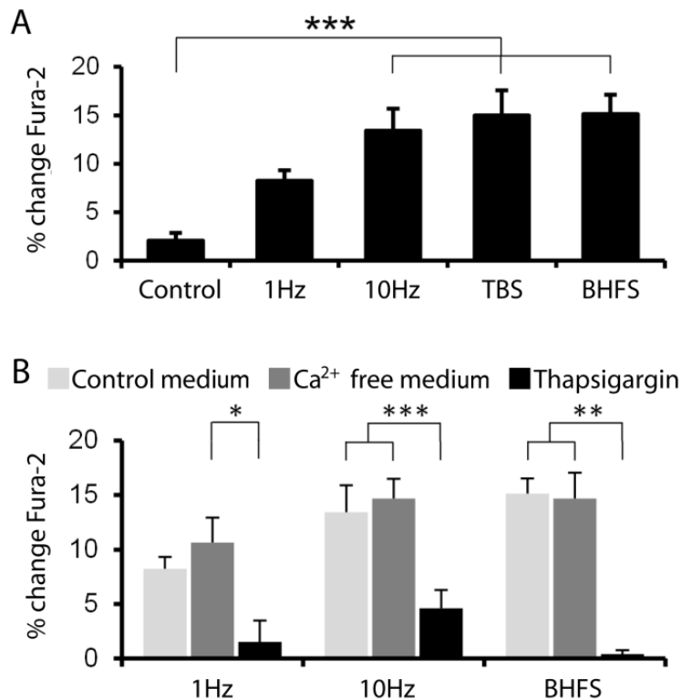
Figure 2.4 LI-rMS induces Ca 2+ release from intracellular stores. Alterations in Fura-2 340/380 nm ratiometric fluorescence (% change Fura-2) in cortical neurons after a single 10 min stimulation with 1 Hz, 10 Hz, cTBS and BHFS frequencies. A) LI-rMS at each of 10 Hz, cTBS and BHFS increased intracellular calcium compared to unstimulated controls, while 1 Hz only generated an intermediate rise ( H = 20.7 , p = 0.000 ). Pairwise comparisons Control-10 Hz: U = -27.97 , p = 0.007 ; Control-cTBS: U = -32.48 , p = 0.001 ; Control-BHFS: U = -38.03 , p = 0.000 . B) LI-rMS induced similar increase in Fura-2 ratiometric fluorescence in normal imaging and calcium-free media but not in thapsigargin supplemented ( H = 20.89 , p = 0.000 ). Pairwise comparisons Normal-Thapsigargin: U = 23.6 , p = 0.000 ; Ca 2+ free – Thapsigargin: U = 31.39 , p = 0.000 ). Error bars are standard error of the mean.
