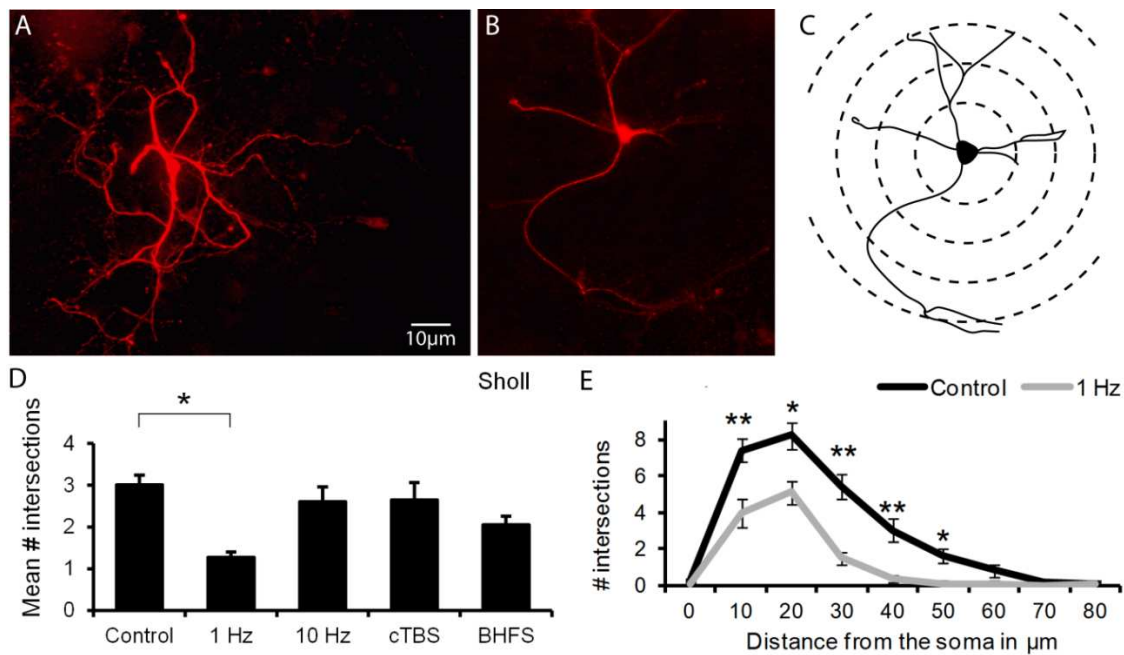
Figure 2.3 LI-rMS has stimulation pattern-specific effects on neuronal morphology. A,B) Representative neuronal morphology from control (A) and 1 Hz (B) stimulation. C) diagram illustrating Sholl analysis. D) mean number of dendrite intersections per neuron following LI-rMS (4 days, 10 min per day) at different frequencies ( H = 17.84 , p = 0.001 . Pairwise comparisons Control-1 Hz: U = 30.771 , p = 0.001 ). E) Number of intersections per concentric Sholl circle from 10-80 \mu\text{m} from the soma are decreased in 1 Hz stimulated samples compared to unstimulated controls (10 \mu\text{m} : U = 7.13 , p = 0.008 , 20 \mu\text{m} : U = 5.94 , p = 0.015 , 30 \mu\text{m} : U = 7.86 , p = 0.005 , 40 \mu\text{m} : U = 6.84 , p = 0.009 , 50 \mu\text{m} : U = 5.29 , p = 0.021 ). Error bars are standard error of the mean.
