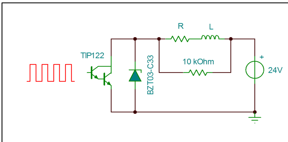
Figure 3.3 Schematic overview of the electronic circuit used to produce the desired current in the coil ( L ). The microcontroller produces a squared waveform, which triggers the darlington transistor (TIP122) on and off to permit the 24V power source to drive current through the RL circuit at the desired frequency during the desired period. The unidirectional zener diode (BZT03-C33) limits the level of current induced by the coils energy, after the opening of the transistor, to control the fall time.
