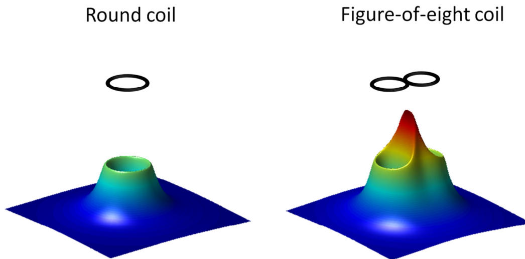
Figure 1.4 Shape of stimulation coils and their associated magnetic field. Classic round shaped coil with its associated magnetic field, showing strongest field intensities under the edges of the coil. A figure of eight coil with its associated magnetic field, with strongest field intensities under the central intersection of the two adjacent coil loops.
