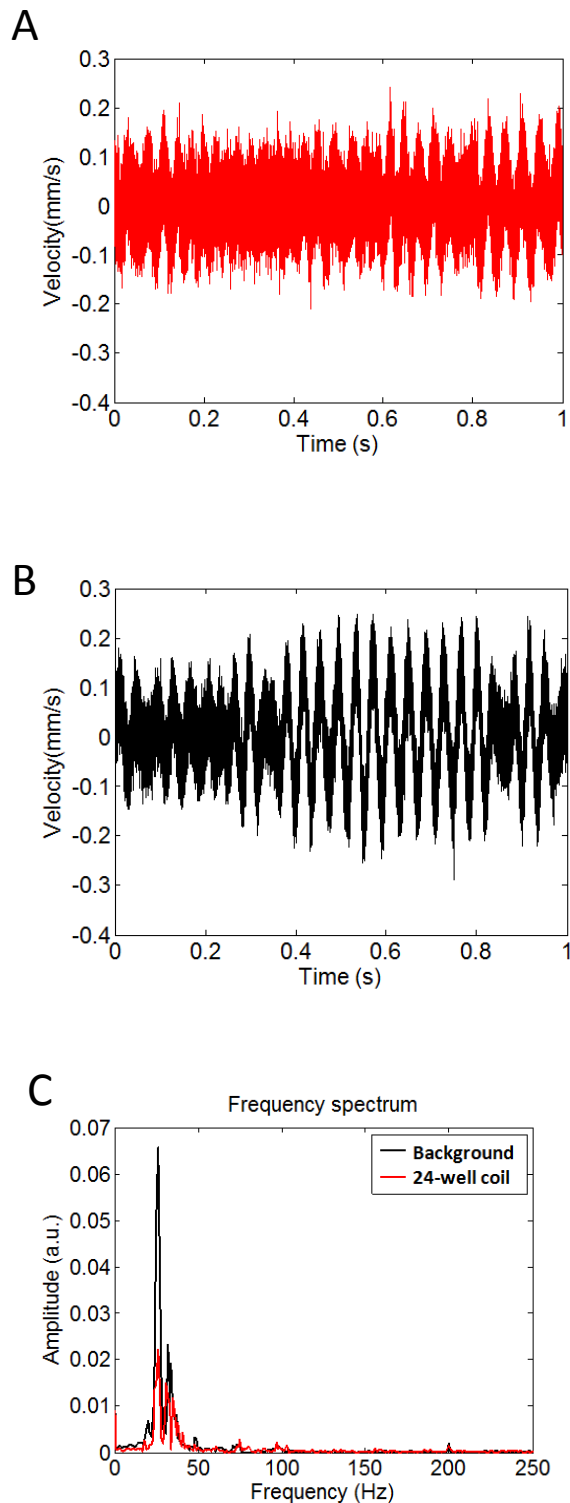
Figure D.1 Vibration measurements of the 24 well coil (A, red) and background surface (B, black) in mm/s as measured by a single point vibrometer with OFV-534 compact sensor head for high optical sensitivity. Vibration velocity of coil is below background vibration. C) Fourier transform of the frequency spectrum, confirming below background amplitude vibrations as shown in Chapter 2/article for publication).
