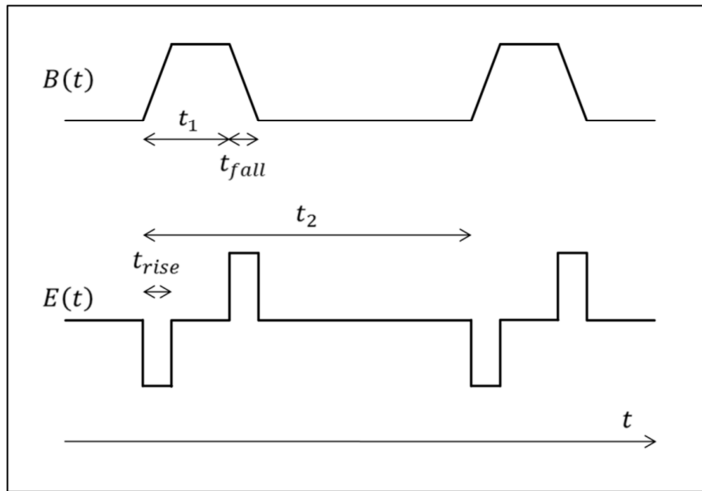
Figure 3.2 Desired magnetic field ( B(t) ) and the predicted induced electric field inside a conductor ( E(t) ). Three different temporal domains are specified for this set-up: t_{rise} = rise-time, t_{fall} = fall-time, t_1 = pulse ON and t_2 = inter-pulse interval (frequency). t_{rise}/t_{down} and t_1 are based on previous experiments and have a value of 100 \mu s and 300 \mu s respectively; t_2 is experiment dependent.
