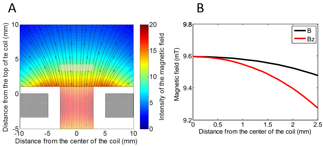
Figure 3.5 A) Modelled overview of the coil and its generated magnetic field. Grey squares at the bottom of the image show a dissected view of the coil wiring. White surround corresponds to the coils' plastic shell. Colours correspond to the magnetic field strength and black arrows to magnetic field direction B . The beige block in the centre of the image shows the location of the explant. B) Schematic overview of the different magnetic field components at 4 mm distance from the base of the coil. One can observe that the magnetic field B is almost exclusively comprised of the vertical field component B_z .
