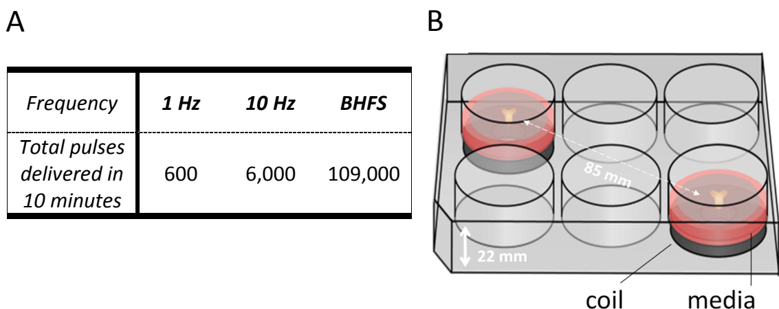
Figure 4.4 Culture set-up and pulse delivery. Number of pulses delivered per 10 min stimulation session (A) and schematic view of in vitro culture set-up for stimulation (B). B) Coils were centered below the well of a 6 well plate resulting in 4 mm distance from the centre plane of the explant located on the Millicell membrane.
