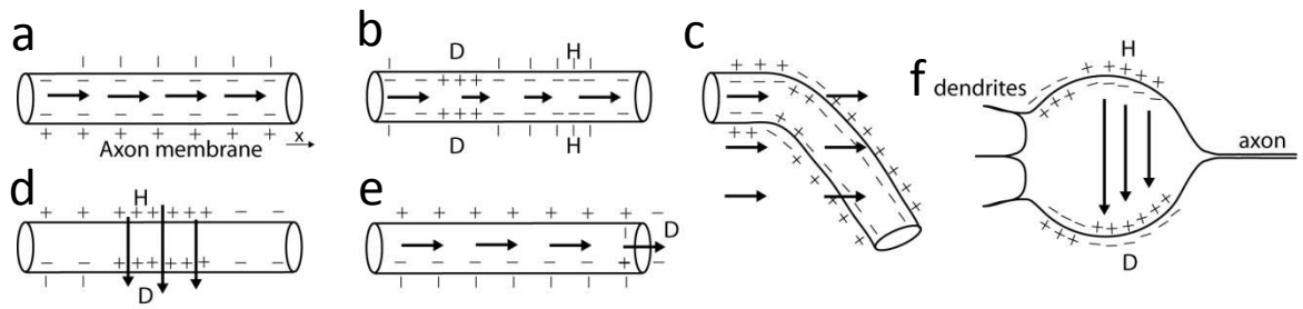
Figure 1.2 Illustration of possible activation mechanism of magnetic stimulation by gradient changes to membrane potentials. a) A uniform electric field (black arrows) flowing parallel to the axon does not result in gradients along the axon and hence no membrane potential changes occur. b) A non-uniform electric field induces partial membrane potential changes. c) An uniform electric field along a bending axon (spatial variation) causes strong membrane potential changes. d) An electric field perpendicular to an axon results in strong membrane potential changes. e) An electric field induces change at axonal terminals and f) A non-uniform field at a relative larger soma, induces partial membrane potential changes. D and H represent depolarization and hyper-polarization, respectively. Strong membrane depolarization through b, c, d, e or f are suggested to be able to generate action potentials. Figure partially adapted from Ruohonen & Ilmoniemi (1999).
