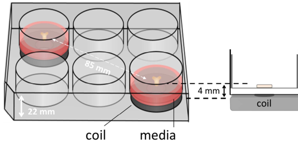
Figure 3.1 Overview of the culture set-up. The total height of the culture plate was 22 mm, resulting in a large difference between distance from the explants to the top (~18 mm) and the bottom (~4 mm). Hence, to produce a homogenous magnetic field at the position of the explants, a circular coil larger than the sample was needed. Organotypic hindbrain samples (orange) were located on a membrane ~4 mm away from the top of the coil, located underneath the culture well.
