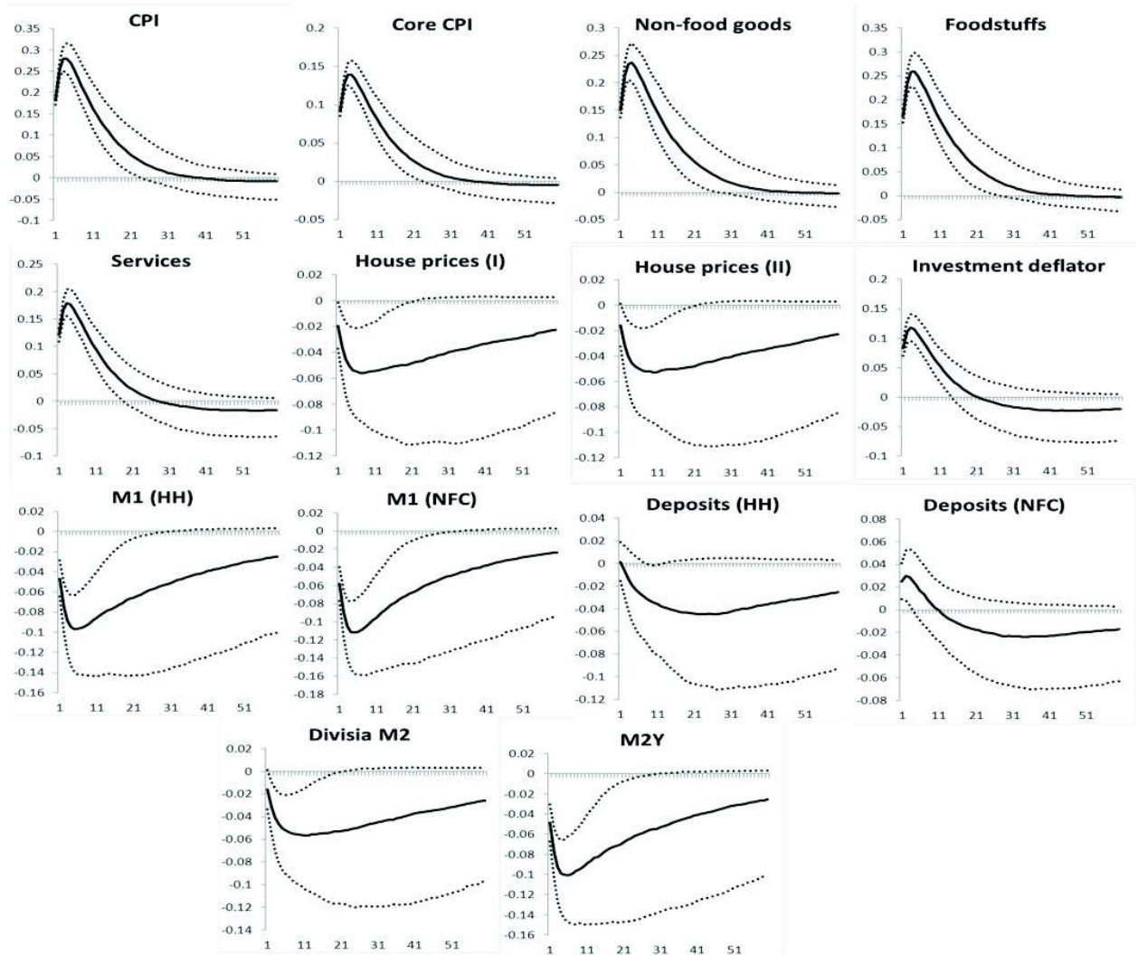
Figure 2.2A Impulse response functions for the second structural shock
